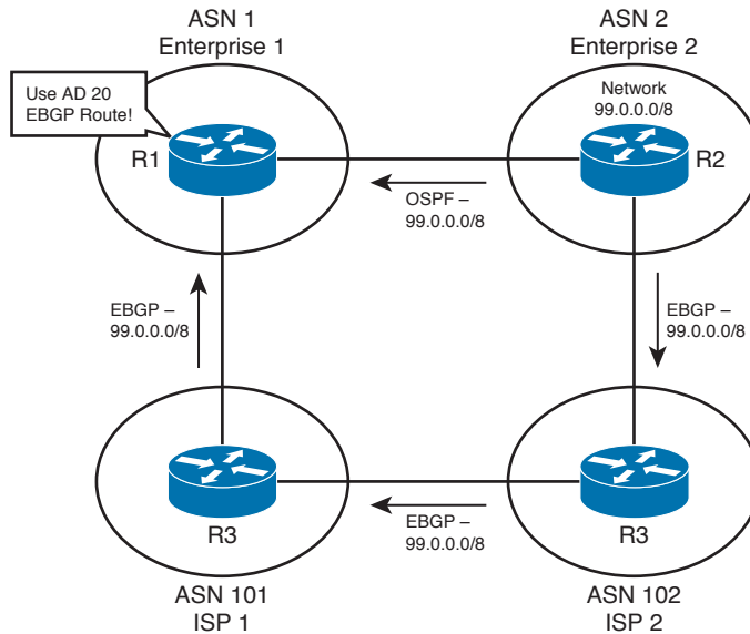
Figure 1-6 Need for BGP Backdoor Routes
