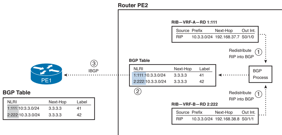
Figure 11-15 Making Prefixes Unique Using an RD
