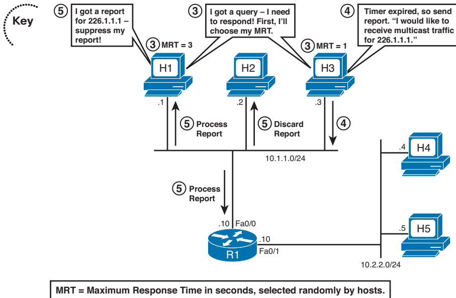
Figure 7-9 IGMPv2 Solicited Host Membership Report and Report Suppression Processes
