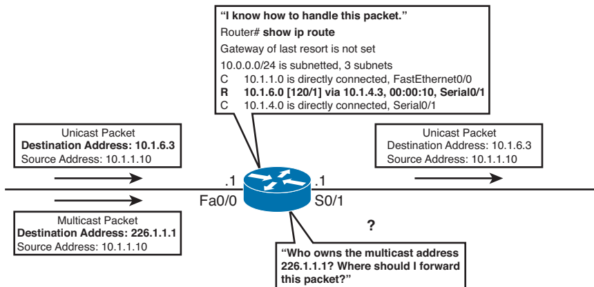
Figure 8-1 Multicast Routing Problem
