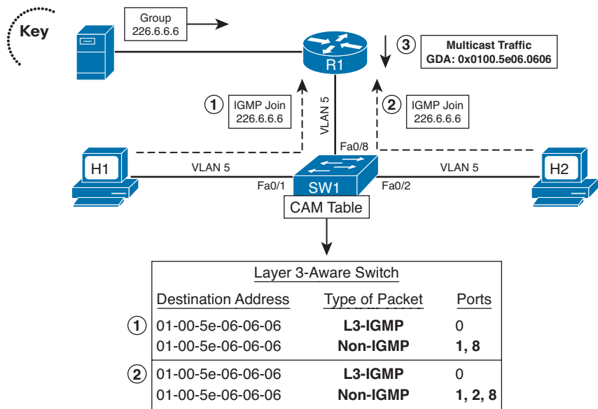
Figure 7-19 Joining a Group Using IGMP Snooping and CAM Table Entries
