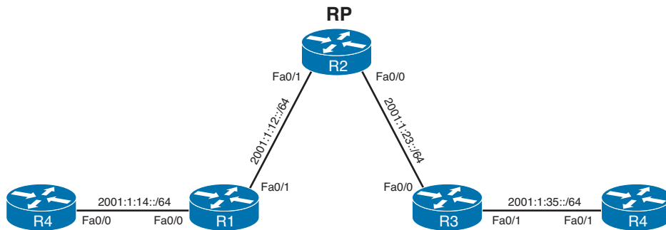
Figure 8-25 IPv6 Static RP Multicast Topology
