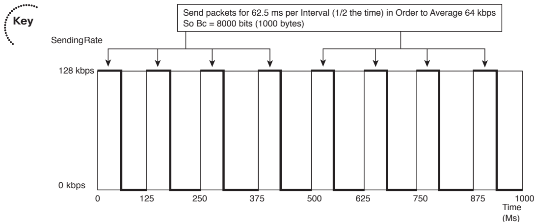
Figure 5-1 Mechanics of Traffic Shaping—128-kbps Access Rate, 64-kbps Shaped Rate
