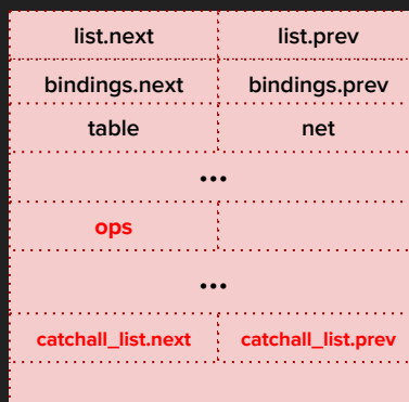
struct nft_set
