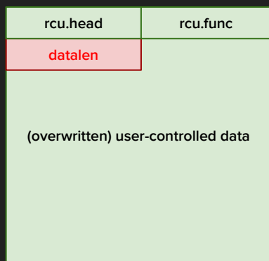
struct user_key_payload
