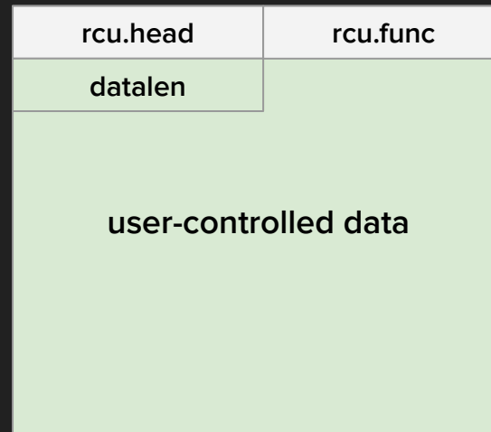
struct user_key_payload
