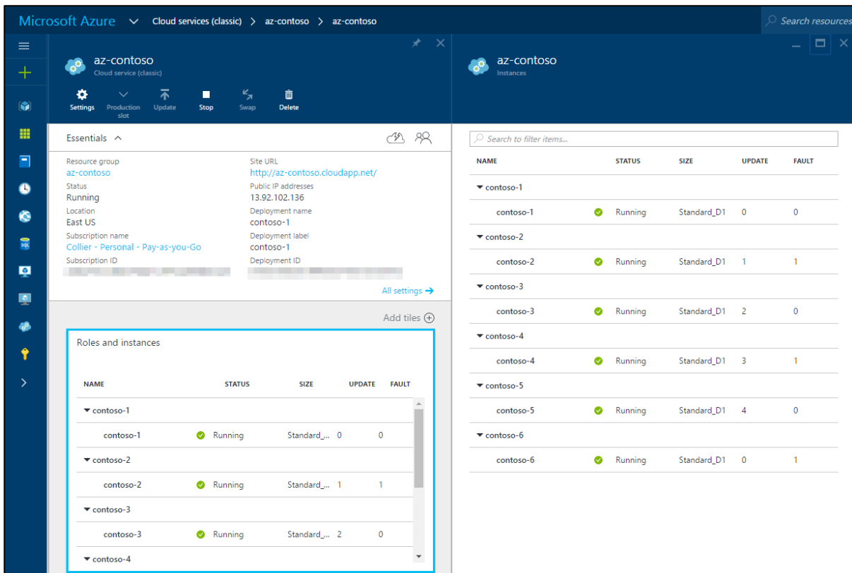
Figure 3-15 VMs, update domains, and fault domains for classic VMs.
