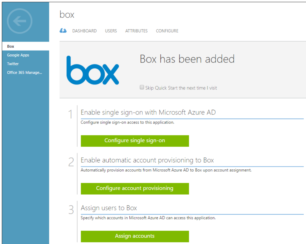
Figure 7-32 Configuration for gallery application.
