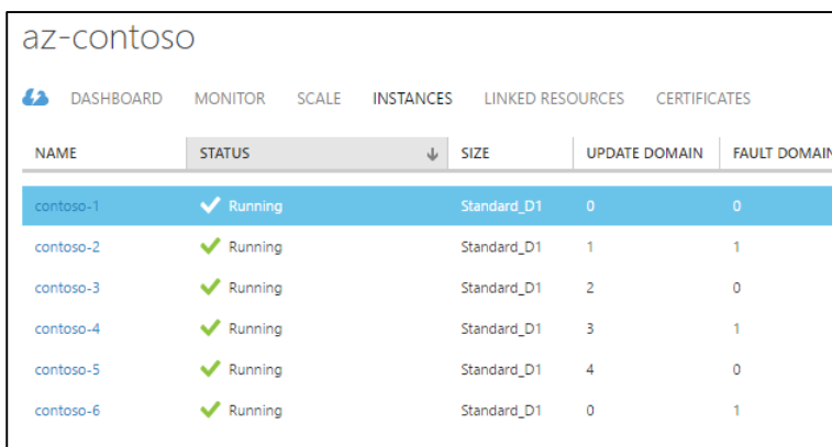
Figure 3-16 VMs, update domains, and fault domains for classic VMs in the Azure classic portal.
