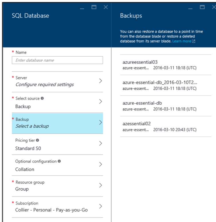
Figure 6-11 Select the desired backup as the source for a new SQL Database.
