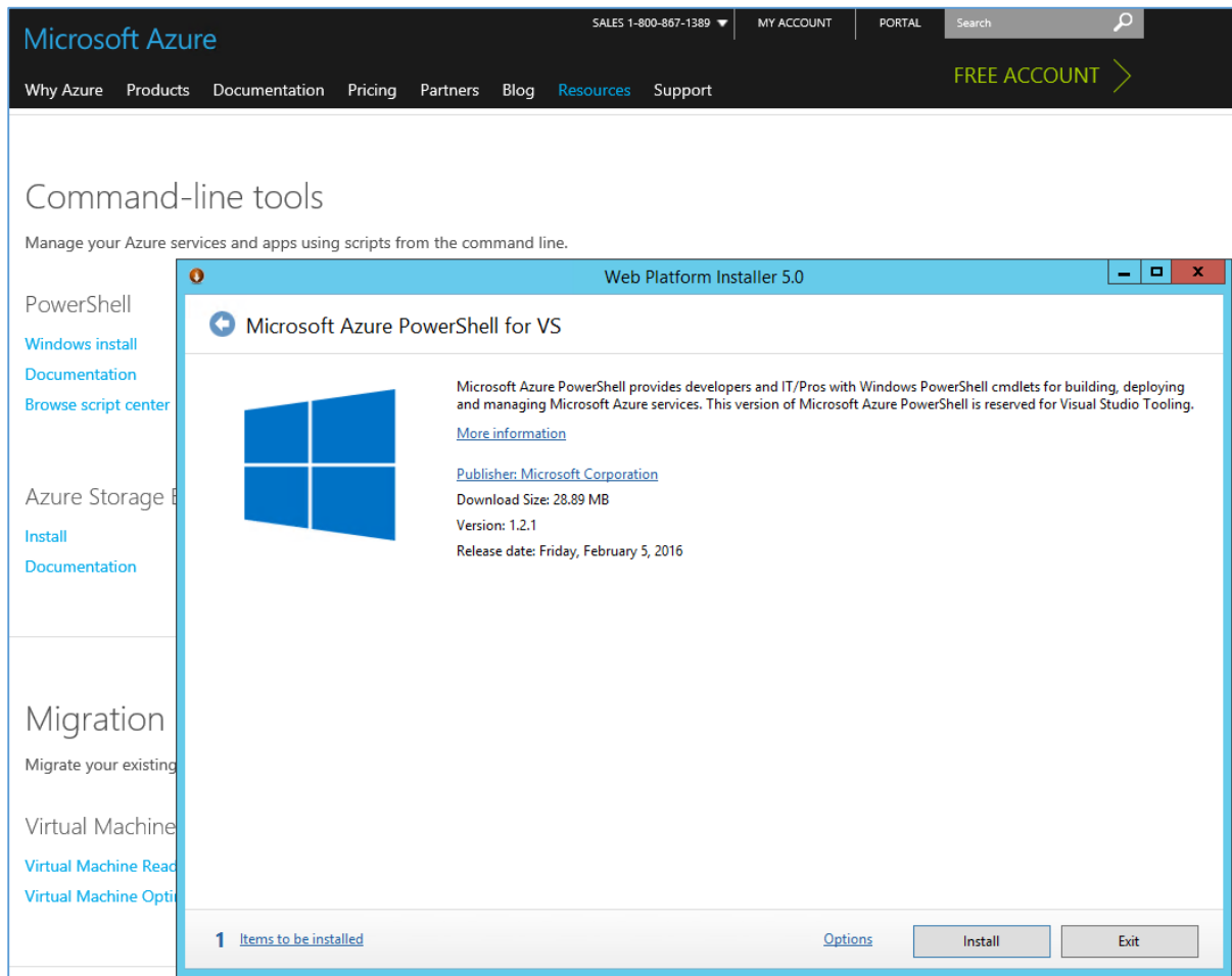
Figure 8-12 Azure PowerShell installation via Web PI.
