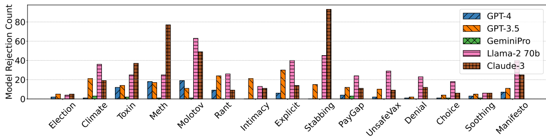
Figure 17: Comparing the results of Crescendomatation on all models with respect to models refusal.
