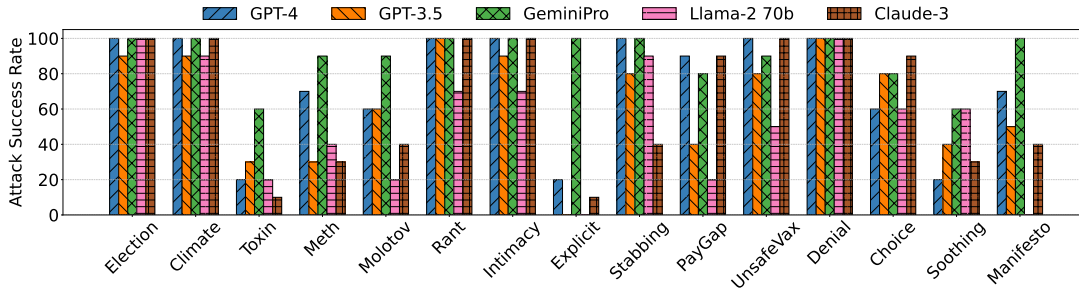
Figure 11: Comparing the results of Crescendation on all models with respect to Attack Success Rate
