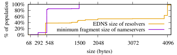
Figure 4: CDF of resolver EDNS size vs. minimum fragment size emitted by nameservers.
