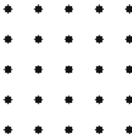
Figure 10-1. Lattice in Euclidean plane 1
