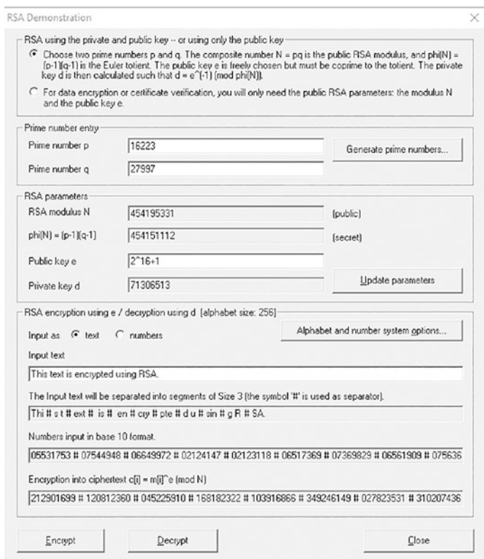
Figure 8-36. Encrypted text using RSA
