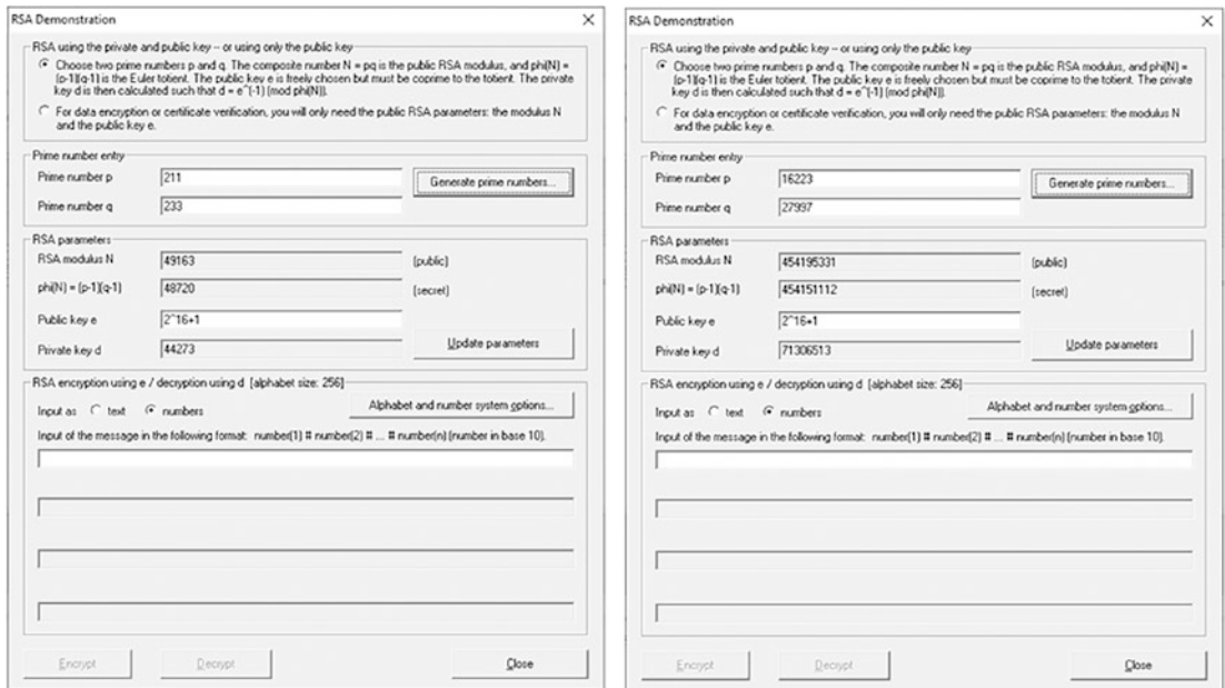
Figure 8-34. (a) RSA Demonstrator window (b) RSA Demonstrator window after generating prime numbers
