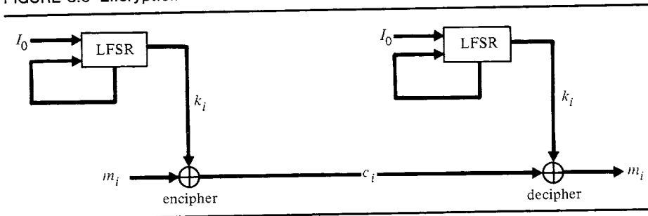
FIGURE 3.6 Encryption with LFSR.
