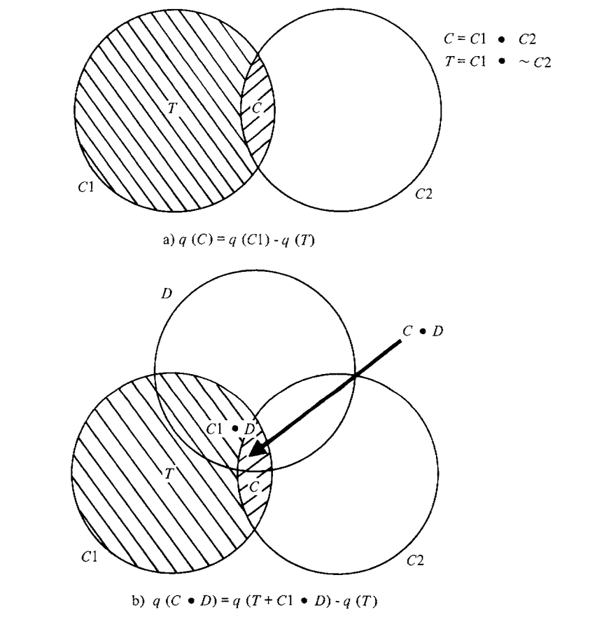
FIGURE 6.4 Individual tracker compromise.
