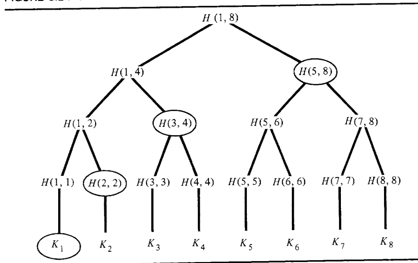
FIGURE 3.24 Tree authentication.
