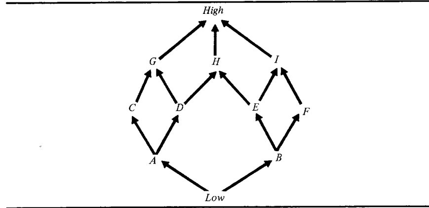
FIGURE 5.1 Lattice.
