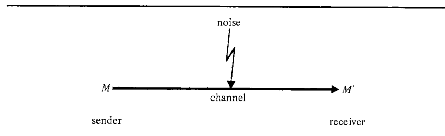
FIGURE 1.13 Noisy channel.
