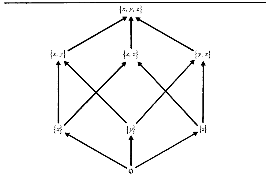
FIGURE 5.2 Subset lattice.
