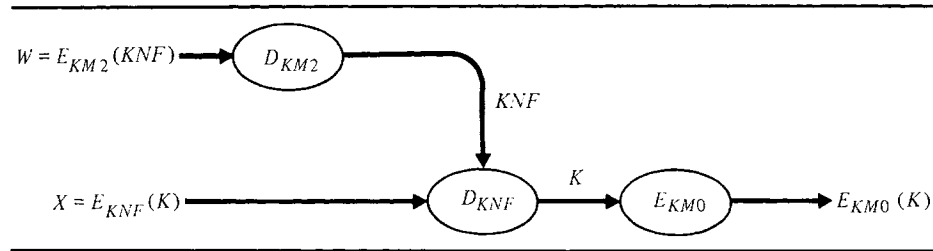
FIGURE 3.23 Reeincipher to master key ( rtmk ).
