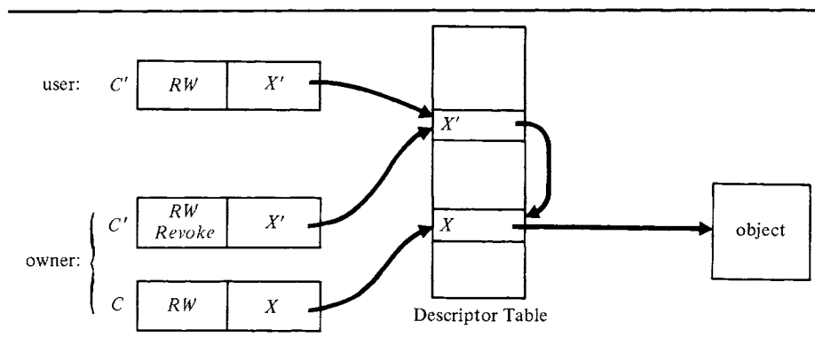
FIGURE 4.25 Revocation of rights with indirection.
