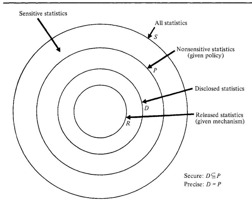
FIGURE 6.2 Security and precision.
