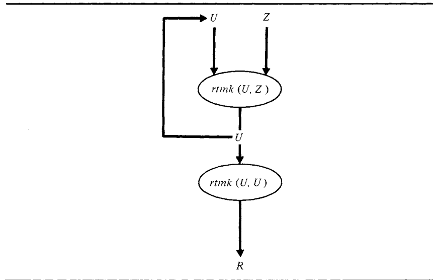
FIGURE 3.25 Key generation.
