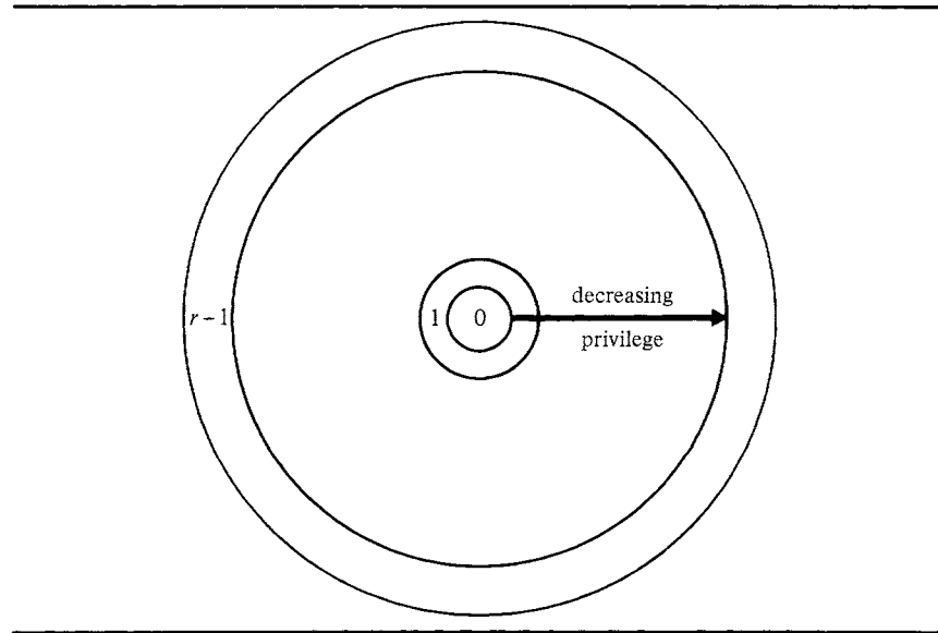
FIGURE 4.10 MULTICS rings.
