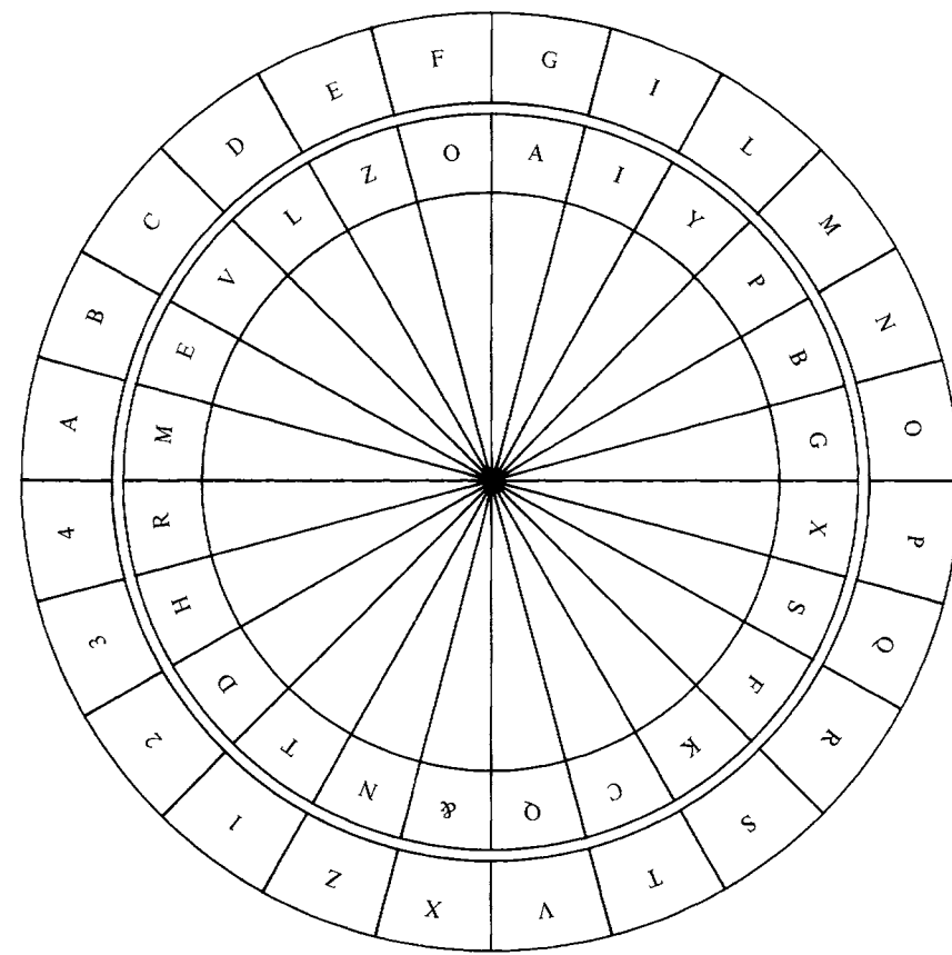
FIGURE 2.7 Cipher disk.
