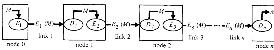
FIGURE 3.13 Link encryption.
