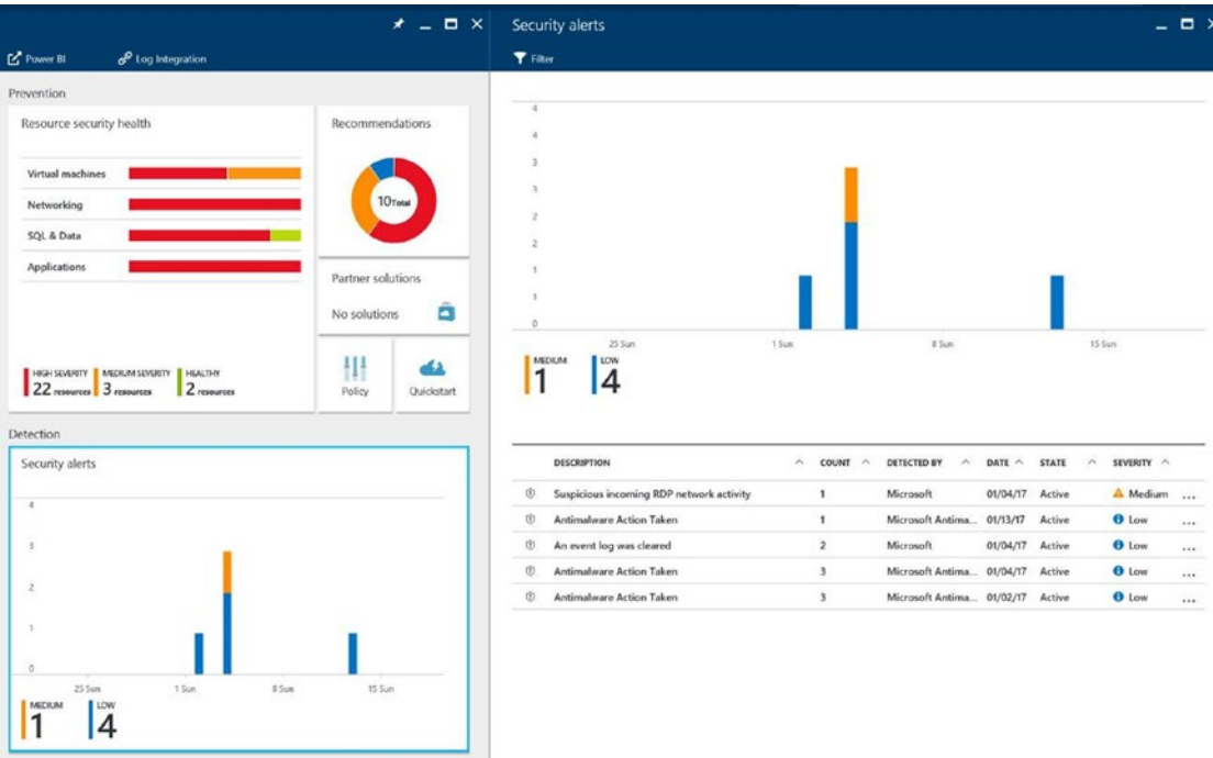
Figure 6-2. Detection and security alerts identified on the VM infrastructure
