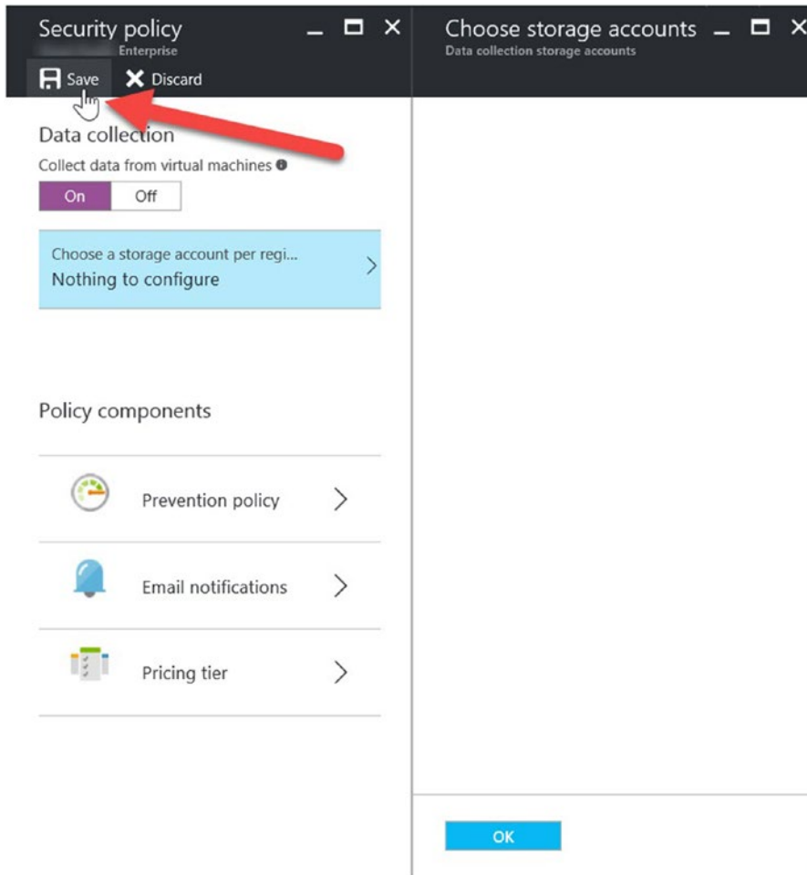
Figure 4-7. View of the data collection options to enable and save the options from the Azure blade
