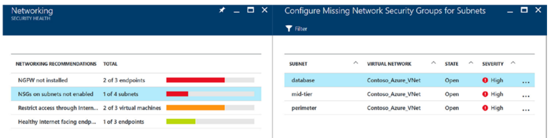
Figure 5-18. View of the NSG subnets that are not enabled
