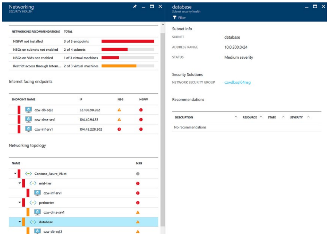
Figure 5-21. Networking security health blade after selecting the database vnet
