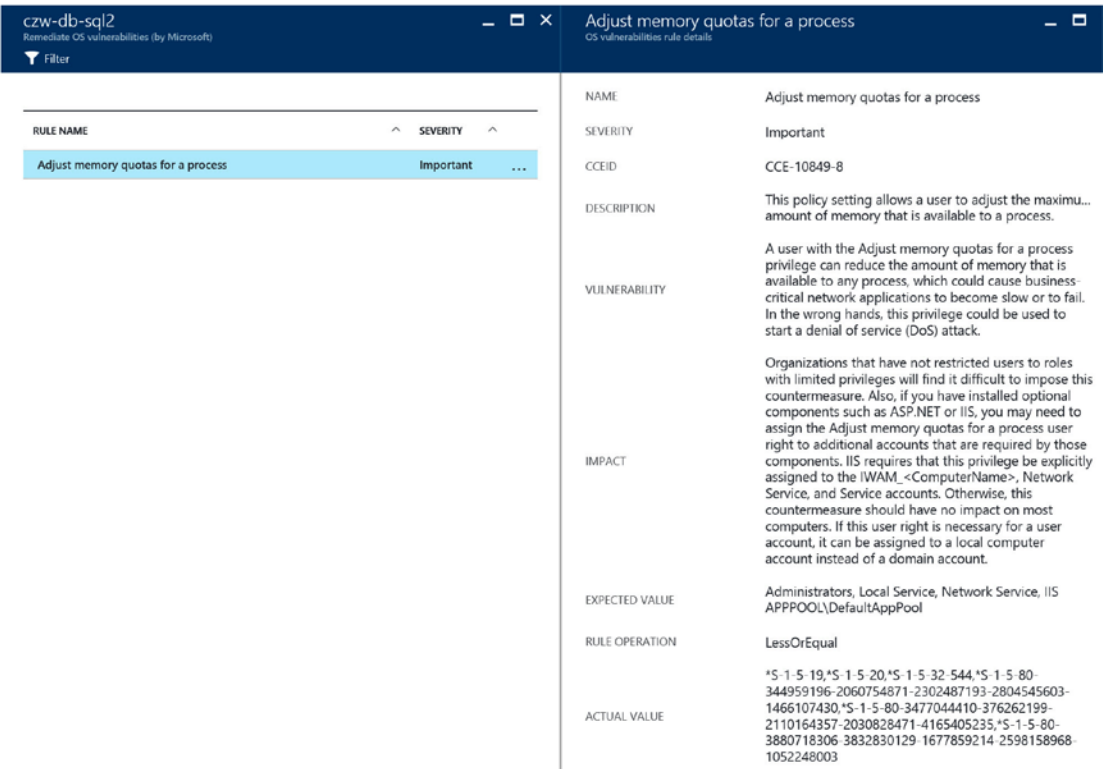
Figure 5-12. Detailed view of the automatic adjustment of the memory quota for a process action
