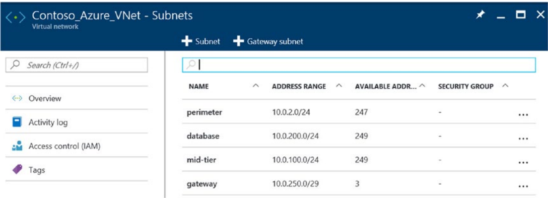
Figure 5-16. View of the Contoso Azure vnet IP subnets
