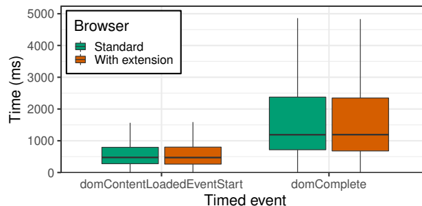
Figure 10: Impact of the countermeasure on the loading times of webpages.
