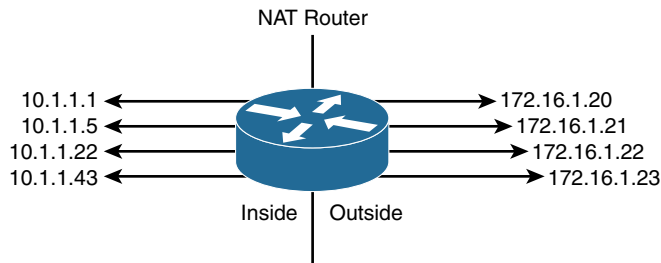
Figure 7-4 Static NAT
