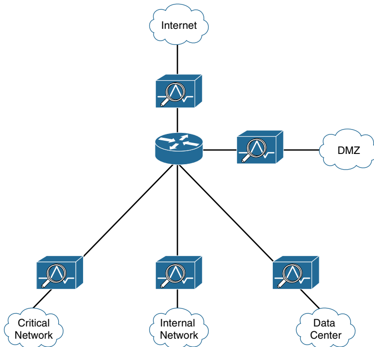
Figure 6-12 Typical NGIPS Deployment Locations
