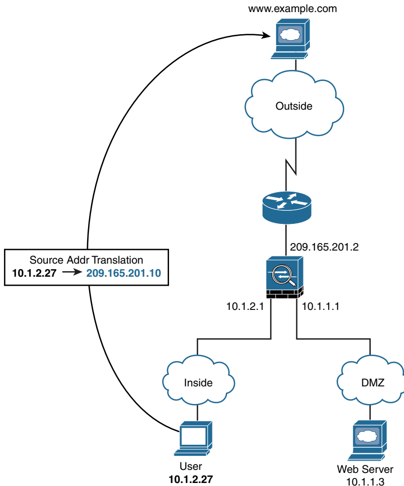
Figure 4-2 Routed Mode ASA
