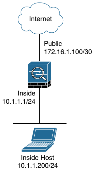
Figure 5-1 NGFW in Routed Mode
