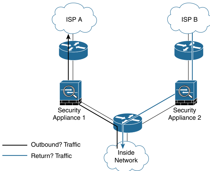
Figure 4-17 ASA Asymmetric Flow
