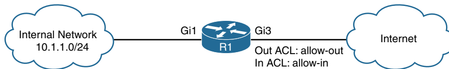
Figure 2-4 Reflexive ACL
