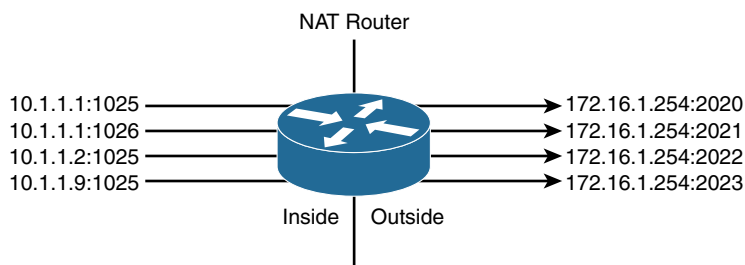
Figure 7-2 NAT Overload
