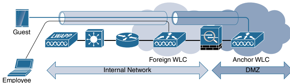
Figure 3-7 Guest Anchor Controller
