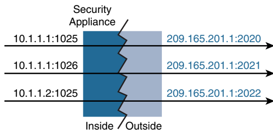
Figure 4-10 Dynamic PAT (NAT Overload)
