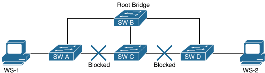
Figure 2-2 Network During Normal STP Operations
