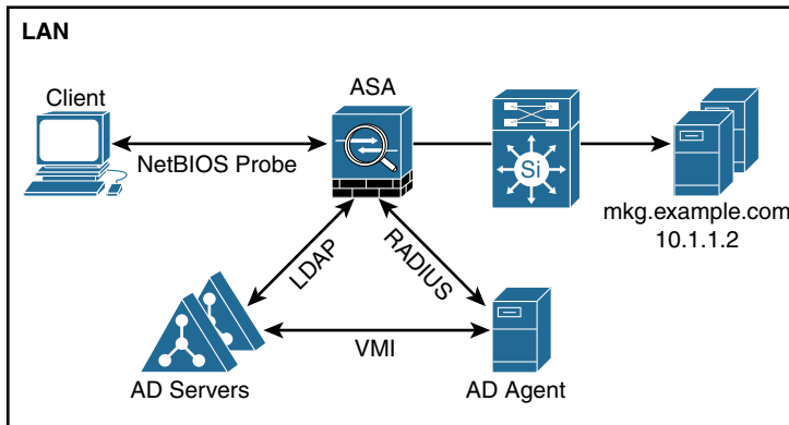
Figure 4-16 ASA-to-AD Communication
