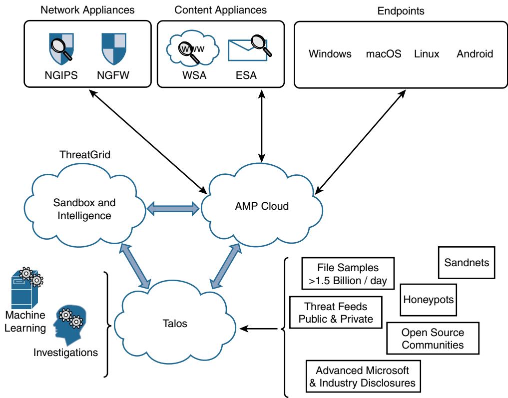
Figure 10-1 AMP Architecture
