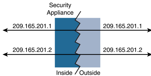
Figure 4-14 Identity NAT
