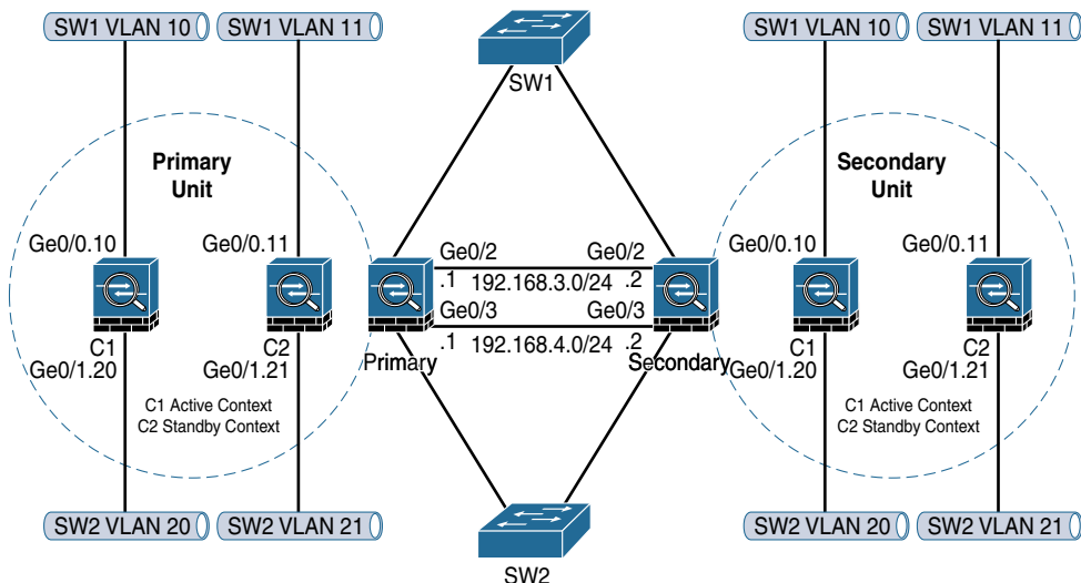
Figure 4-4 ASA Active/Active Failover
