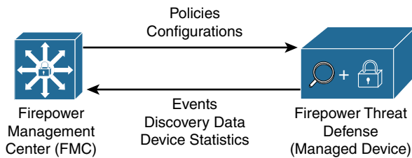
Figure 5-3 FMC Communication with a Managed Device
