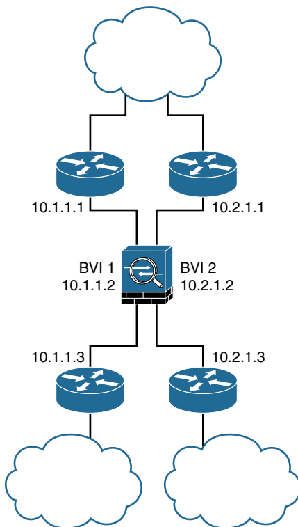
Figure 4-3 Transparent Mode ASA
