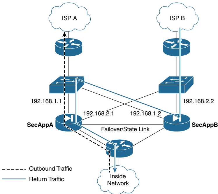
Figure 4-5 Asymmetric Flow on an Active/Active ASA Pair
