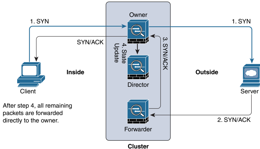
Figure 4-7 ASA Cluster Control Plane Operation with Asymmetric Traffic
