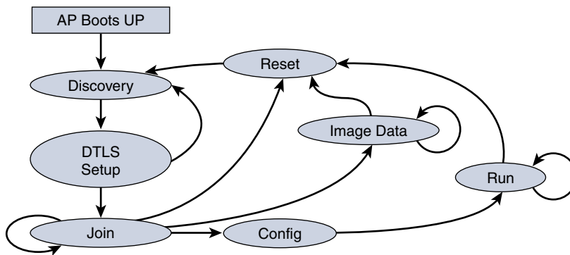
Figure 3-3 CAPWAP State Machine
