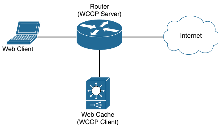
Figure 7-9 WCCP
