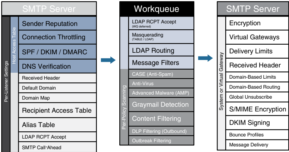
Figure 8-43 ESA Mail Flow
