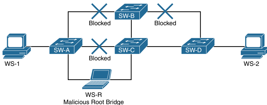
Figure 2-3 Network After a MITM Attack with STP
