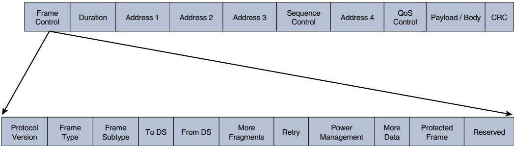
Figure 3-1 802.11 Frame Format
