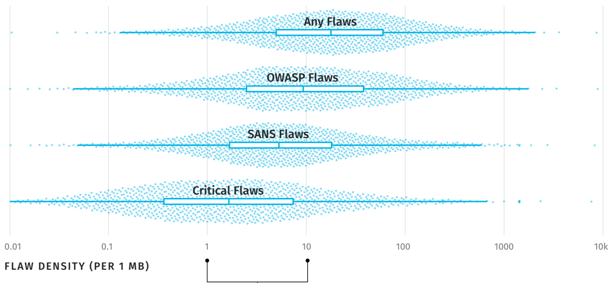
Figure 2: Application flaw density for various measures of flaw severity
