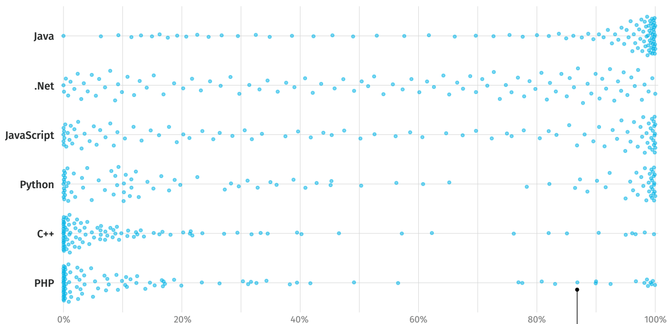
Figure 6: Percentage of application size that is third-party code
