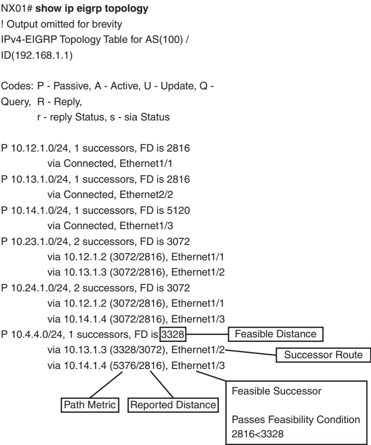
Figure 7-2 EIGRP Topology Table
