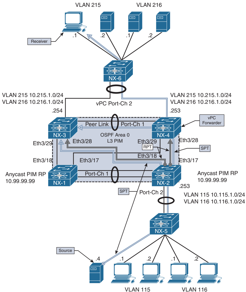
Figure 13-21 uPC-Connected Receiver Topology
