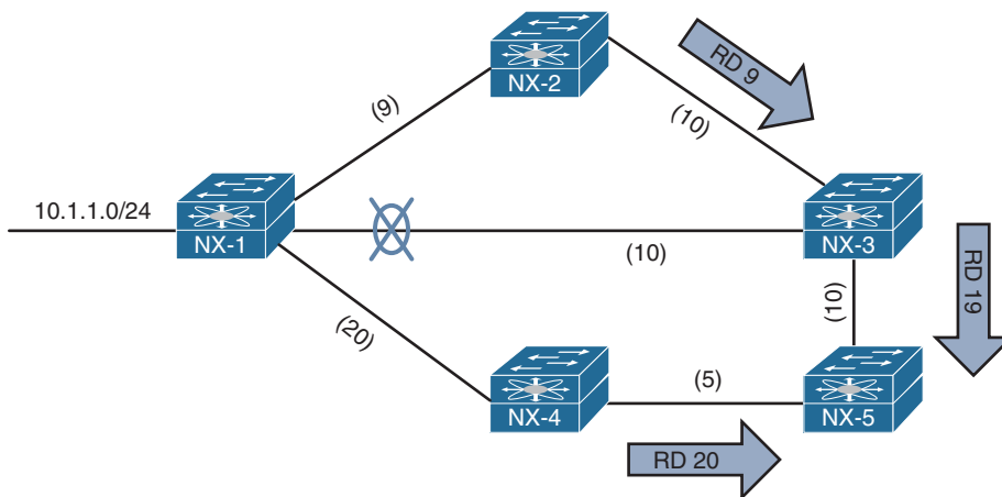
Figure 7-12 EIGRP Topology with Link Failure
