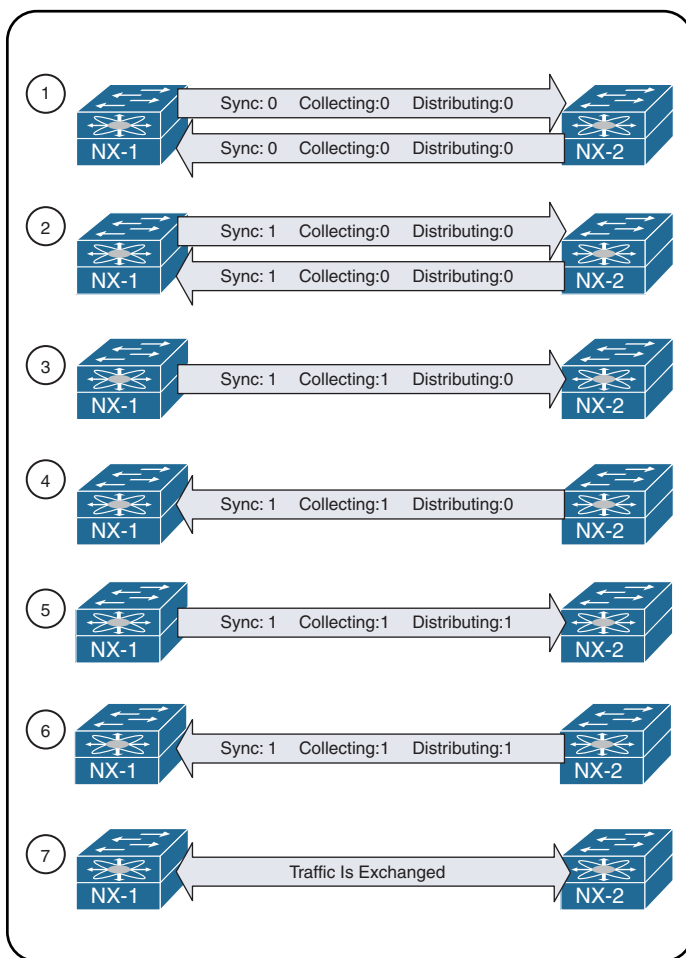
Figure 5-3 LACP Negotiation
