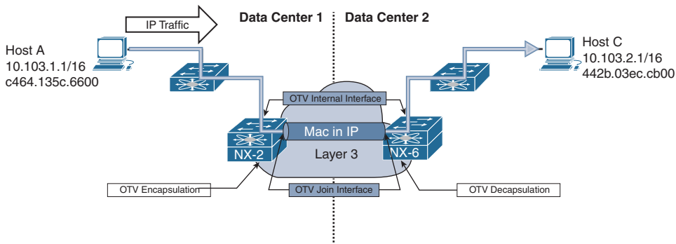
Figure 14-10 Unicast Host-to-Host Traffic Across OTV
