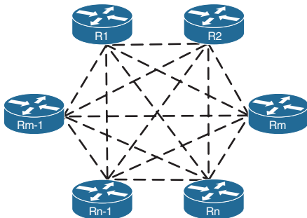
Figure 11-7 IBGP Full Mesh
