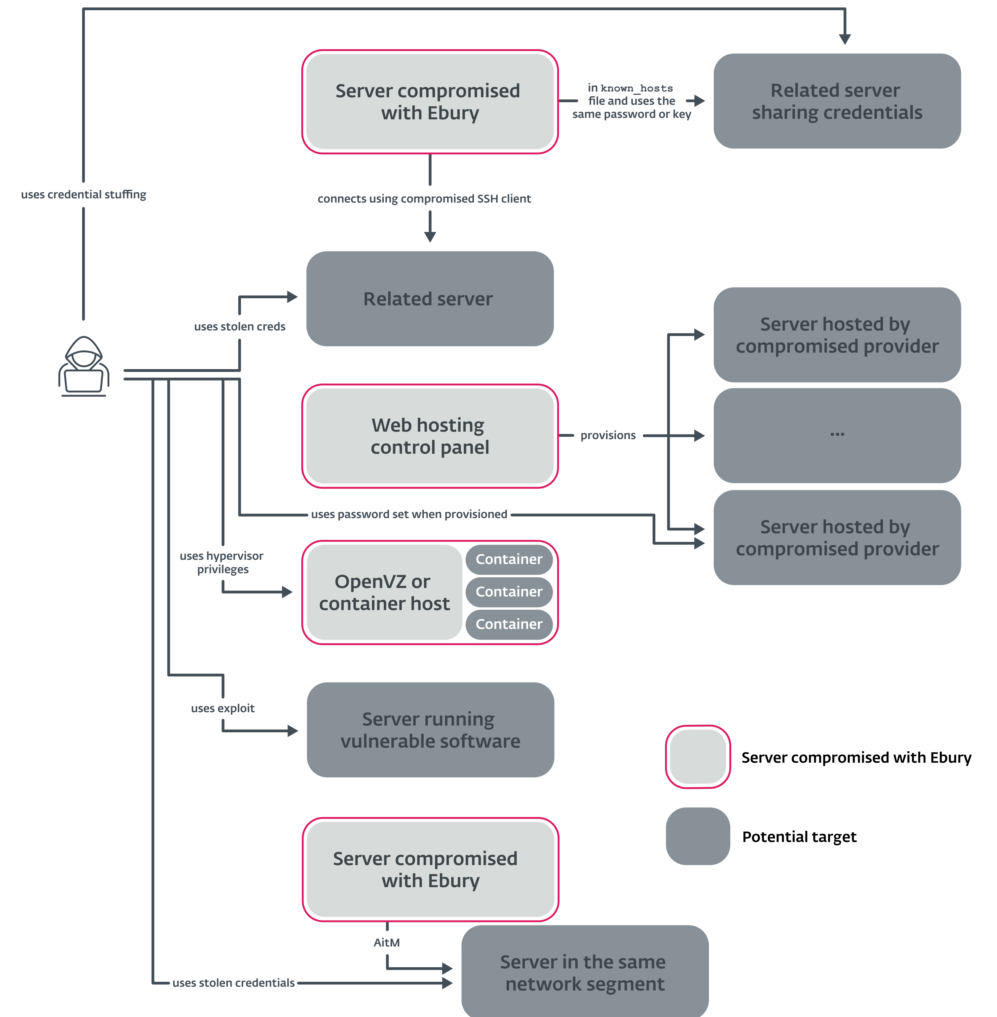
Figure 1. Different methods used by the Ebury gang to compromise new servers
