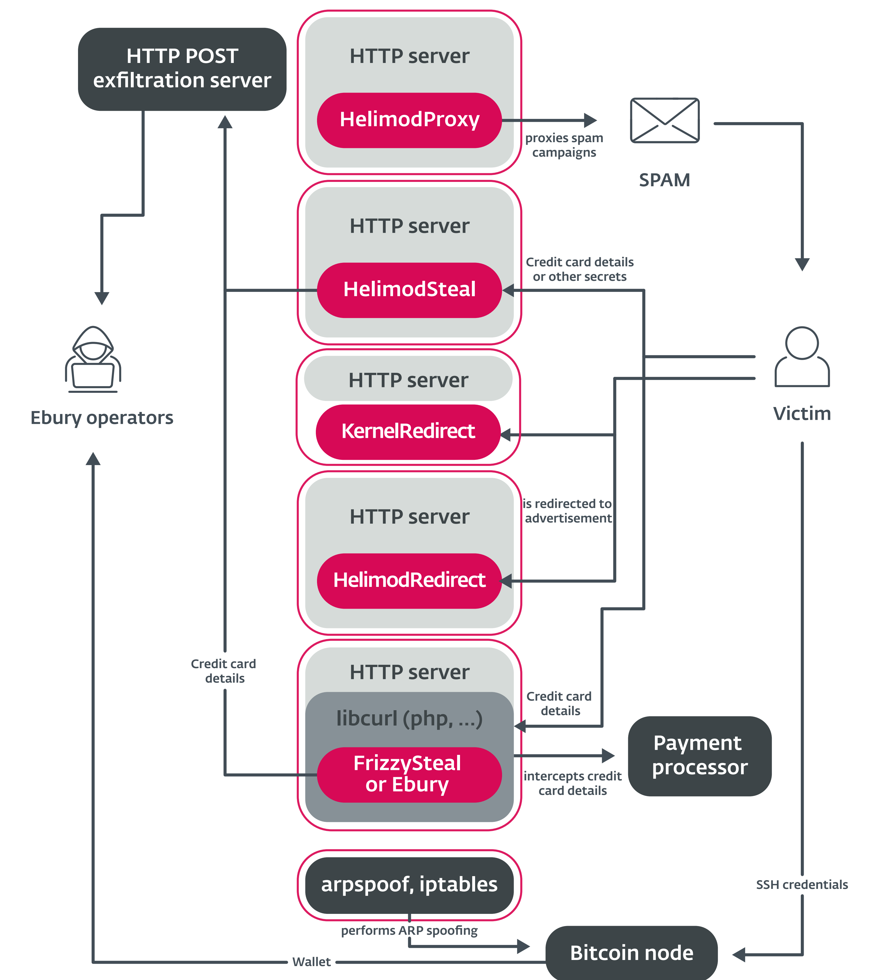
Figure 21. Multiple malware families deployed on Ebury-infested servers and the impact for potential victims
