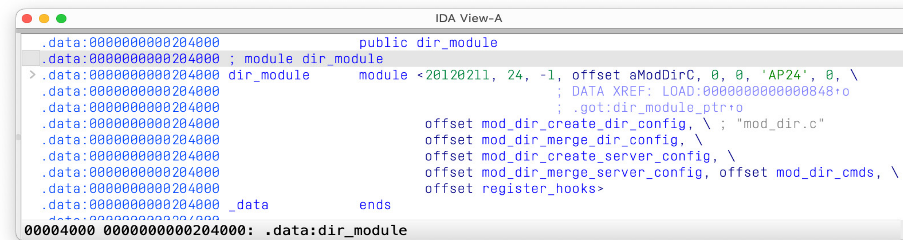
Figure 22. Module information exported by mod_dir.so as seen in IDA Pro with the proper structure definition
