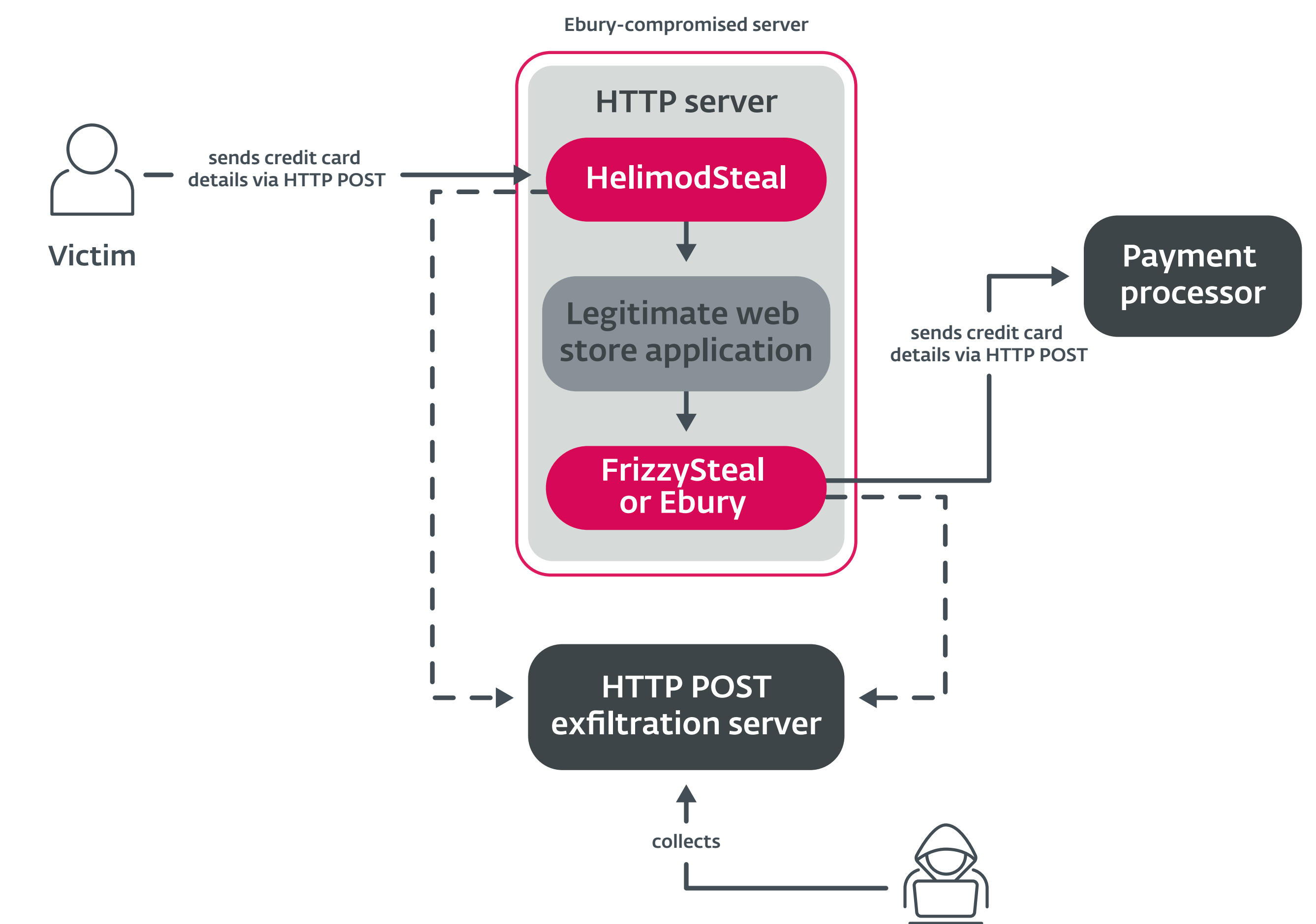
Figure 40. Flow of credit card details on transactional website compromised by Ebury
