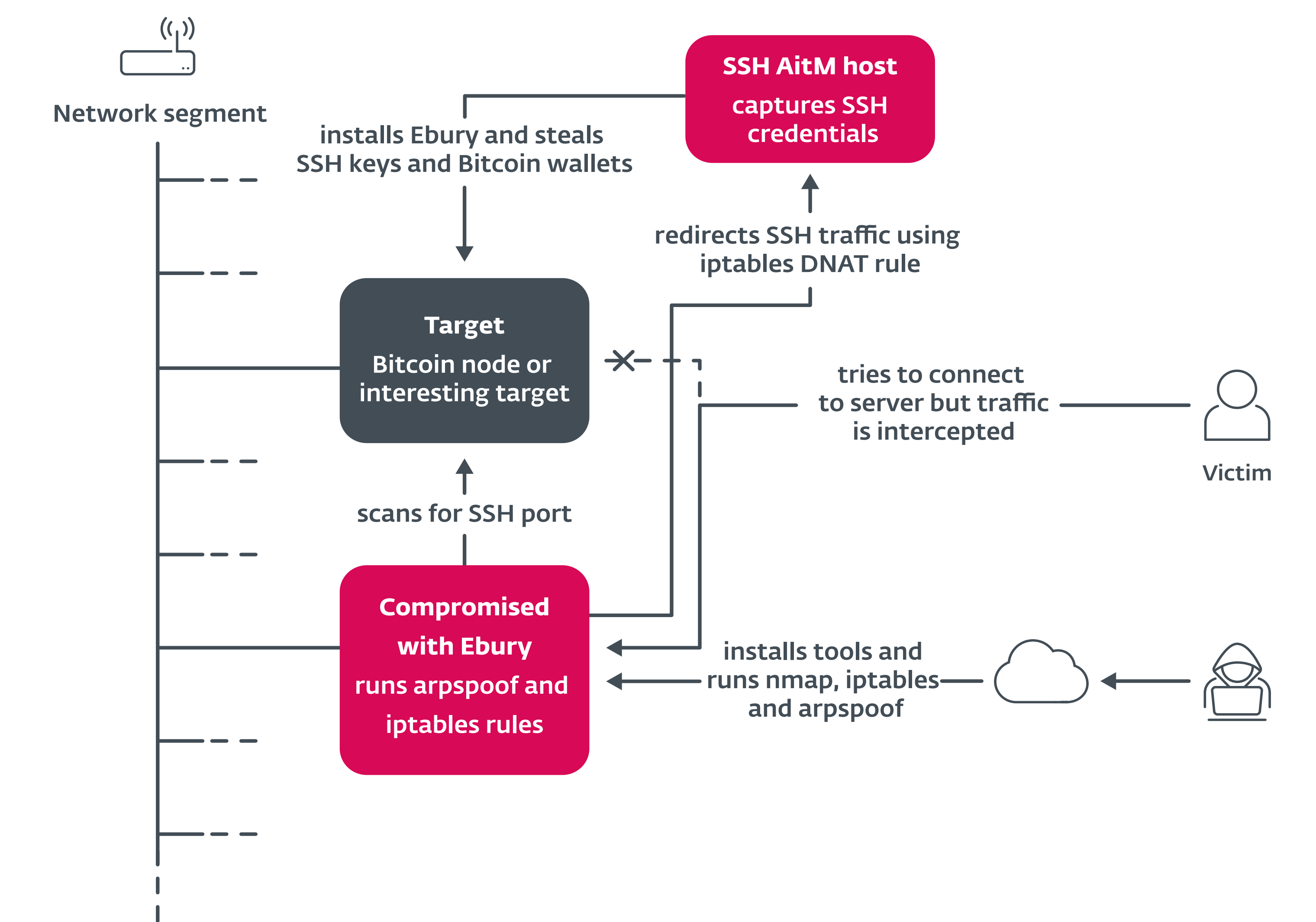
Figure 43. Overview of the AitM attacks perpetrated by the Ebury gang
