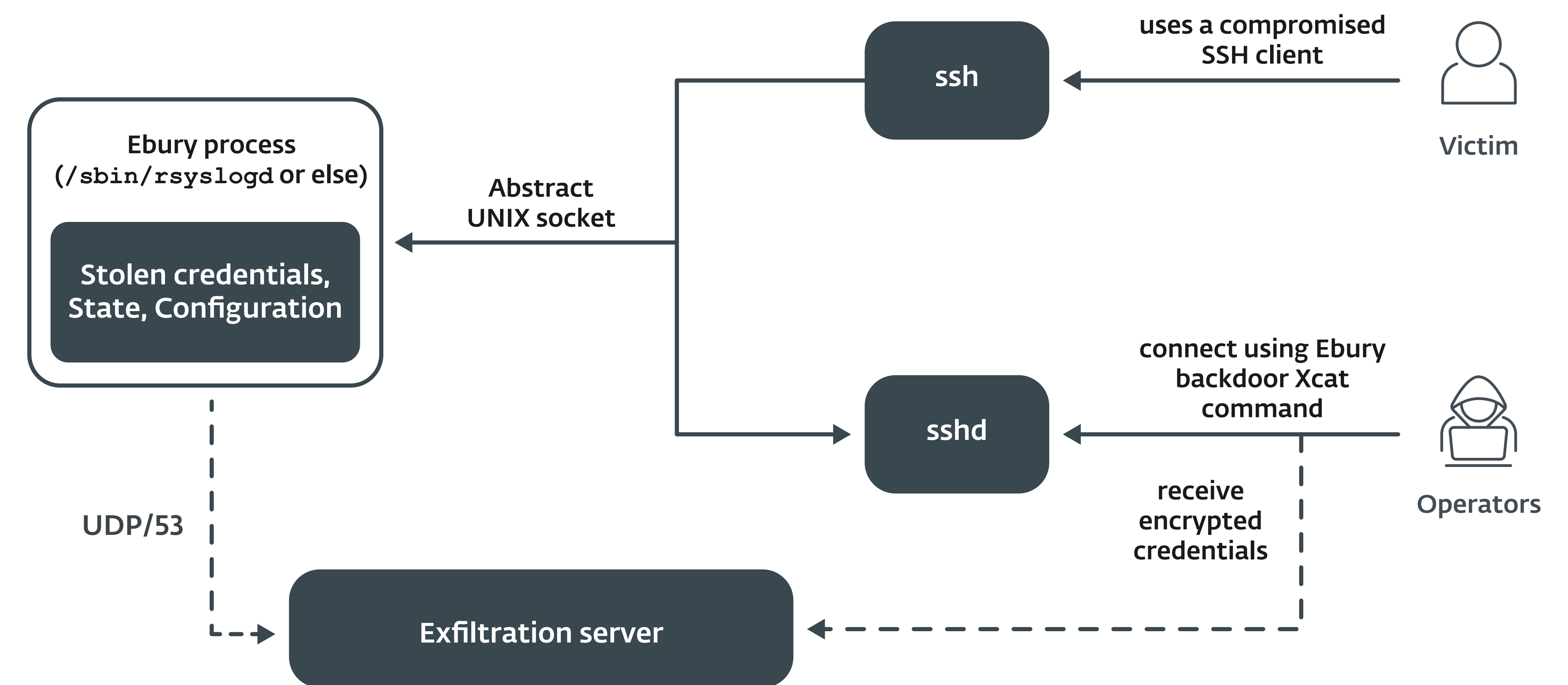
Figure 12. Flow of stolen credentials, from the victim using an Ebury-compromised SSH client to the Ebury process, and later fetched by the operators
