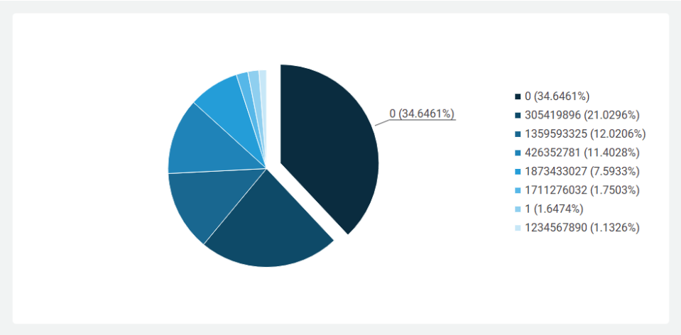
Figure 45 – Common watermarks
