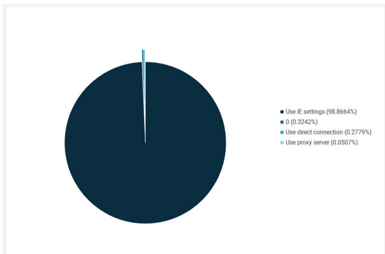
Figure 55 – Proxy behavior
