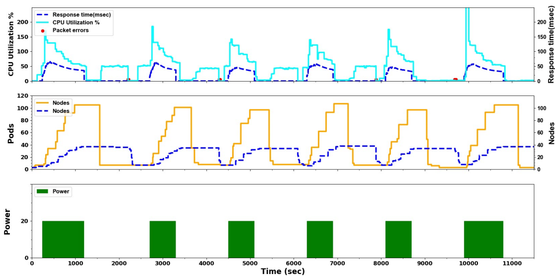
Figure 2: YoYo attack with power k=20 on Kubernetes
