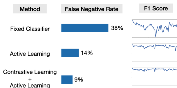
Figure 1: Android malware classification needs a way to update the classifier periodically, to address concept drift. Training a single classifier is ineffective: the average false negative rate over a 7-year period is 38%. State-of-the-art methods for active learning can reduce this to 14%. Our method, based on contrastive learning, further improves on past work, reducing the average FNR to 9% (middle column) and achieving more consistent accuracy over a 7-year period (right column).
