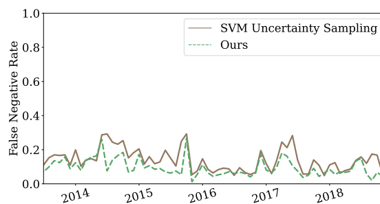
(b) FNR of our technique vs SVM with uncertainty sampling.
