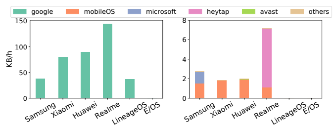
Fig. 2. The average volume of the network traffic generated on each handset by each data collector.
