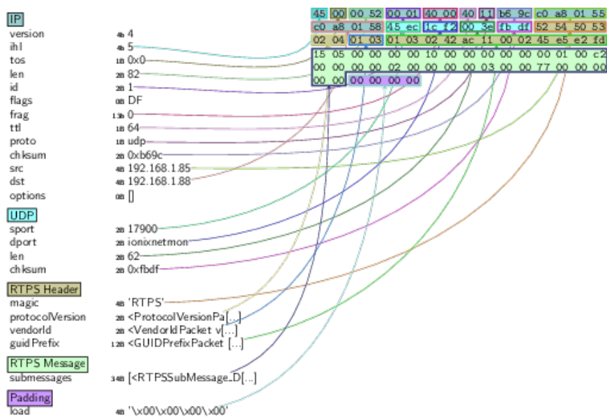
Figure 5. An example of a packet structure of an RTPS message with a DATA submessage
