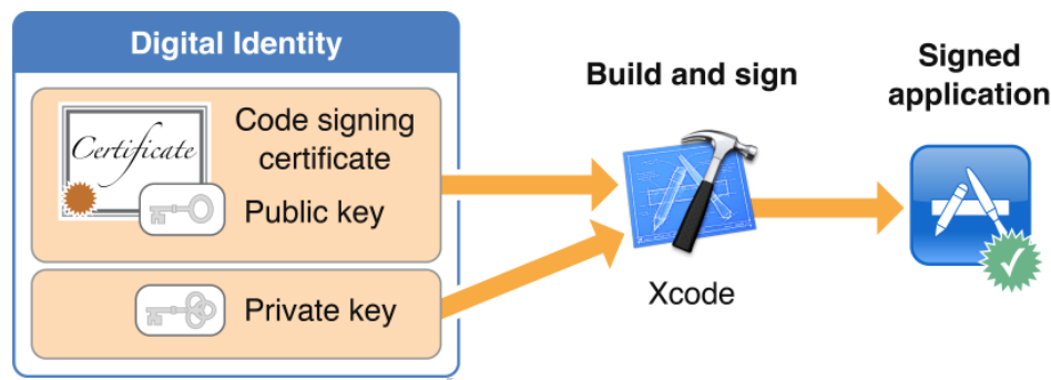
Figure 3.2: Apple Code Signing Process Documentation
