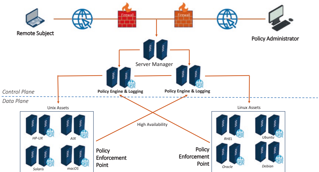
Figure 19-10. Unix and Linux zero-trust least privilege implementation including remote access support
