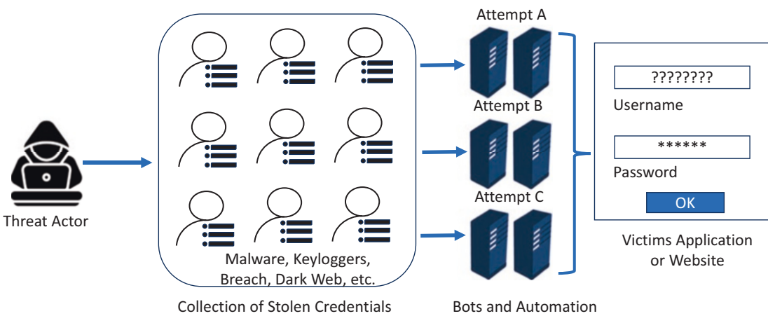
Figure 10-6. Credential stuffing using bots for automation
