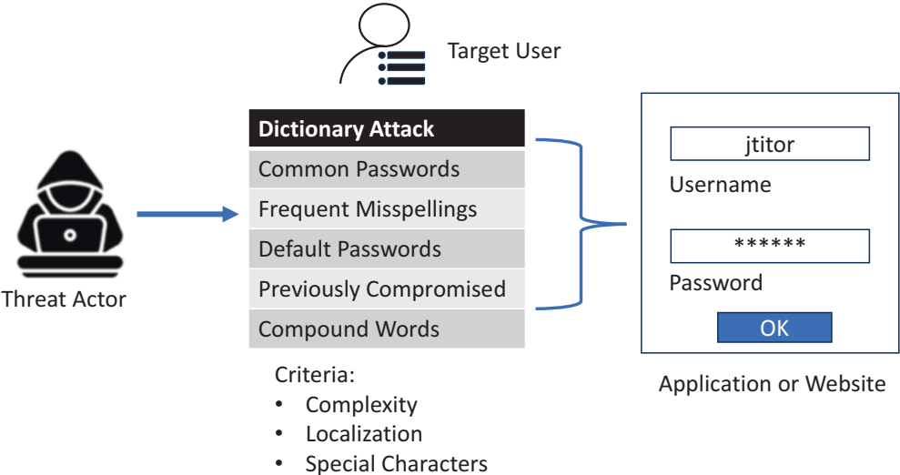
Figure 10-3. A threat actor’s approach to a dictionary attack
