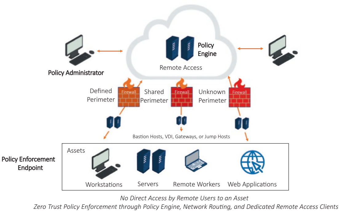
Figure 19-8. A zero-trust architecture for remote access technology
