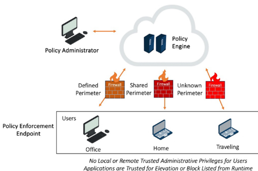
Figure 19-9. Zero-trust least privilege and endpoint privilege management architecture
