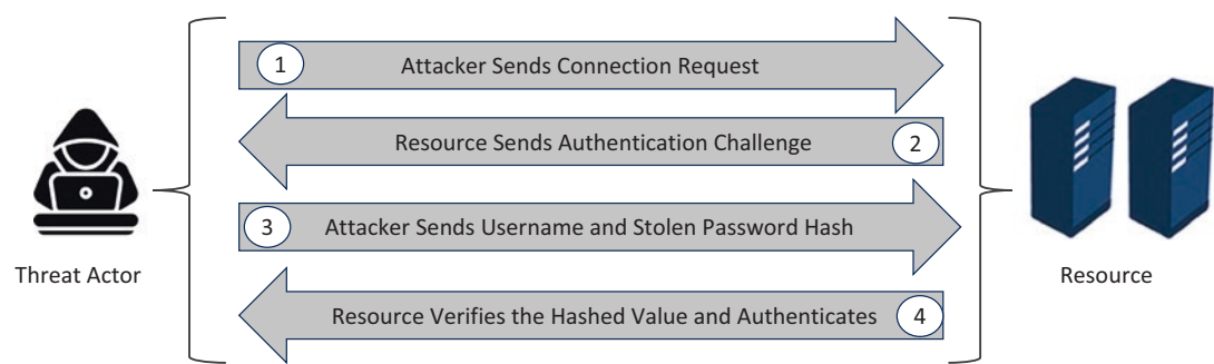
Figure 10-5. Pass-the-Hash simplified workflow for a stolen hash used for authentication
