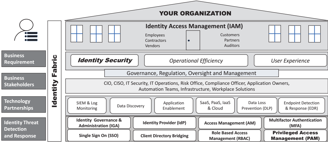
Figure 7-1. IAM discipline model
