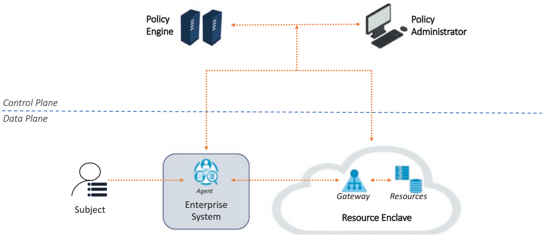
Figure 19-5. Basic zero-trust reference architecture
