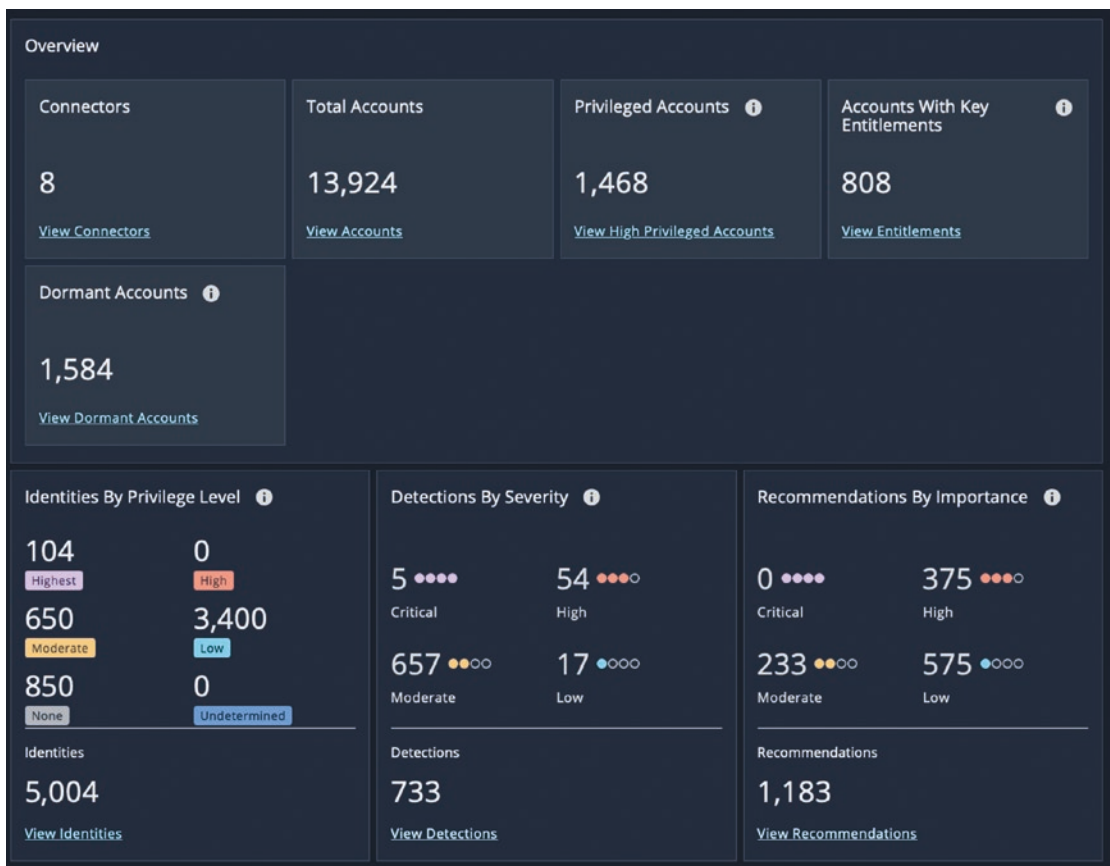
Figure 15-2. Identity security view of account and privileged risks with an organization as an integrated solution overlay
