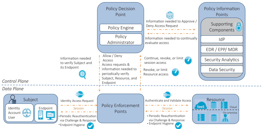
Figure 19-3. Sample zero-trust architecture from NIST 1800-35B
