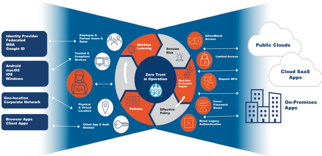
Figure 19-1. End-to-end zero-trust workflows in an environment
