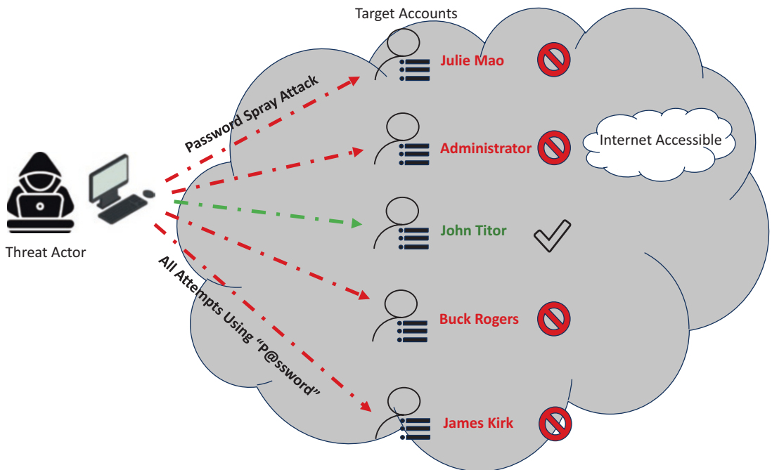
Figure 10-7. Spray attack conducted on the Internet
