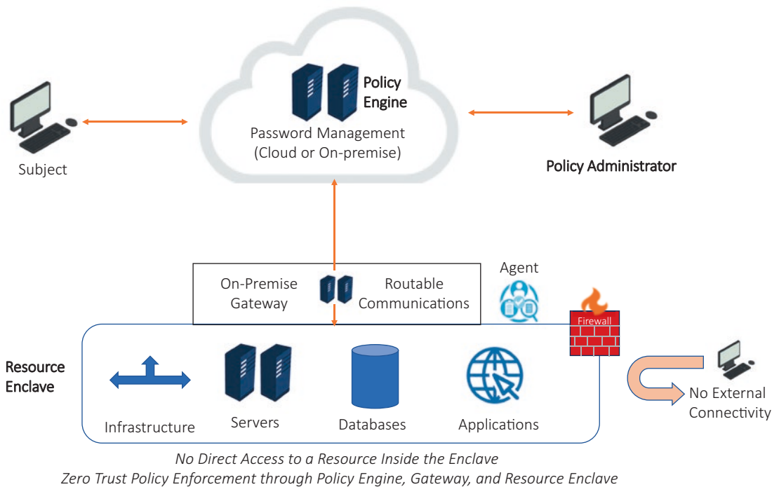
Figure 19-6. Privileged password and secrets management applied to zero trust
