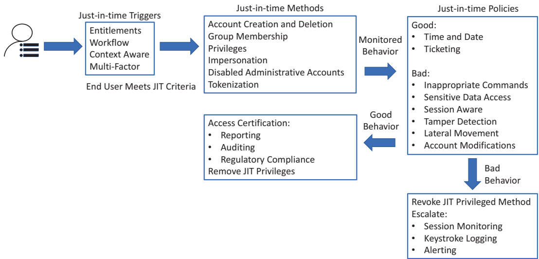
Figure 18-1. Just-in-time workflows based on triggers, methods, policies, and privileges
