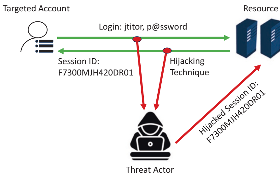
Figure 10-8. Token hijacking where the technique for session ID theft has been simplified as a part of the workflow
