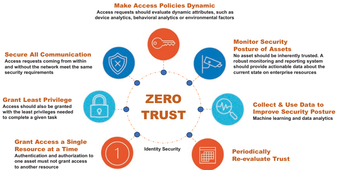
Figure 19-2. Seven tenets of zero trust as defined by NIST
