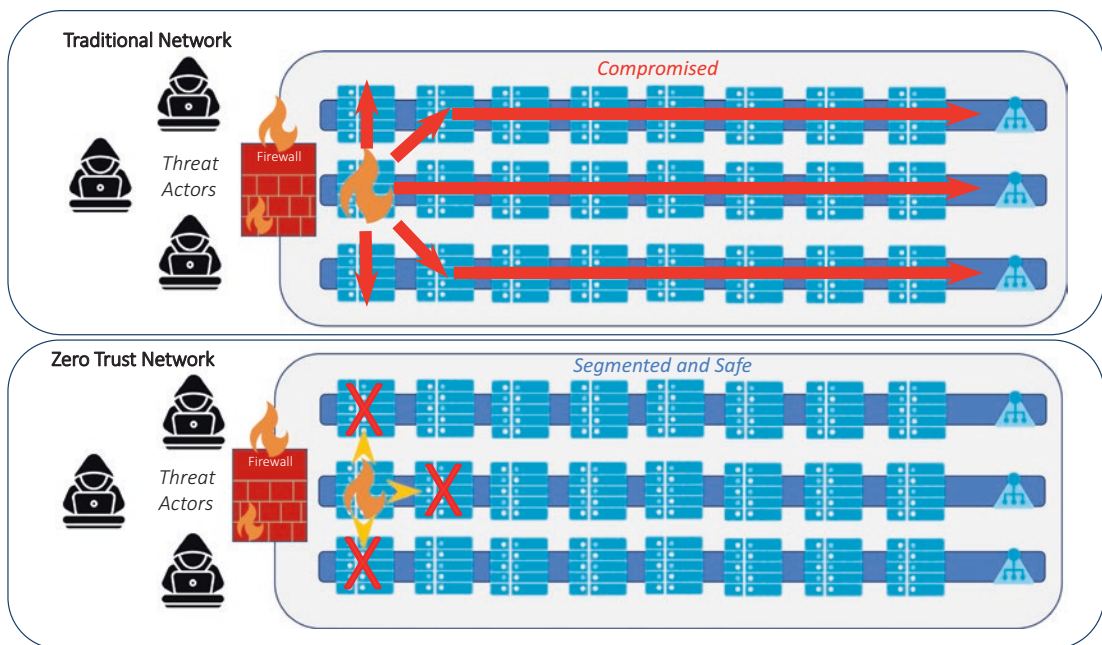
Figure 19-4. Zero-trust exposure vs. network-based security controls
