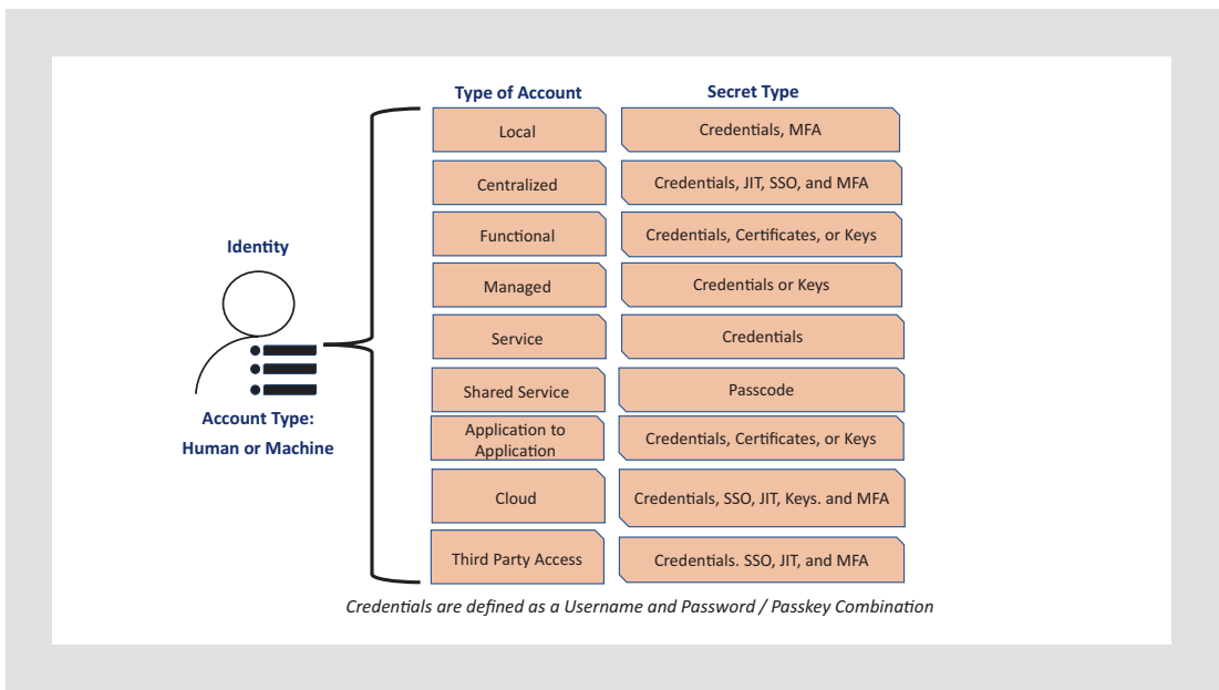
Figure 6-2. Basic identity, account, and credential relationship
