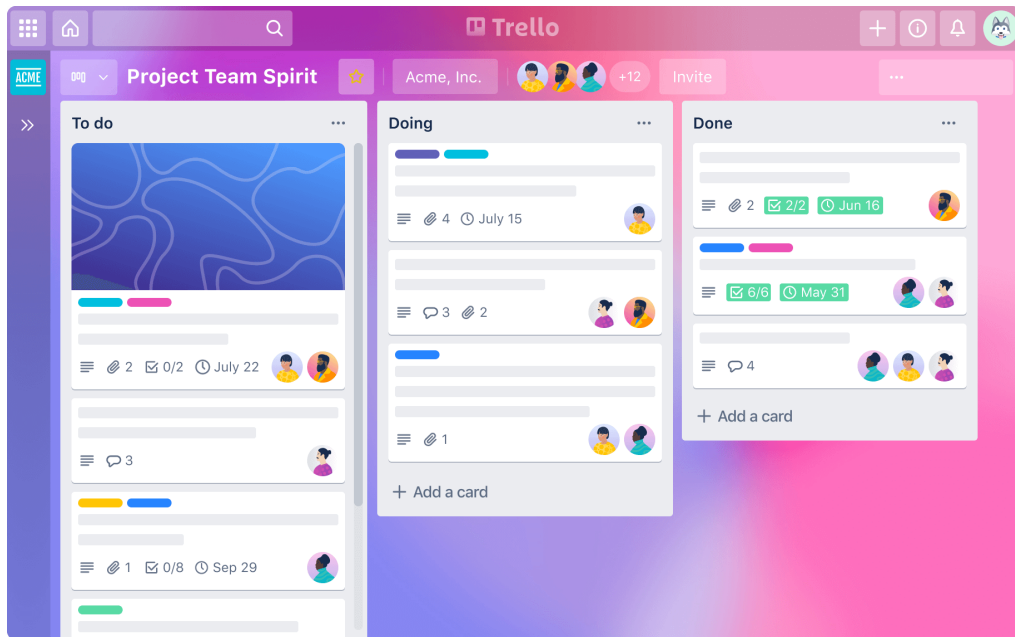
Figure 1.3: Trello board
