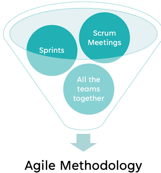
Figure 1.2: Agile methodology
