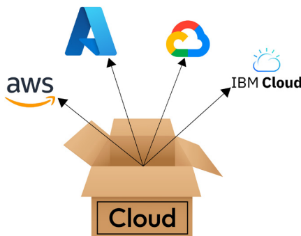
Figure 3.1 – Multi-cloud environment
