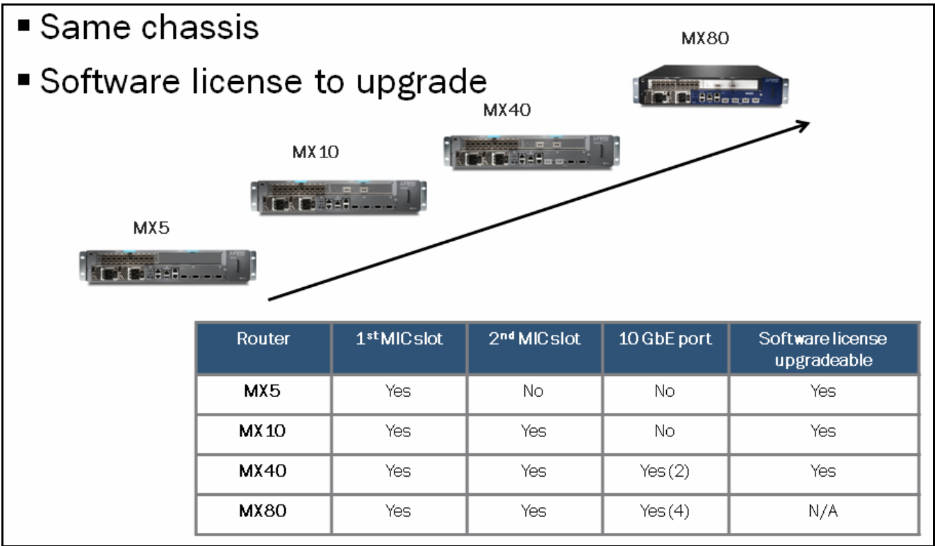
The graphic shows some of the highlights of the MX Series devices.
