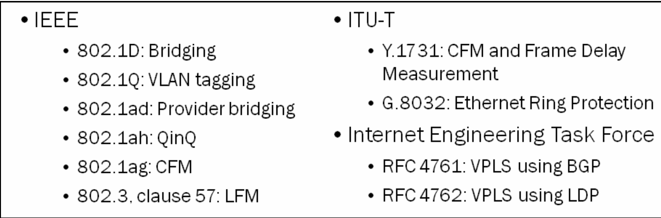
The graphic shows some of the Layer 2 features supported on MX Series devices.
