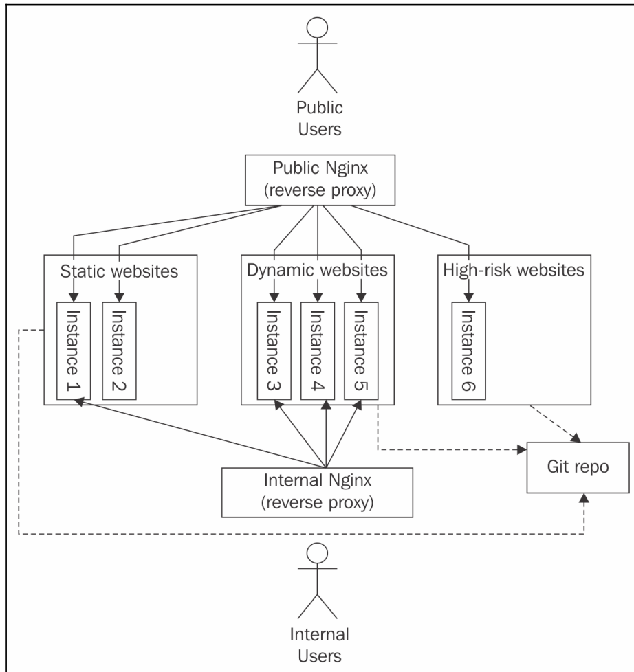
High-level overview of website deployment
