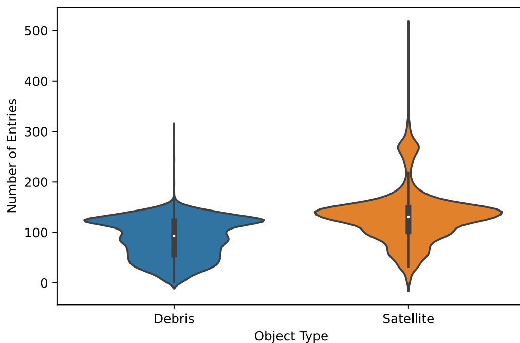
Figure 9.12: The distribution of SSA entries by object type. The width of each plot is proportional to the number of objects which have been updated at a given annual rate.
