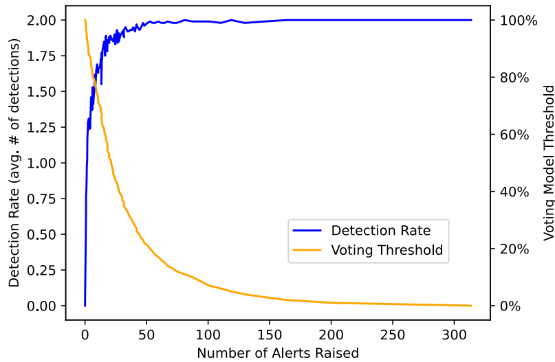
Figure 9.17: Defense Performance over 10,000 Simulations. At high voting thresholds, a defender receives fewer annual alerts, but may miss the spy satellites.
