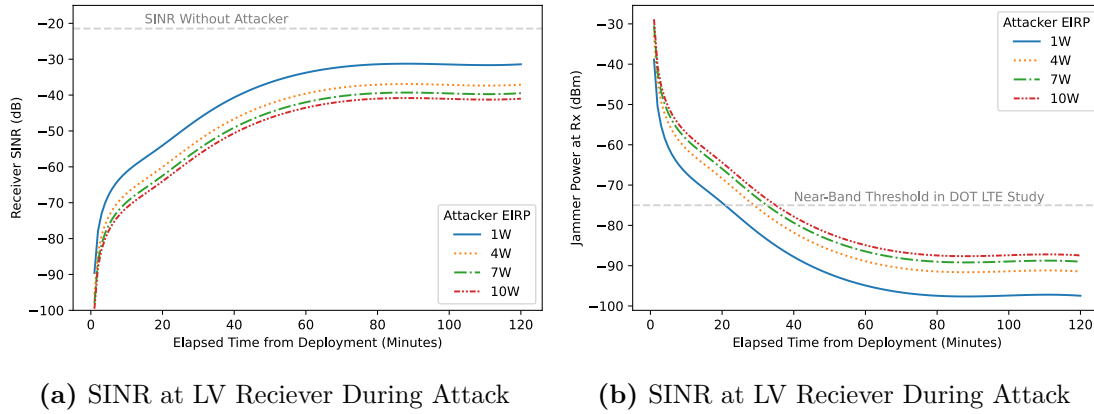
Figure 10.2: Attack Simulation Results.
