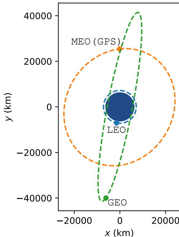
Figure 9.1: Depiction of Common Earth Orbits. Note that GEO satellites are beyond the range of GPS signals.
