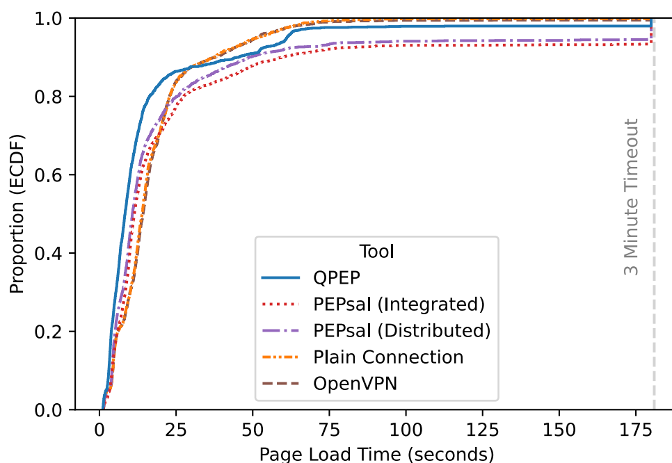
Figure 6.10: ECDF of Alexa Top 20 PLTs in Iridium Simulation. As expected, QPEP offers very little benefit in this lower-latency environment. However, it also imposes smaller overheads than traditional unencrypted PEPs.
