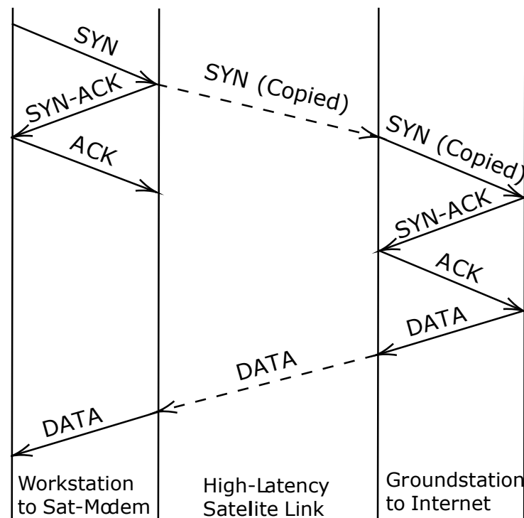
Figure 6.2: Split Distributed PEP Handshake Example
