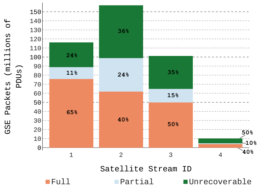
Figure 5.6: The degree to which GSE packets within a given stream were recoverable. Stream 4 was of significantly lower throughput than the others and was included to assess GSEextract’s performance in lower bandwidth contexts.
