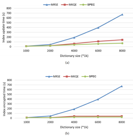
Figure 4. (a) update index time starting with 1000 with update index; (b) Index encryption time comparison with 1000 file indexes encrypted.
