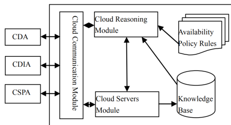
Figure 5. CDAA architecture.
