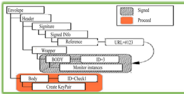
Figure 2. XML data security.
