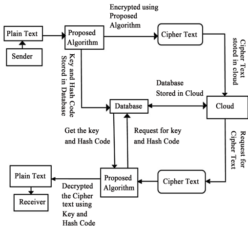
Figure 14. Proposed model of data storage in cloud using the proposed algorithm.
