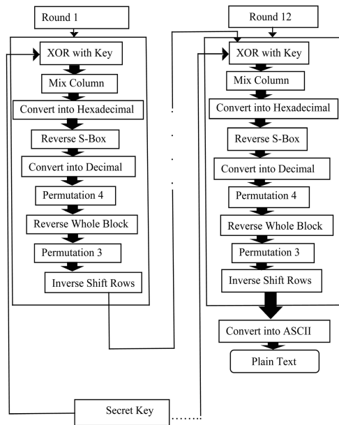
Figure 8. Round function of decryption process.
