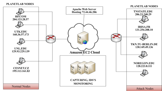
Figure 3. Testbed network architecture for DDoS [5.2].
