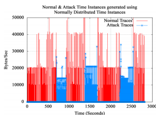
Figure 4. Network traces generated using normal time instances.
