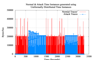
Figure 5. Network traces generated using uniform time instances.
