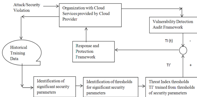
Figure 2. Organization control framework for cloud services.
