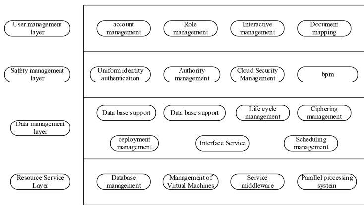
Figure 2. The structure for basic services layer.
