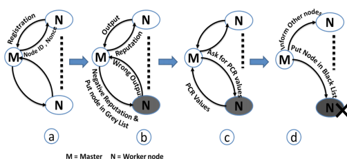
Figure 9. Working of our framework.
