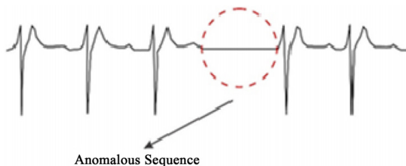
Figure 4. Collective anomaly.
