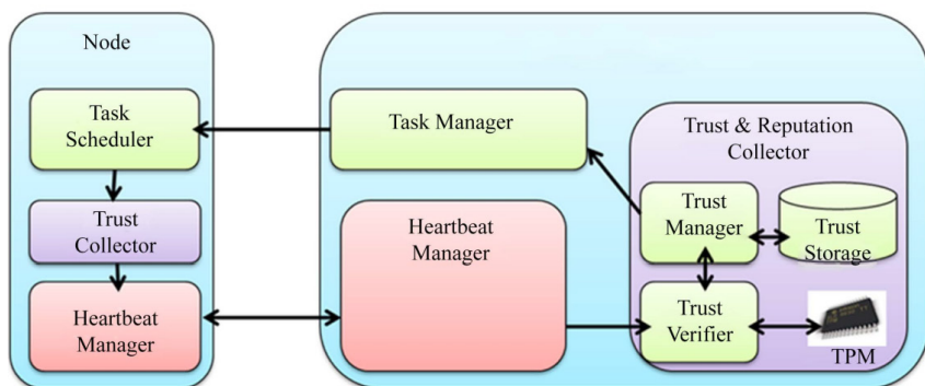
Figure 4. Architecture of trusted heartbeat framework.
