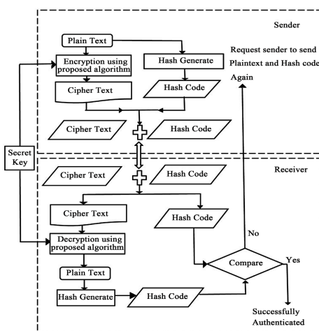
Figure 2. Flowchart of encryption and decryption process overview.
