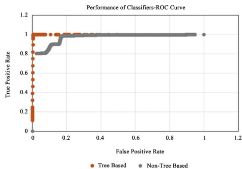
Figure 7. Classifiers’ performance comparison. 6
