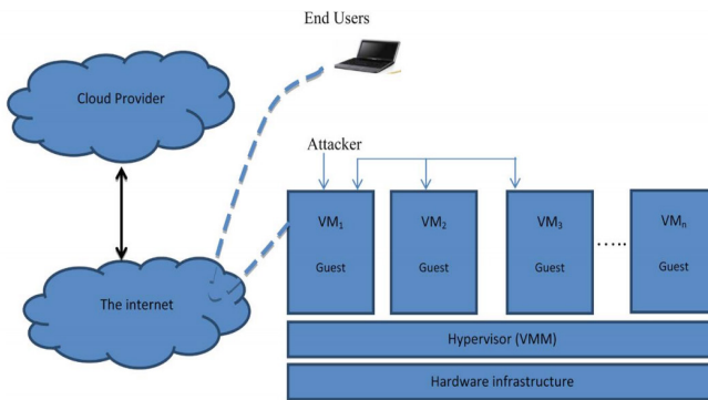
Figure 2. Attack on Virtual Cloud Computing Infrastructure (VCCI).
