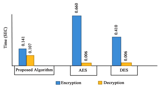
Figure 16. Encryption and decryption for 384-bit data.
