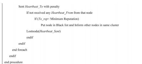
Figure 8. Procedure for reputation based decision.
