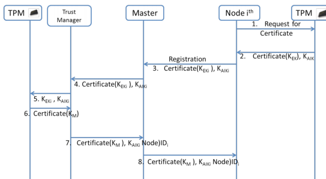
Figure 6. Step by step node registration procedure.
