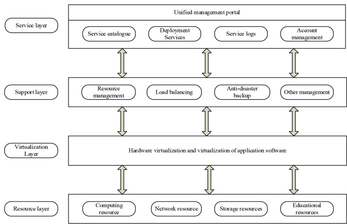
Figure 1. The framework for infrastructure layer.
