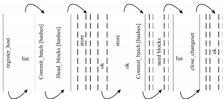
Figure 6. Illustration of Dropbox protocol.
