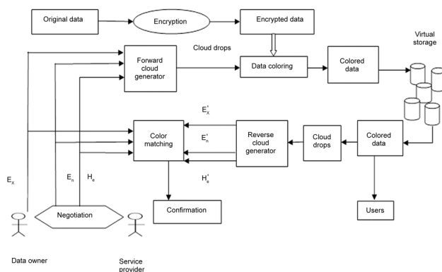
Figure 4. Block diagram for color coding generation.
