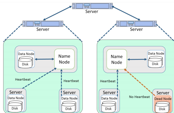
Figure 3. Heartbeat in Hadoop environment adopted from [12].
