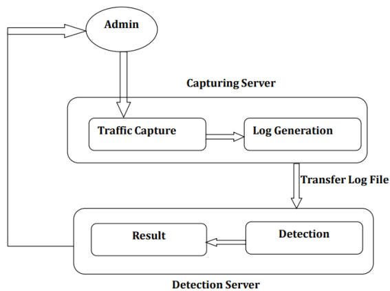
Figure 3. Phases of Hadoop DDoS detection framework. 2
