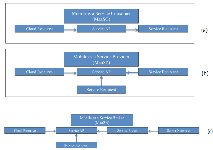
Figure 2. Mobile cloud computing service models: (a) Mobile as a service consumer model; (b) Mobile as a service provider; (c) Mobile as a service broker.
