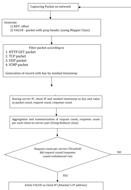
Figure 5. Counter-based DDoS detection algorithm using mapreduce. 4
