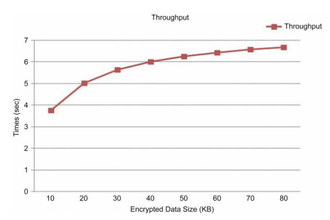
Figure 11. Encrypted data size vs time.
