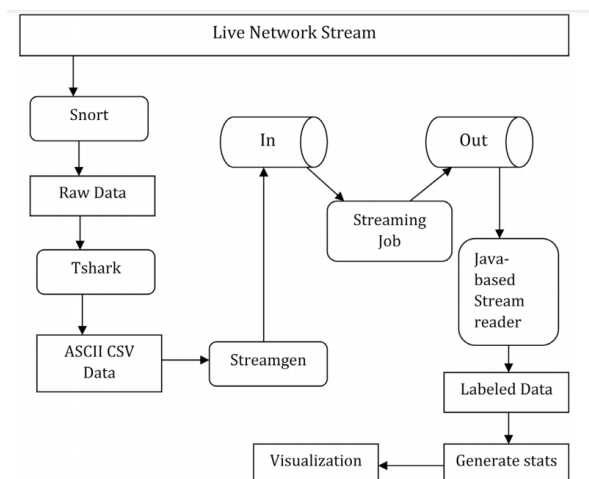
Figure 6. Proposed real-time intrusion through Hadoop and naive bayes. 5
