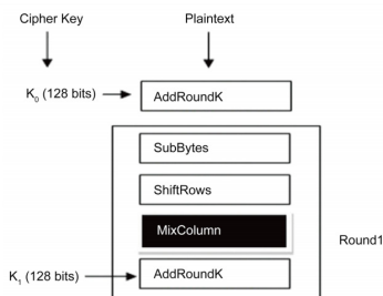
Figure 3. Block diagram for AES algorithm process.
