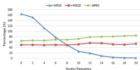
Figure 5. Percentage of files containing highest access frequency. Keywords in the top 20 locations.
