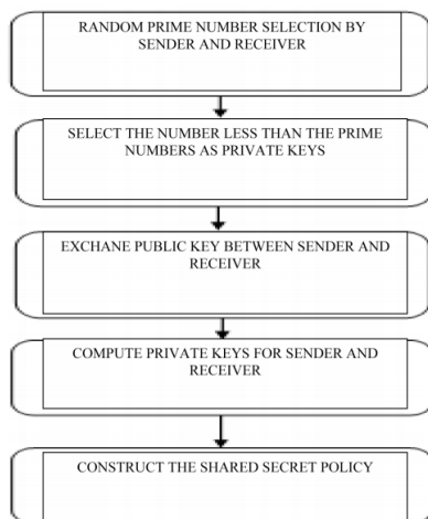
Figure 5. Workflow of key exchange.
