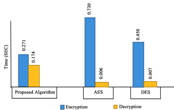
Figure 17. Encryption and decryption for 576 bit data.
