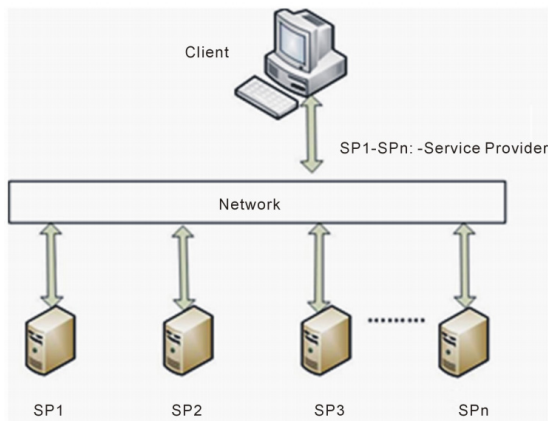
Figure 1. Proposed RSSNS architecture for cloud data storage.
