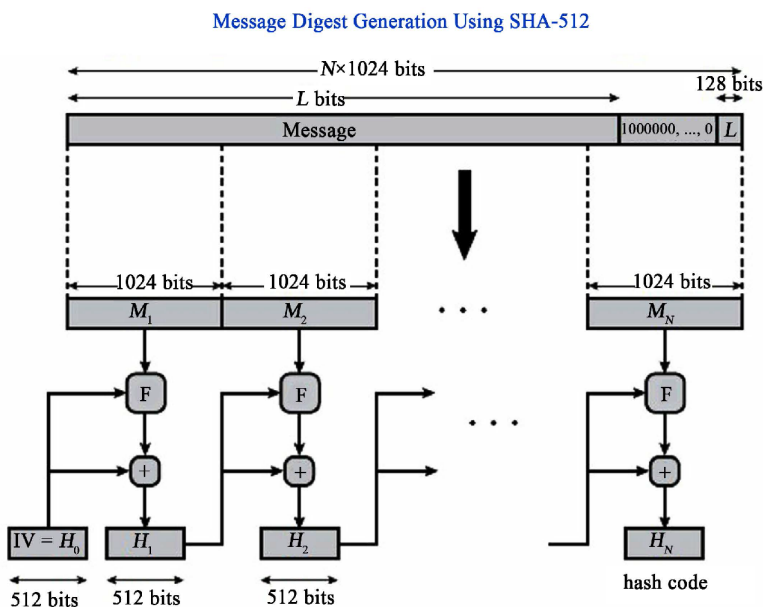
Figure 3. Message digest generation using SHA-512 (“message digest generation using SHA 512-Google search”) [22] .
