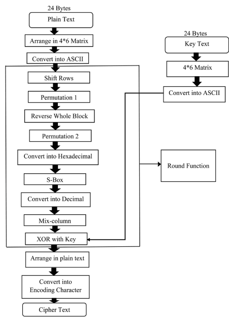
Figure 5. Encryption process flowchart.
