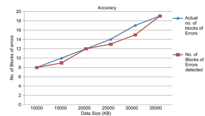
Figure 10. Detection of errors with various block size.
