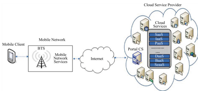
Figure 5. Mobile communication with cloud domain and servers.
