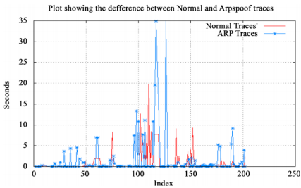
Figure 7. Difference between normal and ARP spoof traffic from same Planet-Lab nodes.
