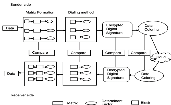
Figure 1. Architecture of the proposed system.
