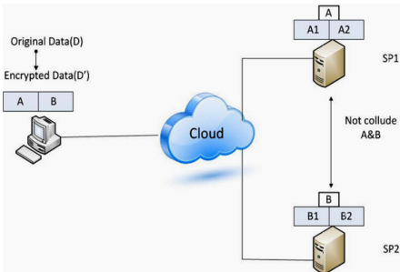
Figure 5. Security of the proposed architecture.
