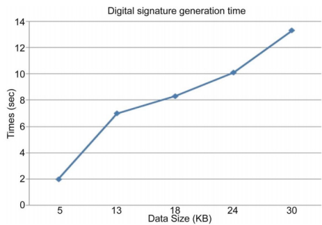
Figure 7. Generation of digital signature.
