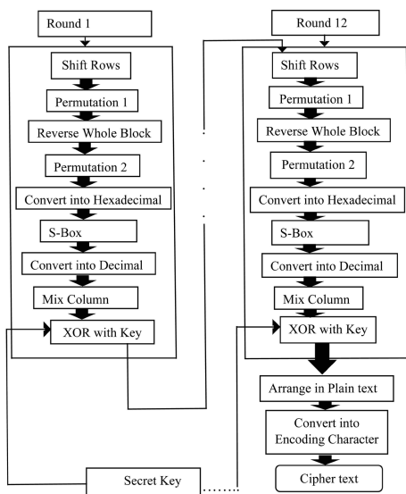
Figure 6. Round function of encryption process.
