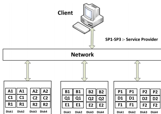
Figure 2. Proposed RSSNS architecture with three service providers.
