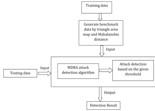
Figure 8. Attack detection flowchart. 7
