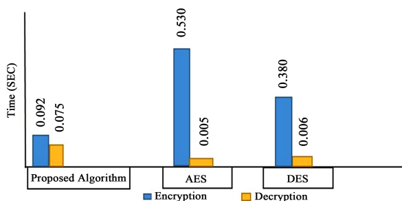
Figure 15. Encryption and decryption for 192-bit data.
