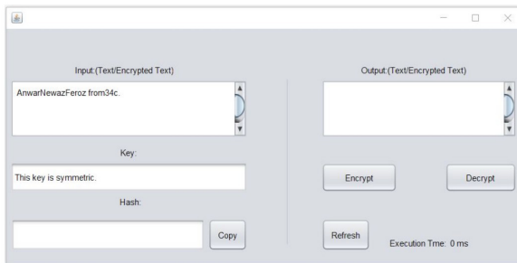
Figure 10. Encryption of data in Java interface.
