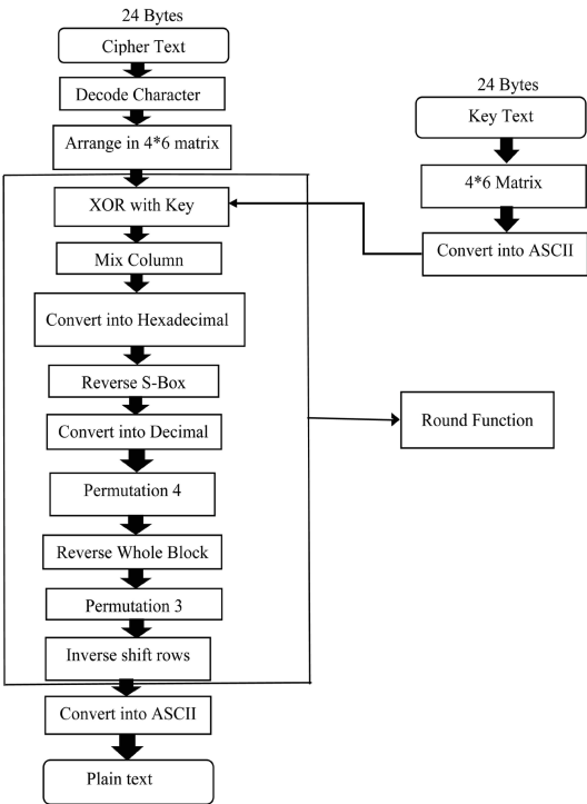
Figure 7. Decryption process flowchart.
