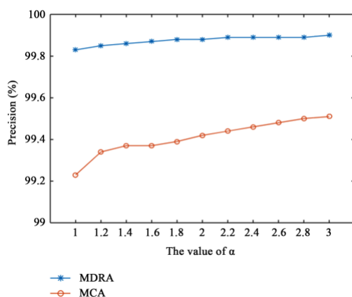
Figure 10. Using precision to compare detection based on MDRA and MCA. 9
