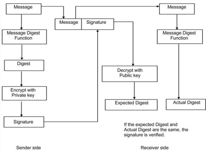
Figure 2. Block diagram for generation of digital signature.
