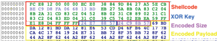
Figure 17 - Breakdown of a shellcode stager
