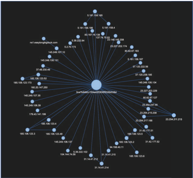
Figure 91 - Clustering TA575/Dridex infrastructure using SSL public key Hash
