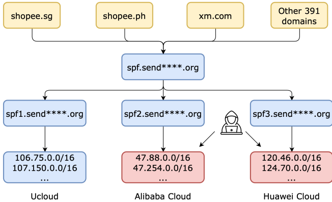
Fig. 11. SPF Dependency Tree of S.
