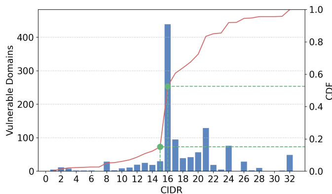
Fig. 10. CIDR Prefix Length Analysis of SPF-vulnerable Domains.
