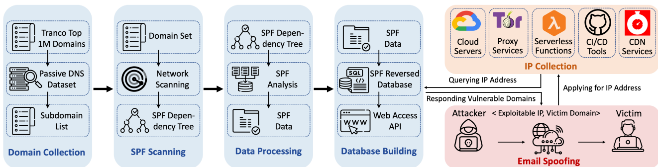
Fig. 6. Exploitation Workflow of BreakSPF Attack.
