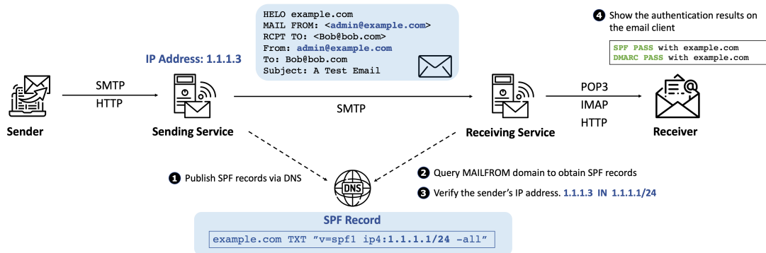
Fig. 1. SPF Verification Workflow.
