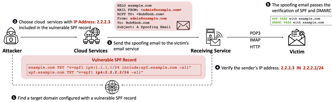
Fig. 3. BreakSPF Attack Model.
