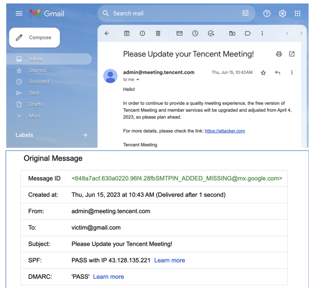
Fig. 12. A spoofing email sent to Gmail impersonating admin@meeting.tencent.com . The spoofing email passed the verification of SPF and DMARC.
