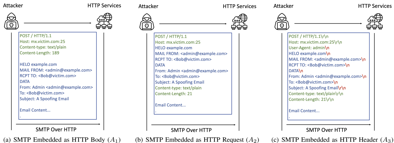
Fig. 5. Cross-Protocol Email Spoofing Attack Techniques.
