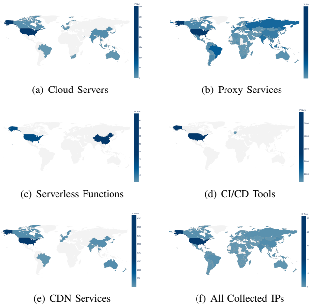
Fig. 8. Global Distribution of Collected IPs from Different Sources in Our Experiment.
