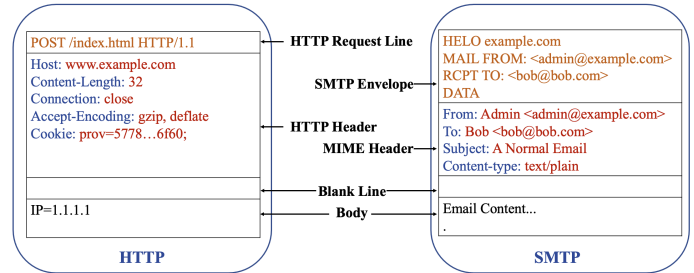
Fig. 4. The Similarities between HTTP and SMTP.
