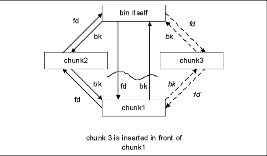
Figure 6.9 Frontlinking a Chunk
