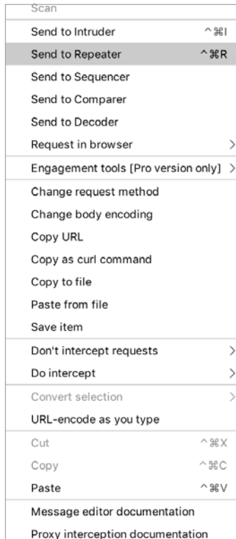
Figure 4-9: You can forward the request or response to different Burp modules by right-clicking it.
