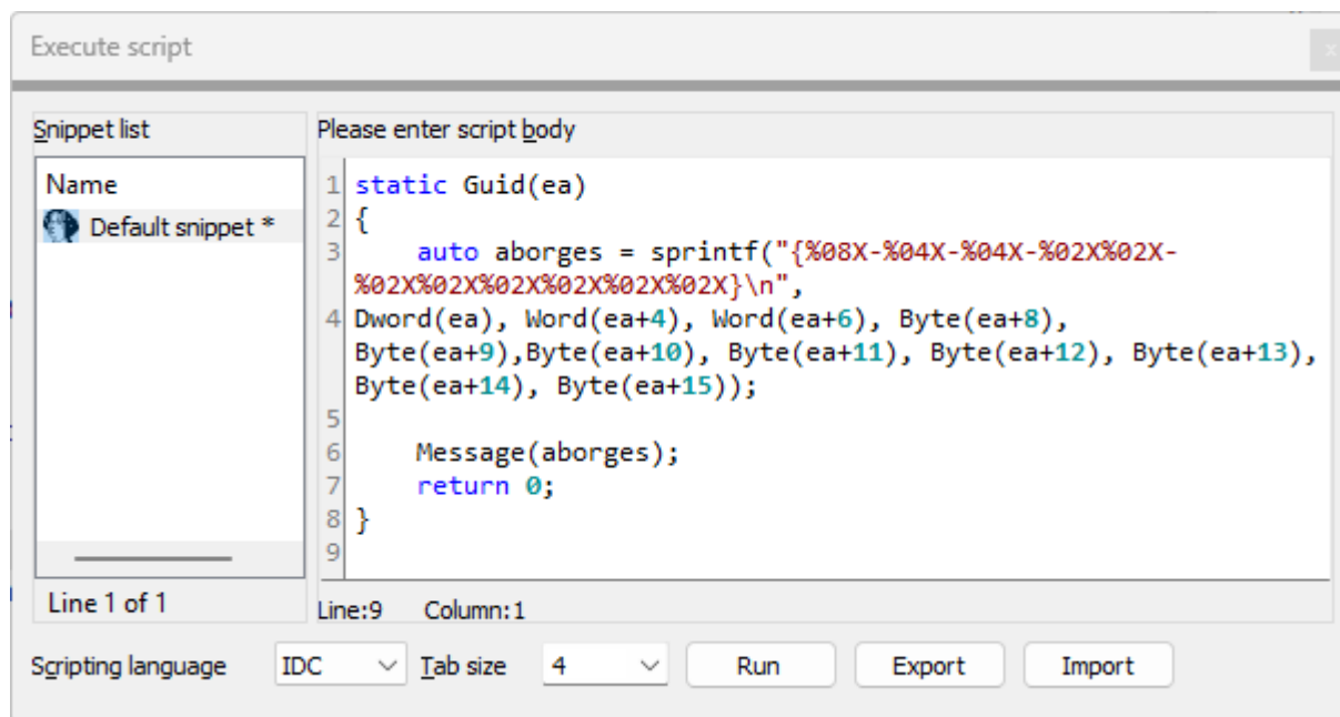
[Figure 91] IDC script to format GUID
