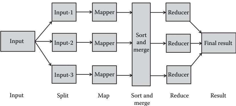
FIGURE 6.5 Computation of MapReduce. (From Jayaraj, A. et al., Programming Models for Clouds .)
