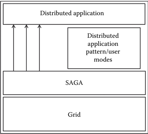
FIGURE 8.9 SAGA architecture. (Adapted from SAGA tutorial, available: http://www.cybertools.loni.org/rmodules.php .)
