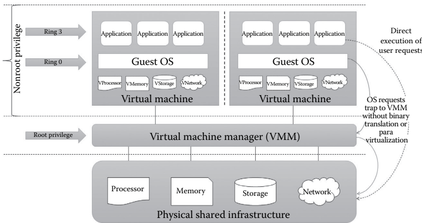
FIGURE 7.12 Hardware-assisted virtualization.
