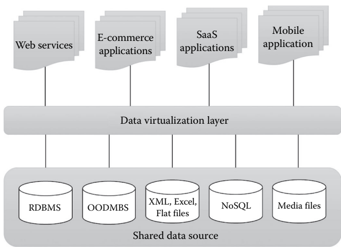
FIGURE 7.7 Data virtualization.
