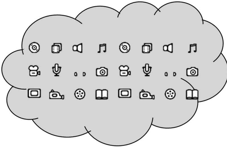
FIGURE 14.7 Multimedia cloud.
