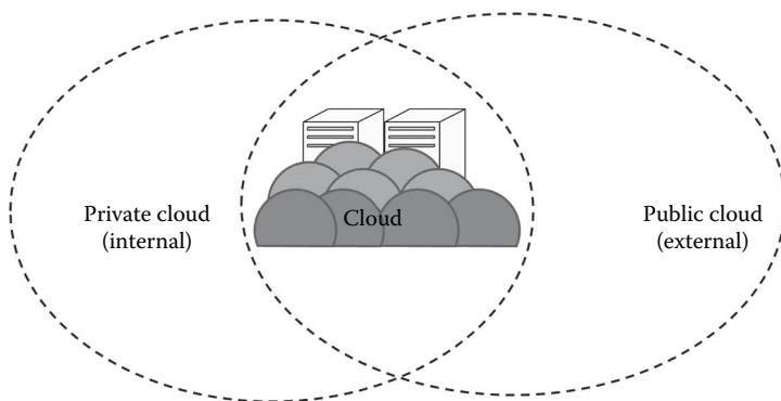
FIGURE 4.6 Hybrid cloud.
