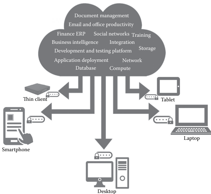
FIGURE 2.1 Cloud computing.
