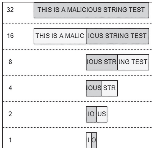
Figure 9-4: DefenderCheck's binary search
