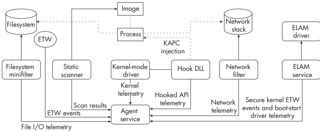
Figure 1-3: The intermediate agent architecture
