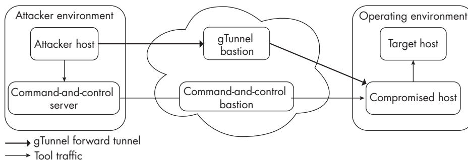
Figure 5-2: The gTunnel proxying architecture
