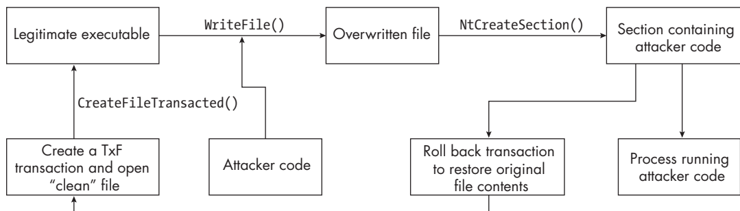
Figure 3-10: The execution flow of process doppelganging
