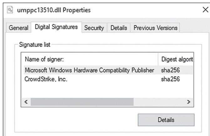
Figure 5-3: CrowdStrike Falcon's DLL countersigned by Microsoft
