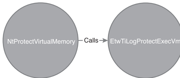
Figure 12-3: A simple path between a syscall and an EtwTi function
