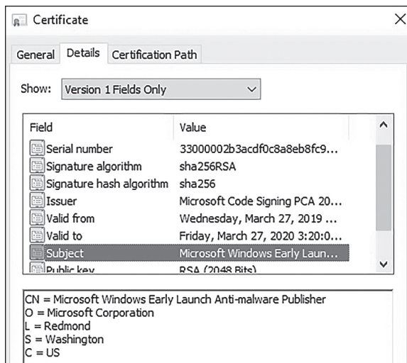
Figure 11-1: Microsoft's countersignature on an ELAM driver
