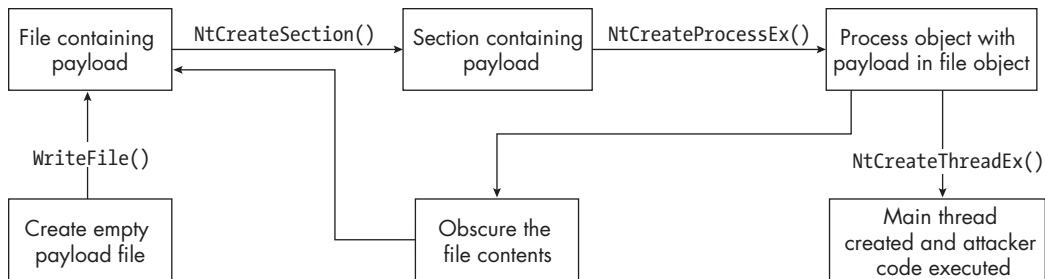
Figure 3-11: The execution flow of process herpaderping
