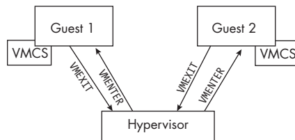
Figure A-1: The operation of VMEXIT and VMENTER
