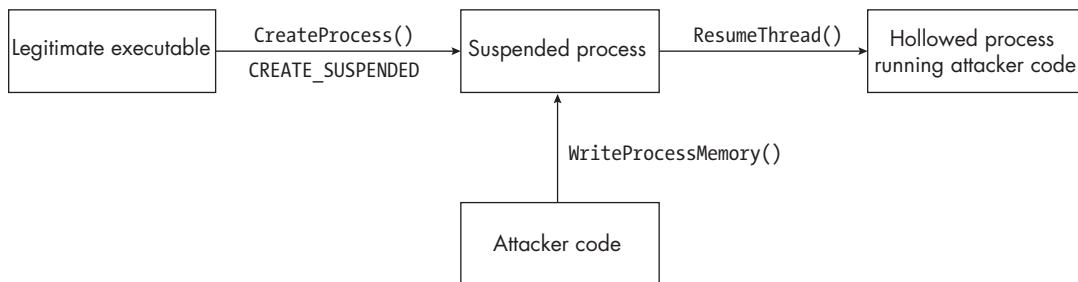
Figure 3-9: The execution flow of process hollowing
