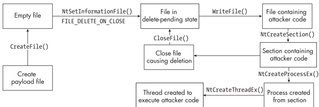
Figure 3-12: The process-ghosting workflow
