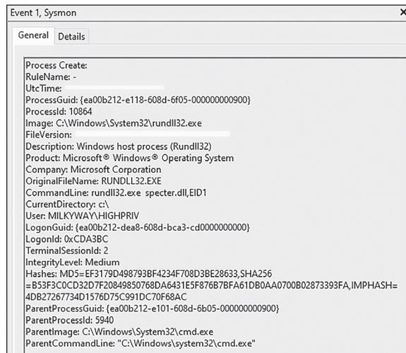
Figure 3-1: Sysmon Event ID 1 showing process creation
