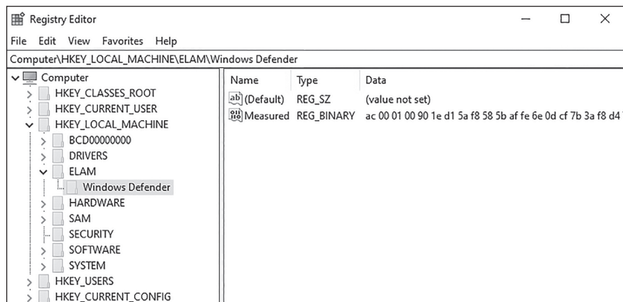
Figure 11-2: Microsoft Defender in the ELAM registry hive
