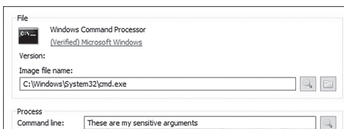
Figure 3-3: Command line arguments retrieved from the PEB
