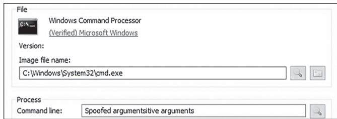
Figure 3-5: Command line arguments partially overwritten
