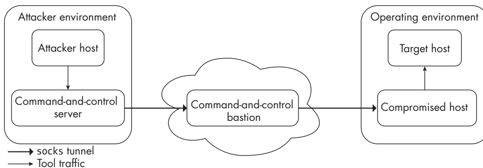
Figure 5-1: A generic proxying architecture
