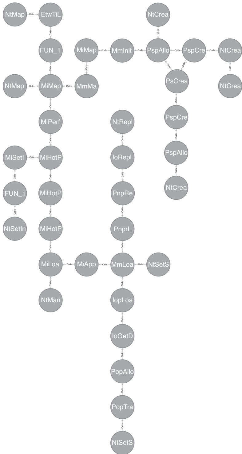
Figure 12-4: Paths from nt!NtCreatePagingFile() to nt!EtwTiLogMapView()
