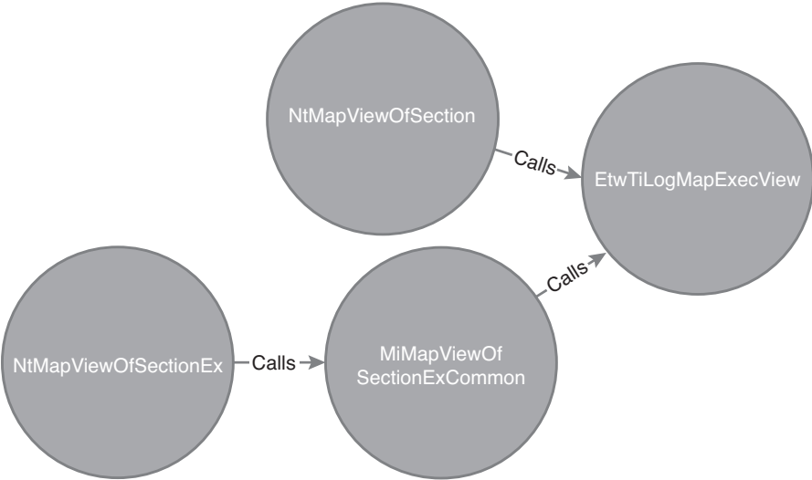
Figure 12-5: Scoped query that returns more useful results
