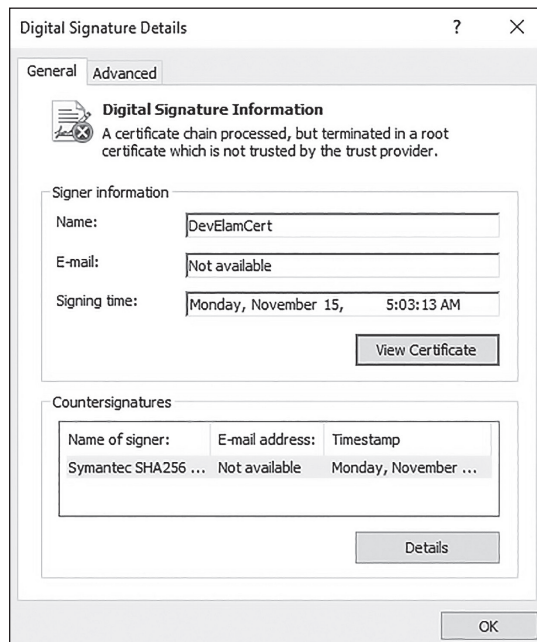
Figure 11-4: A signed driver with the timestamp included
