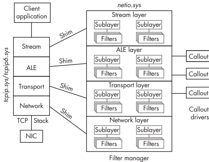
Figure 7-4: The WFP architecture
