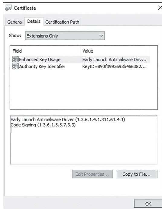
Figure 11-3: ELAM EKUs included in the certificate
