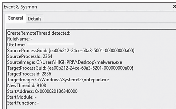
Figure 3-2: Sysmon Event ID 8 detecting remote thread creation
