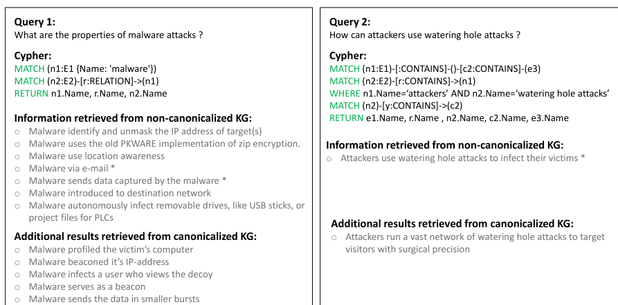
Fig. 10. Two sample query results as retrieved from Open-CyKG..
