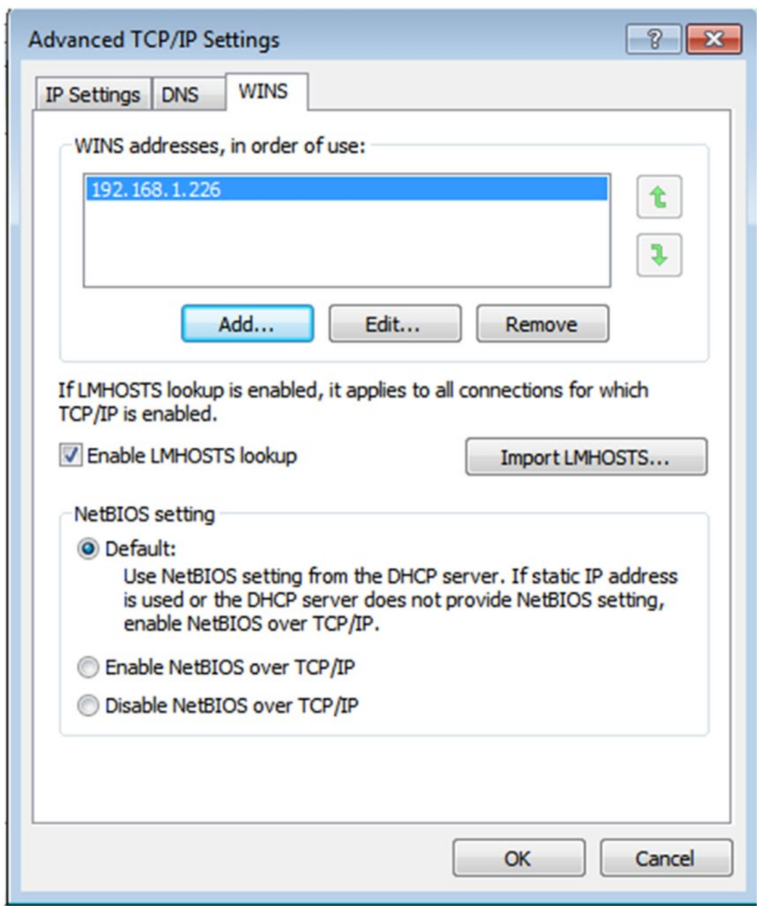
Figure 15-1. WINS server settings
