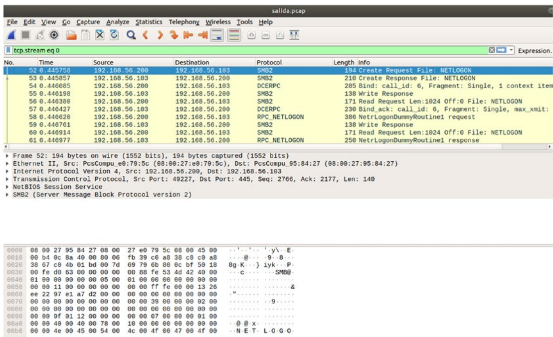
Figure 19-8. Communicating through the SMB version 2 protocol
