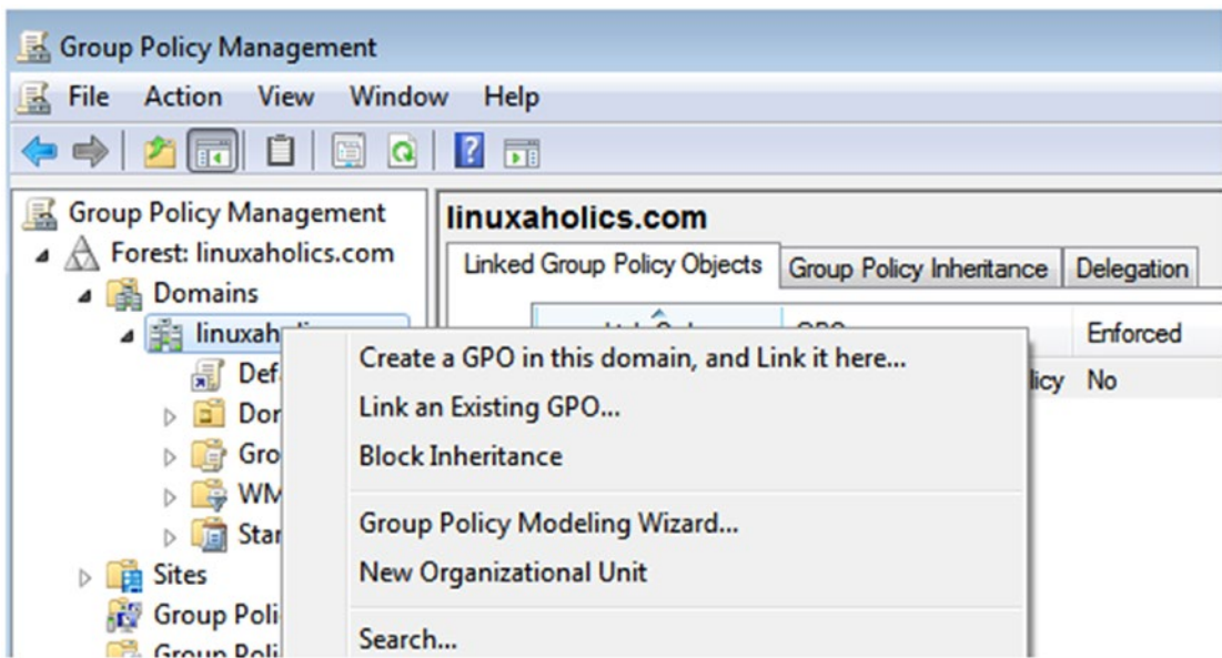
Figure 12-34. Creating a GPO
