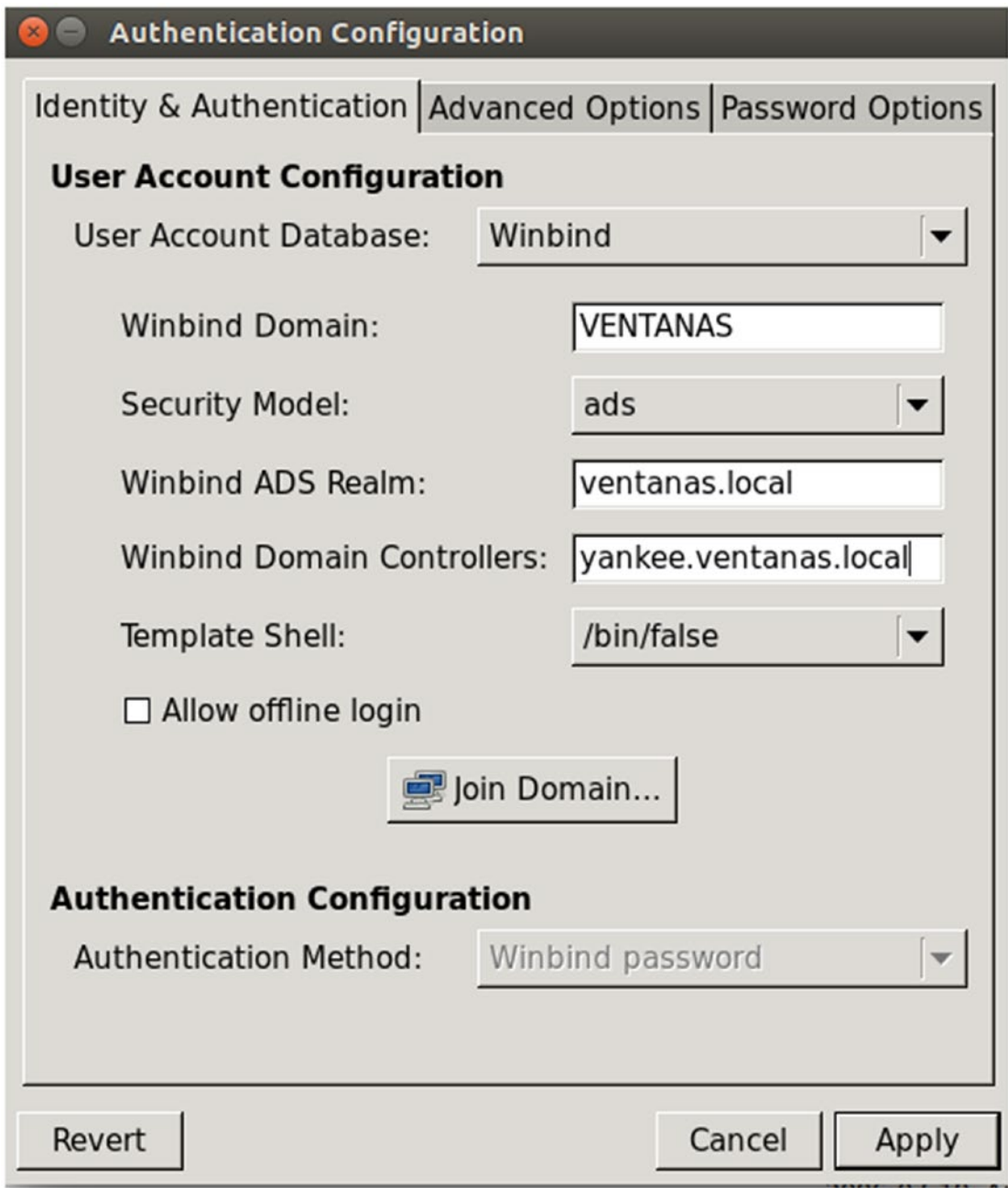
Figure 14-1. Setting up Winbind
