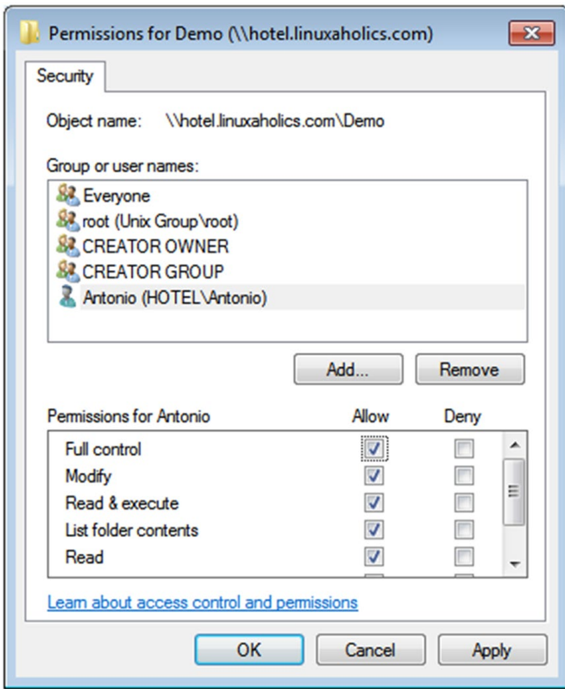
Figure 11-5. Modifying an ACL
