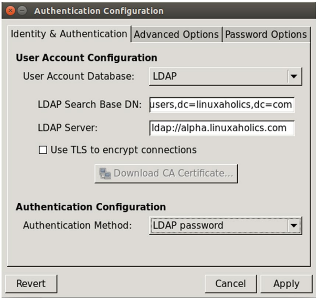
Figure 3-3. Configuring LDAP authentication
