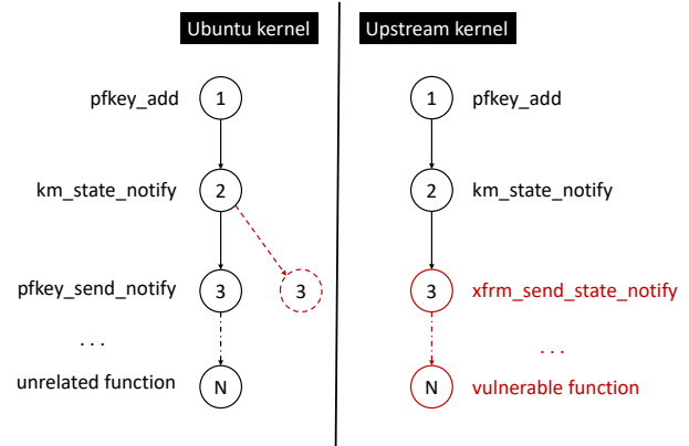
Figure 1: Motivation example
