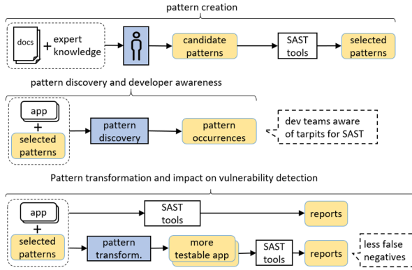
Fig. 1. Approach outline
