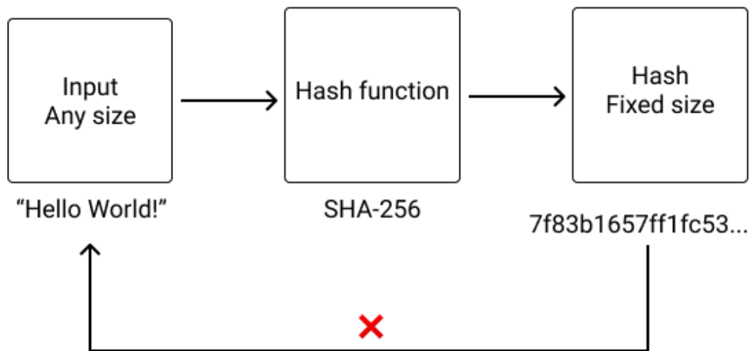
Figure 11.2: Hash function
