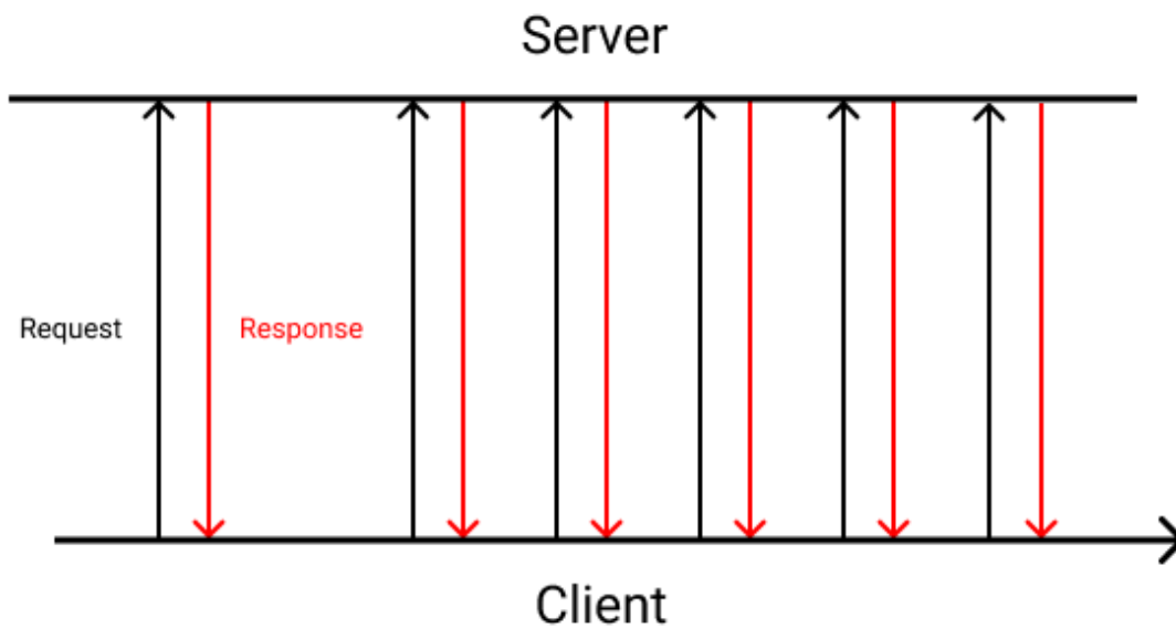
Figure 10.5: Short polling
