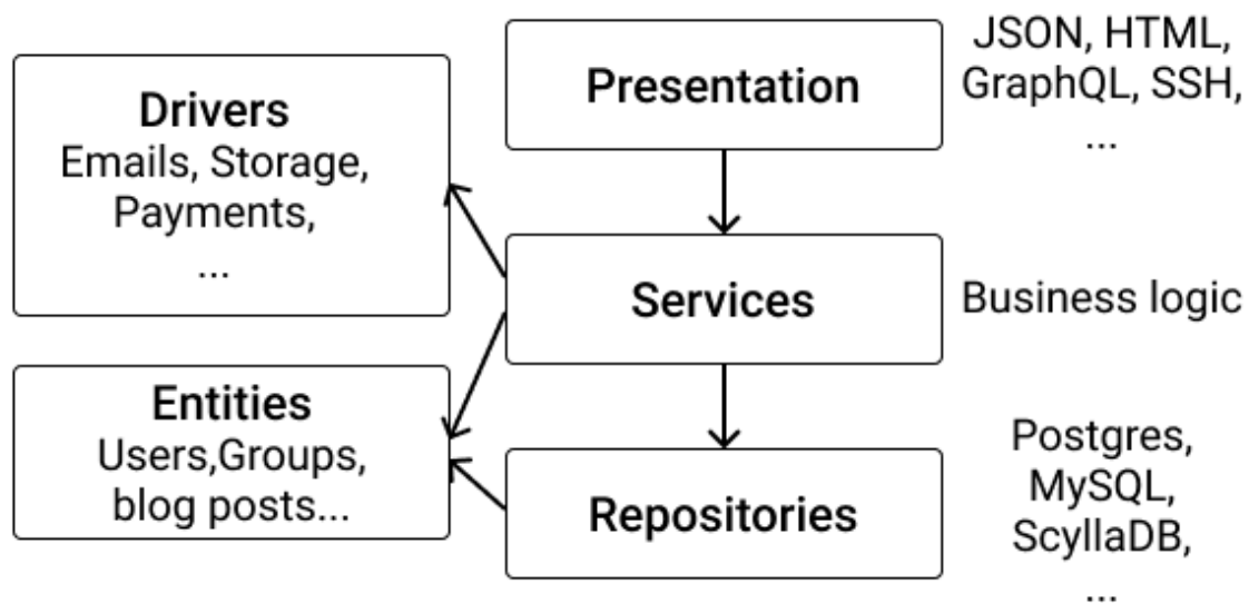
Figure 10.10: Server's architecture
