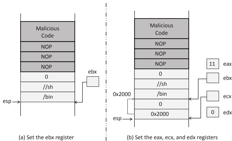
Figure 4.9: Shellcode Execution
