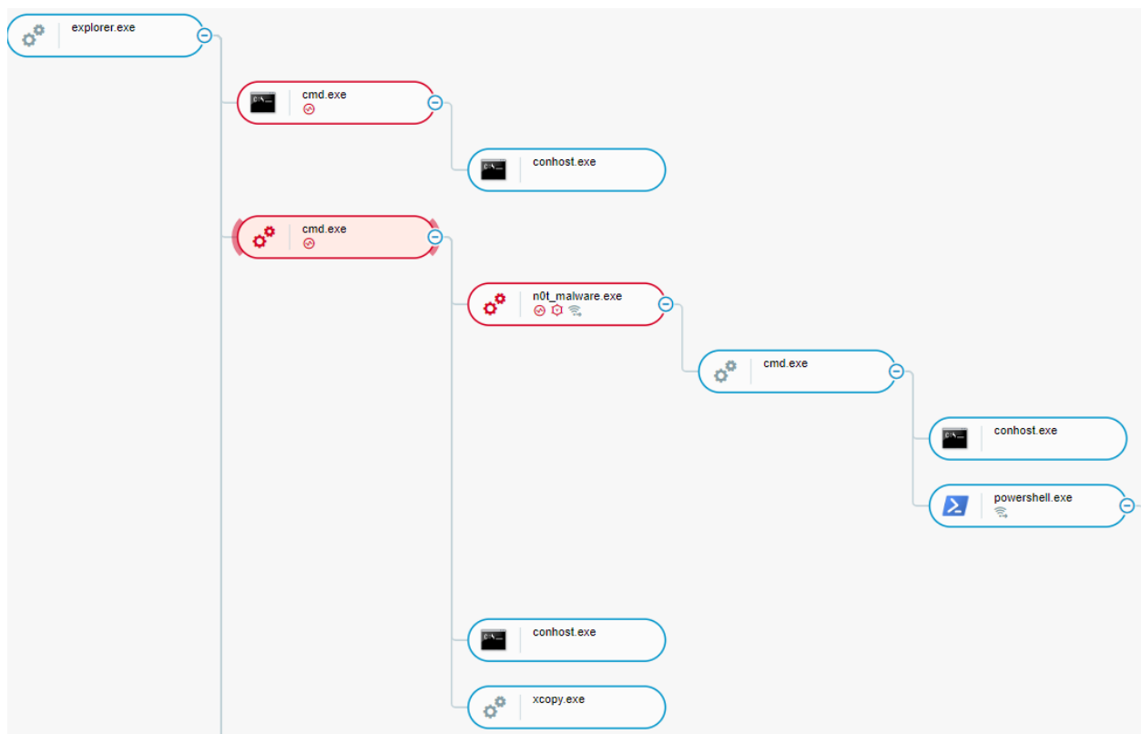
Process Tree
