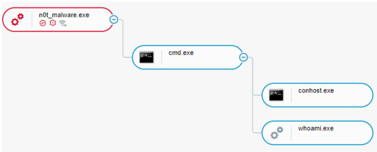
Process Tree
