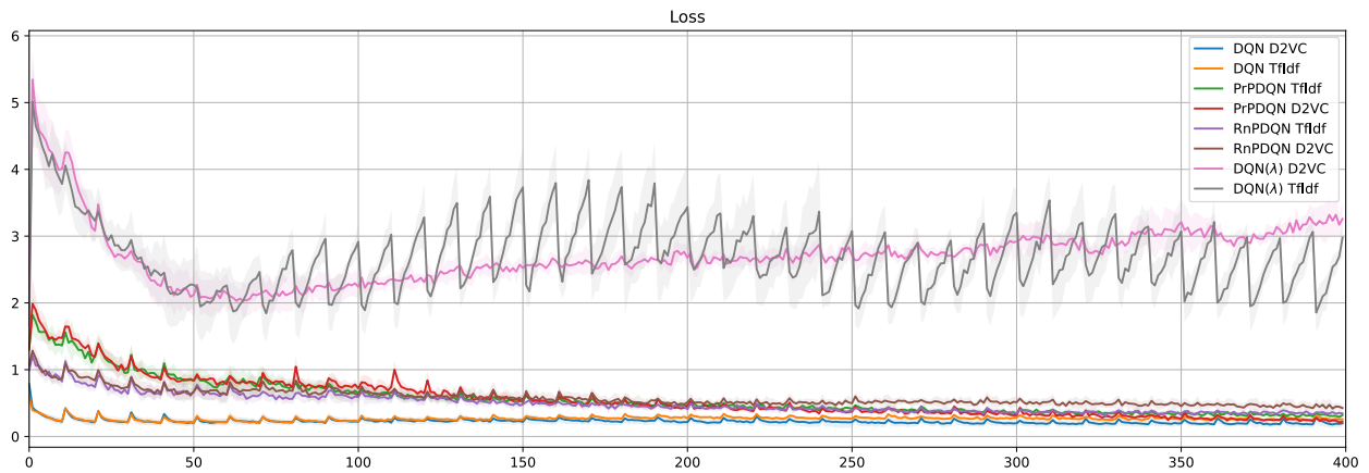
Figure 4.7: Loss evolution over training episodes. Continuous reward. The shaded areas are the 95% confidence intervals.
