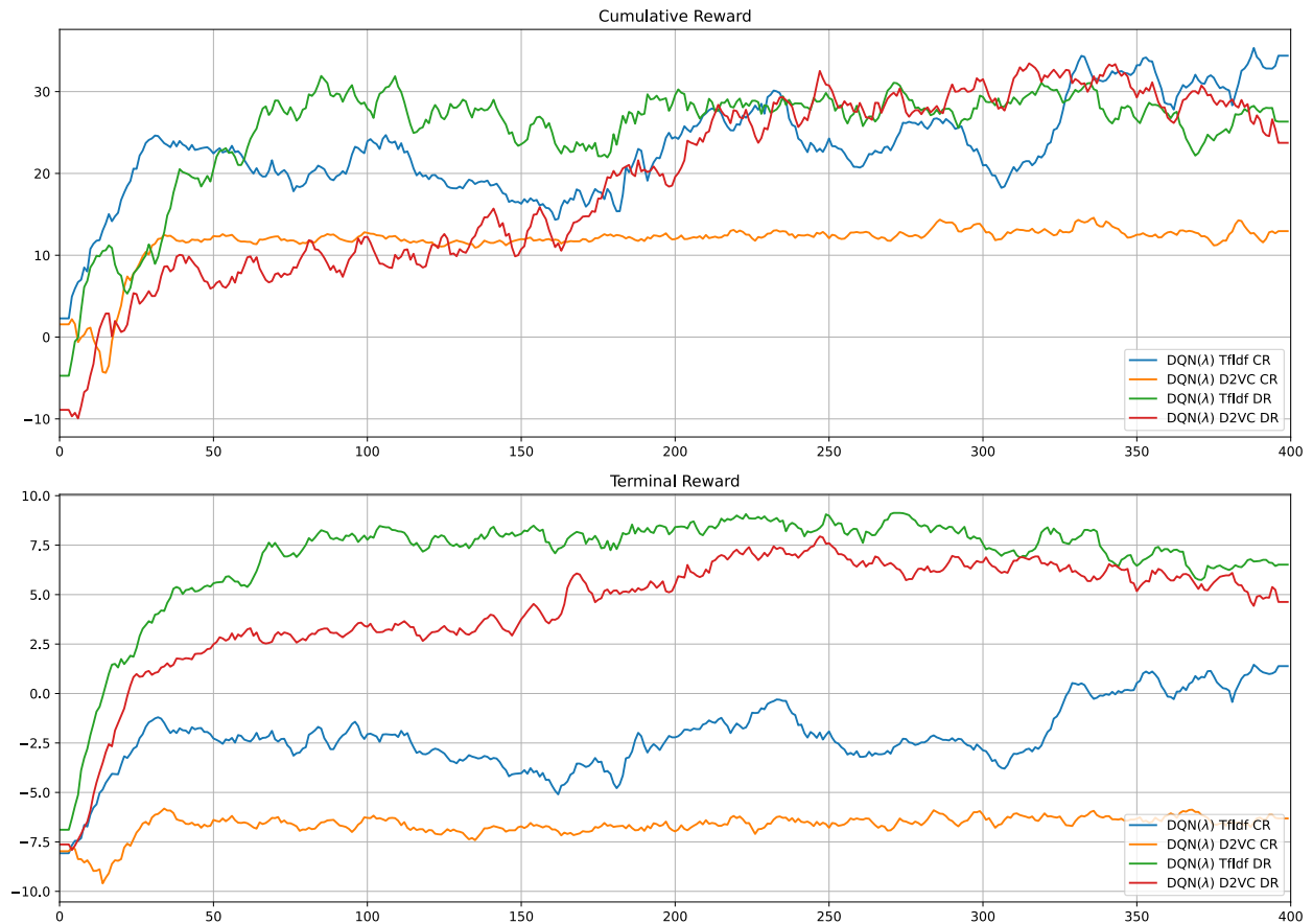
Figure 4.10: Comparison of different configurations of embedding method and reward function for the DQN(\lambda) model. CR: continuous reward, DR: discrete reward.
