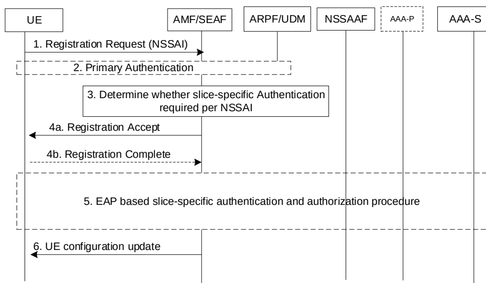
Figure 16.2-1: Relationship between primary authentication and slice-specific authentication and authorization
