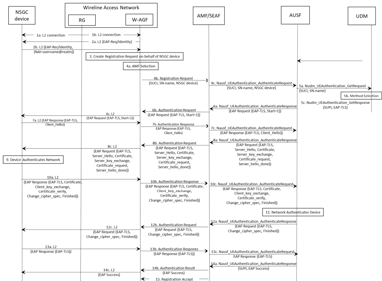
Figure O.3-1: Registration and authentication of a non-5G capable device to the 5GC
