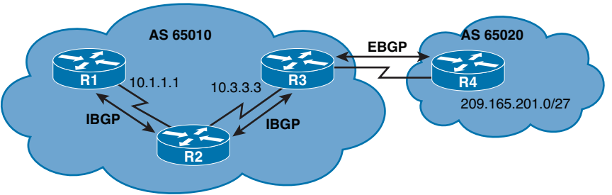
Figure 6-16 Route Reflectors
