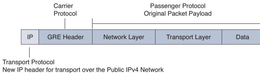
Figure 12-12 GRE Encapsulated Packet
