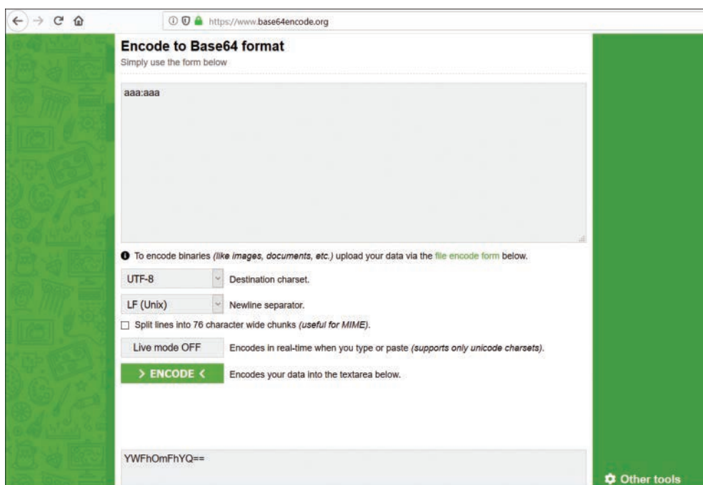
Figure 18-3 Converting a username:password Tuple to Base64 Format
