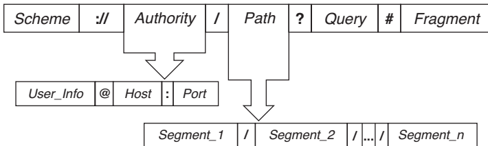
Figure 7-5 Generic Format of a URI
