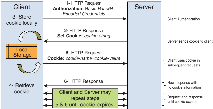
Figure 8-7 State Management Using Cookies: A Typical Workflow
