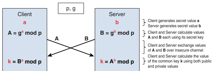
Figure 8-9 Diffie-Hellman Protocol Implementation
