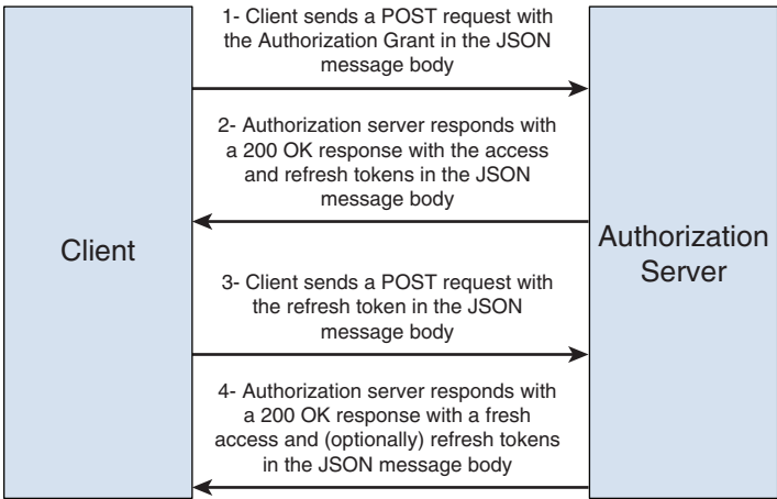
Figure 8-5 Workflow to Issue Access and Refresh Tokens to the Client
