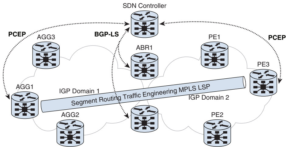
Figure 16-2 Underlay SDN Protocol Suite
