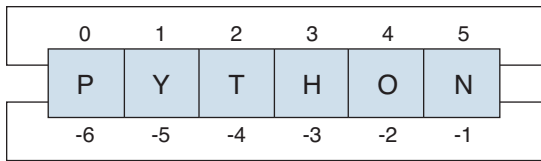
Figure 5-3 String Indexes
