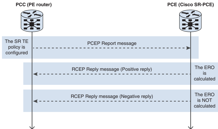
Figure 16-16 PCC-Initiated MPLS LSP
