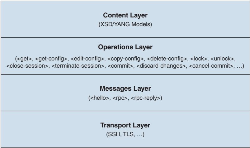
Figure 14-2 The Four-Layer Model Encompassing All NETCONF Functions
