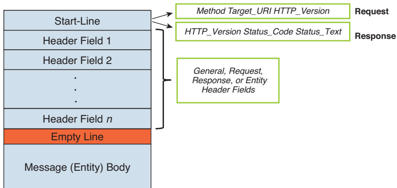
Figure 7-3 The HTTP Message Format
