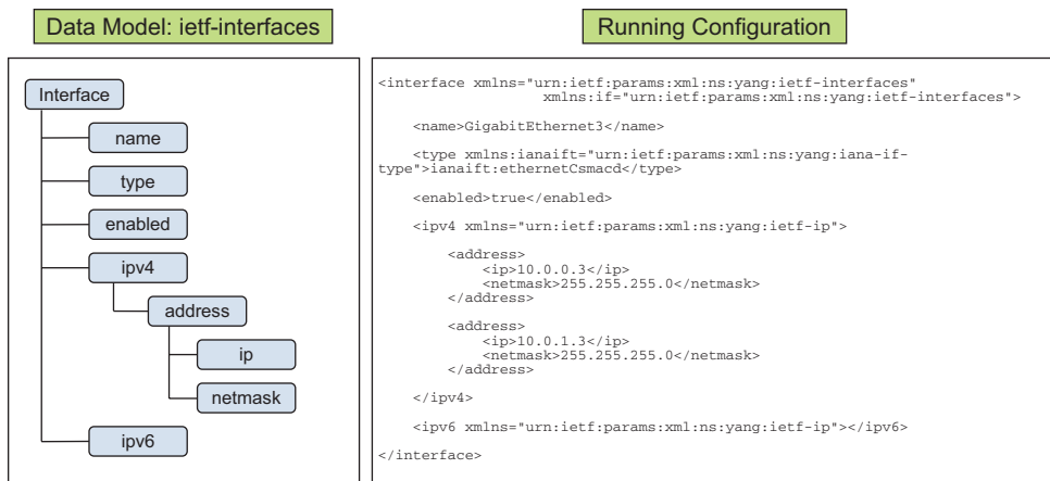
Figure 14-3 The Configuration Hierarchy in the ietf-interfaces YANG Model Mapped to the Configuration on the Device
