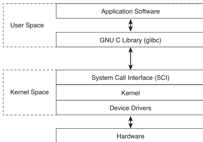
Figure 2-2 Communication Between Applications, Linux, and System Hardware
