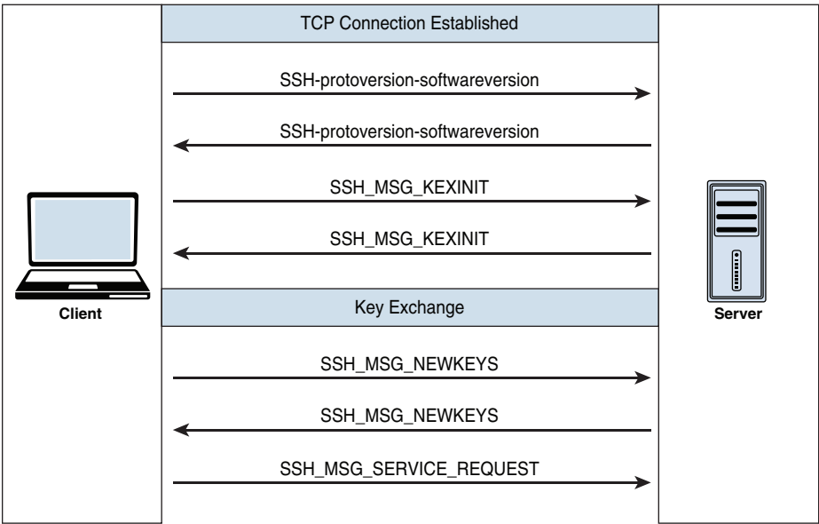
Figure 9-4 SSH-TRANS Protocol Packet Exchange
