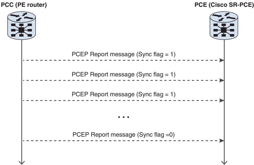
Figure 16-14 PCEP State Synchronization
