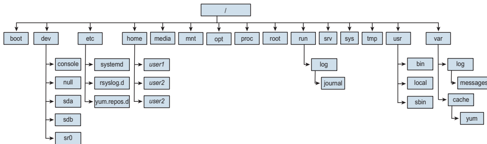
Figure 2-4 The Linux Directory Tree Structure, Starting at the Root (/) Directory and Branching Out
