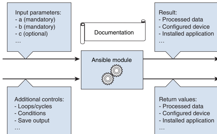
Figure 19-2 Structure of a Generic Ansible Module
