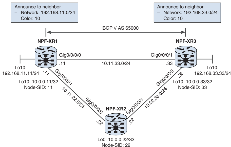
Figure 16-8 BGP Configuration for a Color Extended Community
