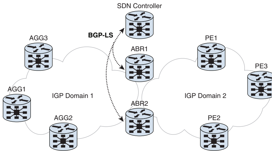
Figure 16-10 High-Level BGP-LS Peering Architecture
