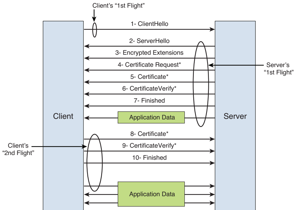
Figure 8-10 Simple 1-RTT TLS Workflow
