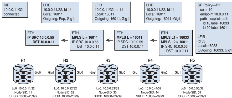
Figure 16-7 Generic Process of Segment Routing Traffic Engineering Using Node-SID
