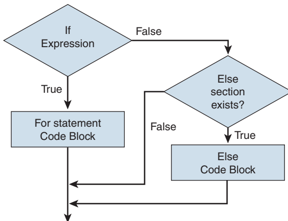
Figure 5-5 if-else Statement Flow Diagram
