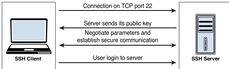
Figure 9-1 Simplified SSH Protocol Setup Flow
