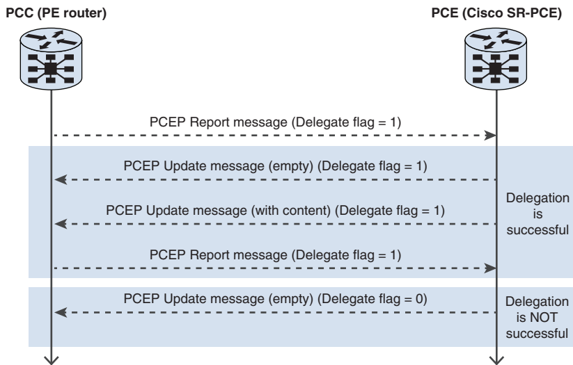
Figure 16-15 PCEP LSP Delegation Options
