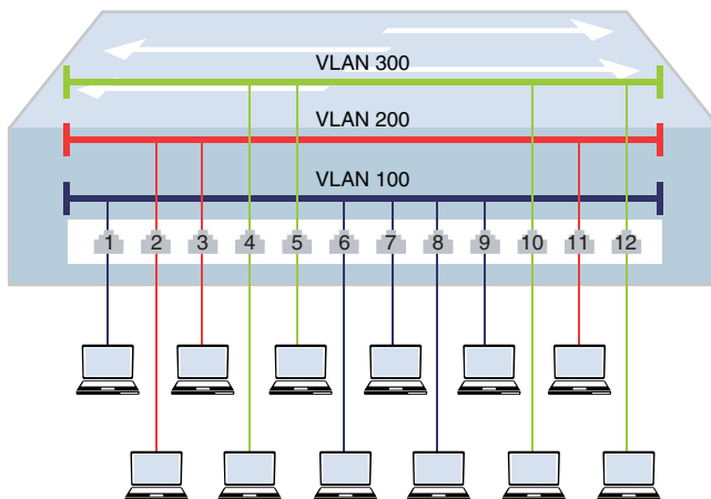
Figure 1-1 VLANs Connected to a Switch Are Not Aware of Each Other
