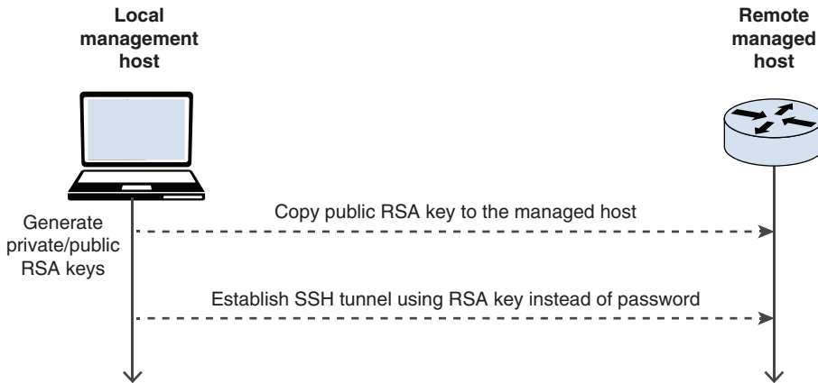
Figure 18-2 SSH with RSA Keys
