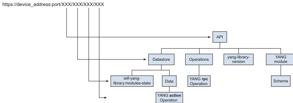
Figure 14-8 RESTCONF Resources and Their Relationship with the Resource URI
