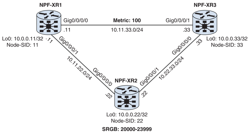
Figure 16-5 Segment Routing Topology with a Modified Metric and SRGB
