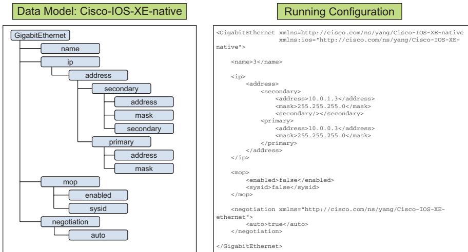
Figure 14-4 The Configuration Hierarchy in the Cisco-IOS-XE-native YANG Model Mapped to the Configuration on the Device
