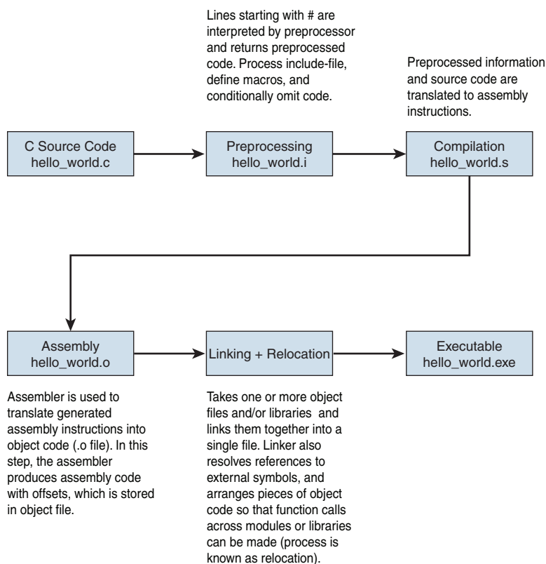
Figure 5-2 Compiling C into an Executable File
