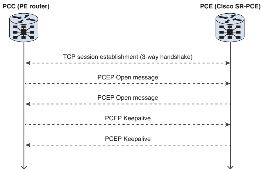
Figure 16-13 PCEP Session Establishment
