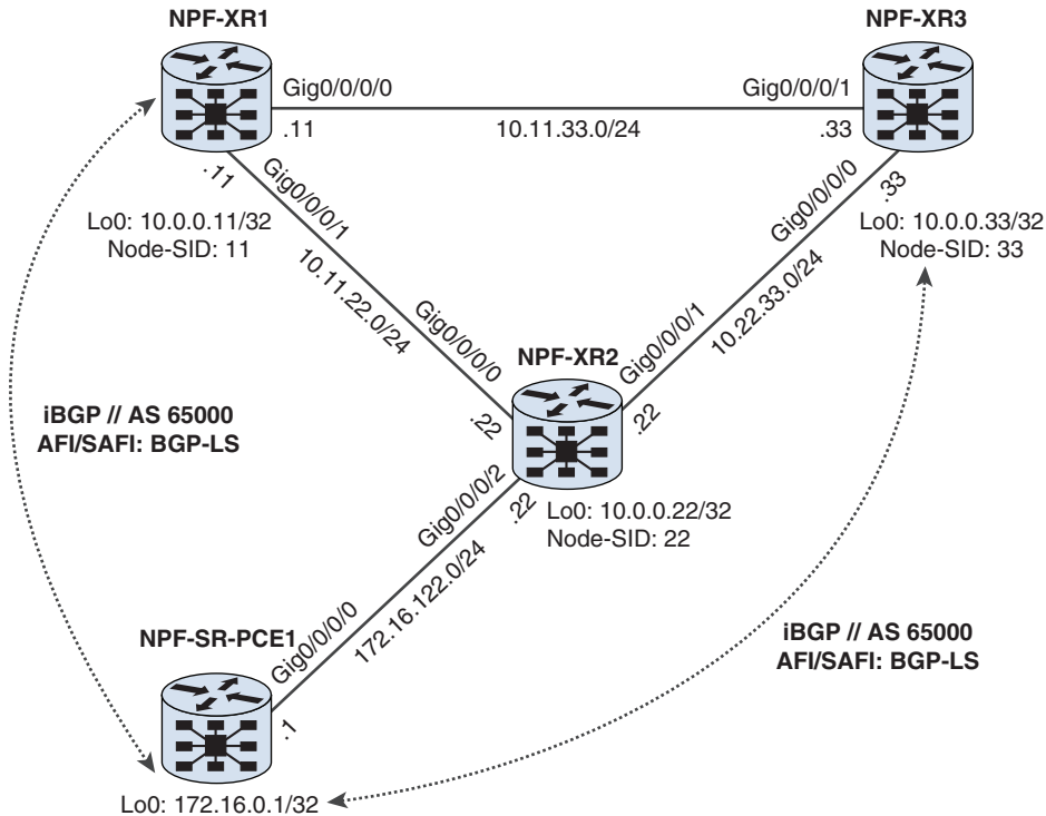
Figure 16-11 Lab Topology for BGP-LS
