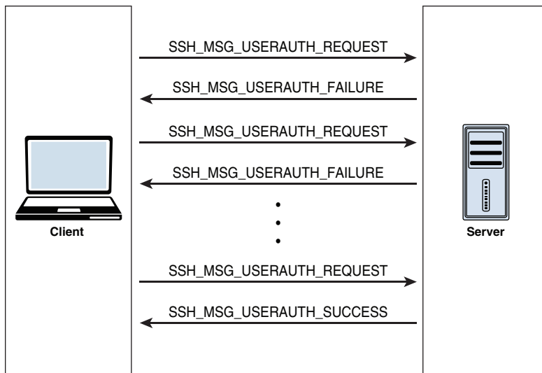
Figure 9-5 SSH-AUTH Message Exchange
