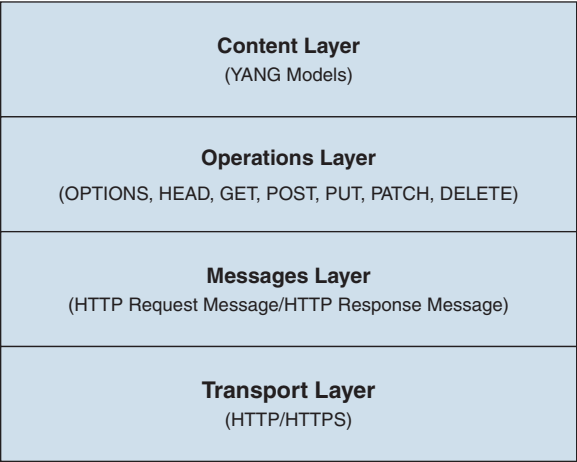
Figure 14-5 The Four-Layer Model Encompassing All RESTCONF Functions
