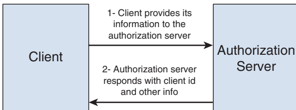
Figure 8-3 Client Registration with the Authorization Server
