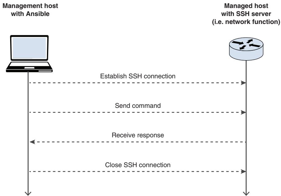
Figure 19-1 Ansible Call Flow for a Single Command
