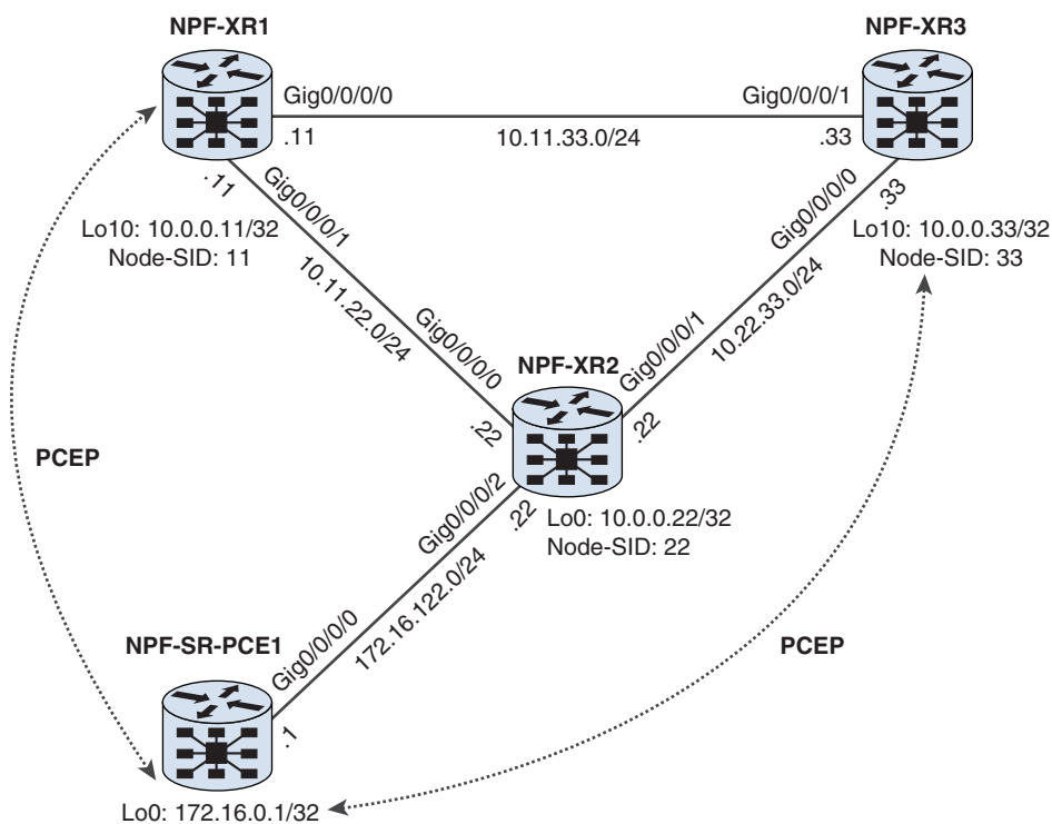
Figure 16-18 The Lab Topology with the PCEP Lab Peering
