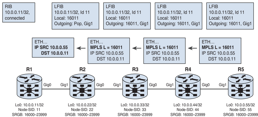
Figure 16-6 Generic Process of Segment Routing Forwarding
