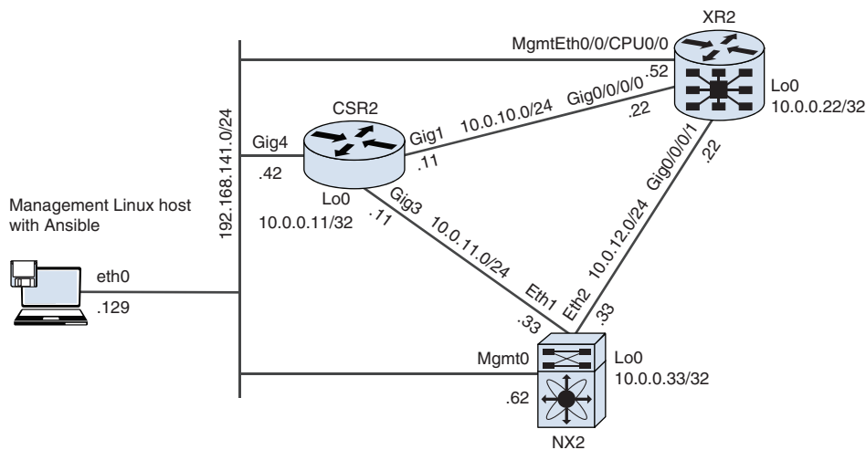
Figure 19-5 Topology Used for Cisco Automation with Ansible
