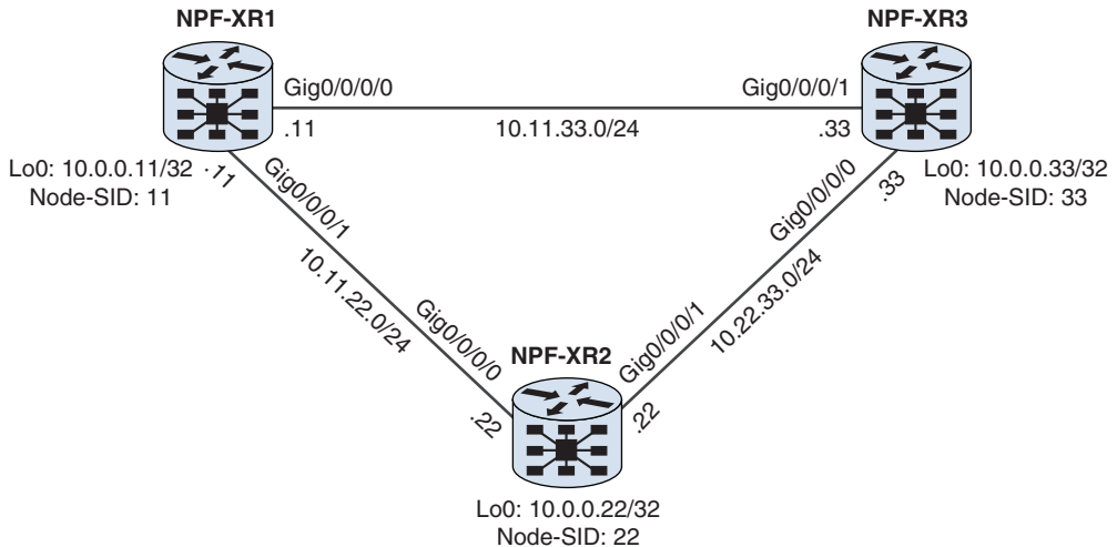
Figure 16-4 Segment Routing Lab Topology
