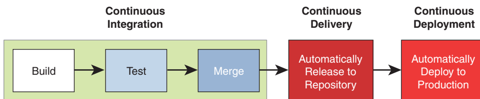
Figure 1-6 CI/CD
