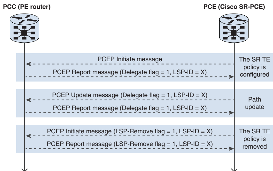
Figure 16-17 PCE-Initiated MPLS LSP
