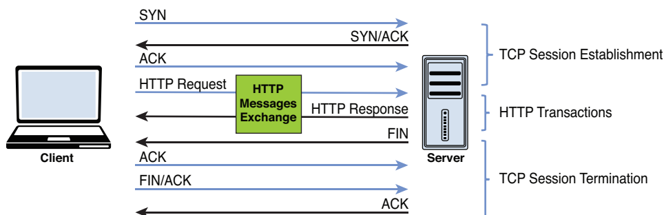
Figure 7-2 TCP Connection Establishment and Termination with HTTP Message Exchange In Between
