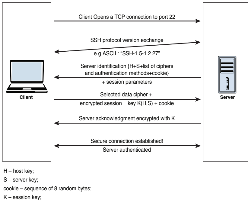
Figure 9-2 SSH1 Protocol Packet Exchange
