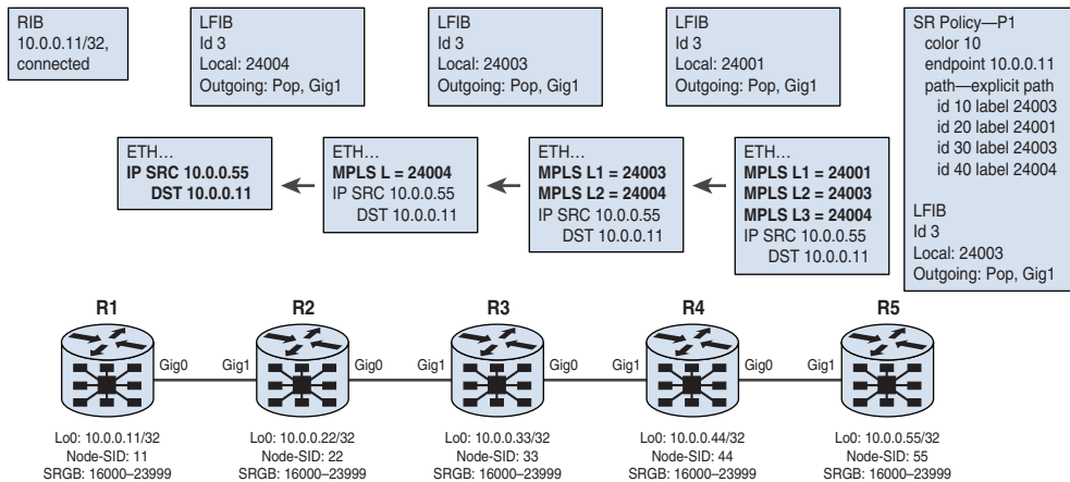
Figure 16-9 Generic SR-TE Process Using Adj-SIDs
