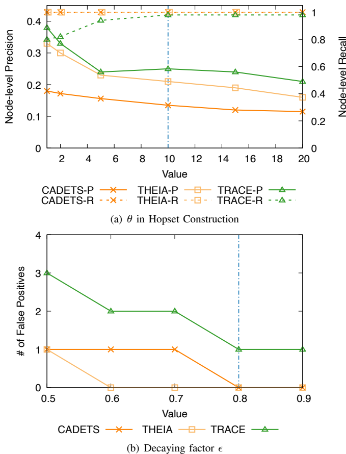
Fig. 10: Performance of NODLINK on different parameters.
