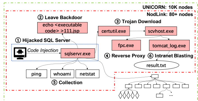
Fig. 6: An attack that first injects a web shell to SQL Server and leaves a backdoor. Then it downloads Trojan for reverse proxy and intranet blasting. During the whole procedure, it collects the system information.
