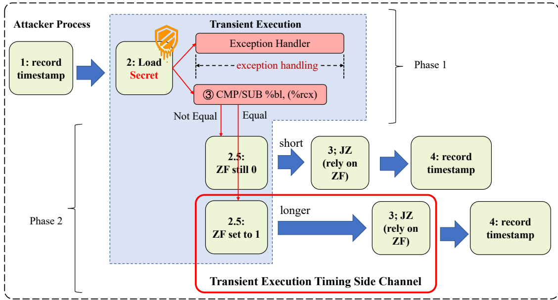
Fig. 1: Overview of Transient Execution Timing Side-Channel.
