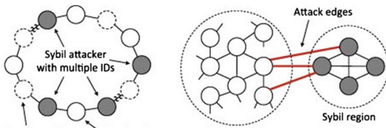
Fig. 8 Sybil attack
