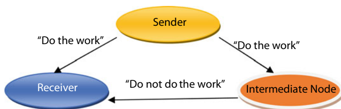
Fig. 11 Byzantine attack
