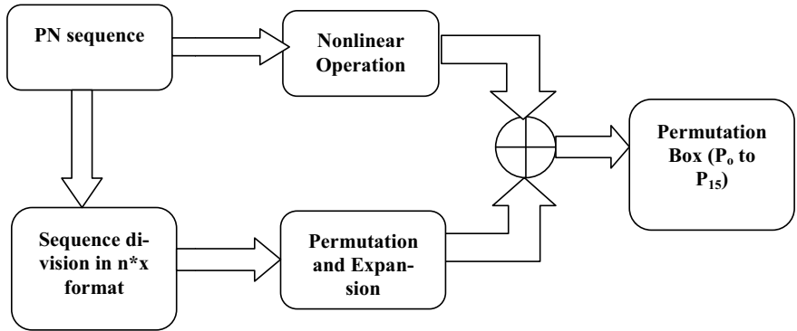
Fig. 12 Functional block diagram of the P-box
