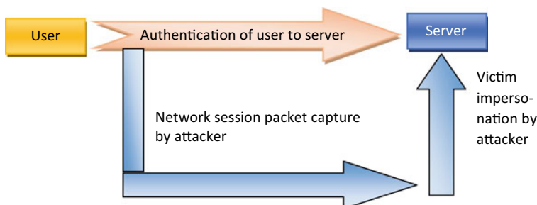
Fig. 10 Replay attack
