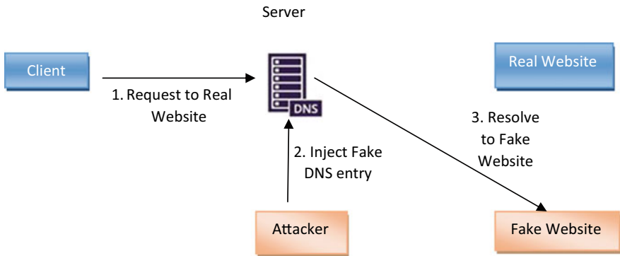
Fig. 5 Spoofing
