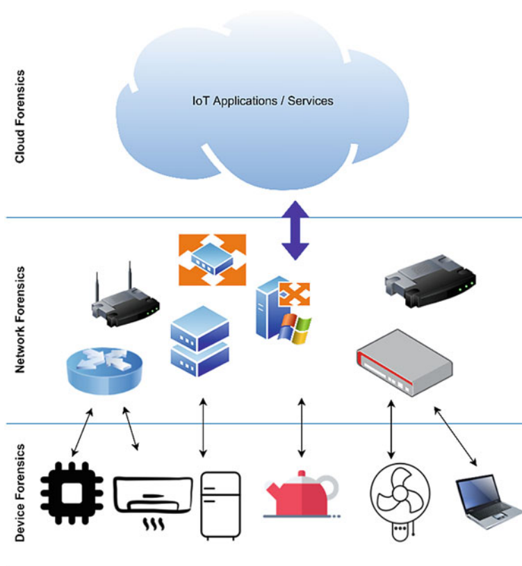
Fig. 7 IoT forensics
