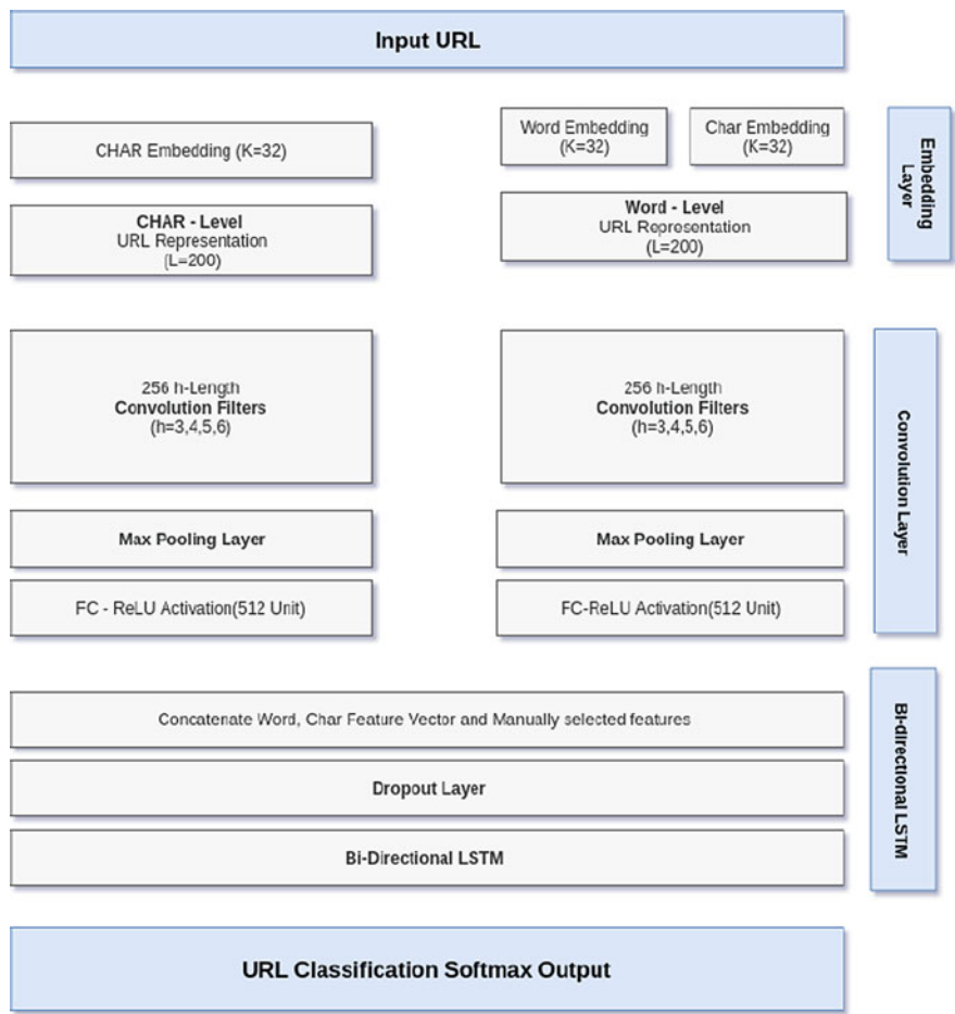
Fig. 9 Model configuration
