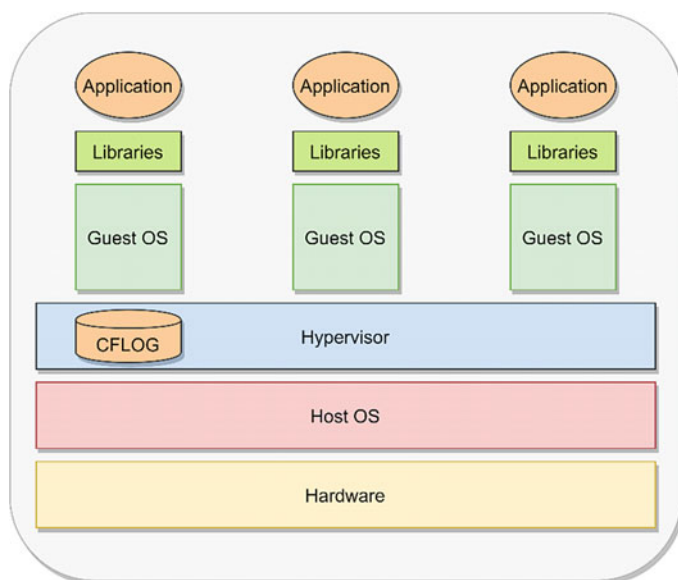
Fig. 5 CFLOG overview
