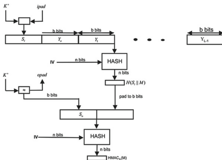
Fig. 10 HMAC algorithm
