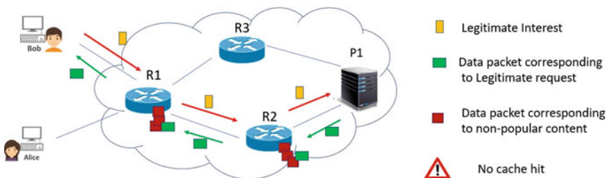
Fig. 5 Cache pollution attack
