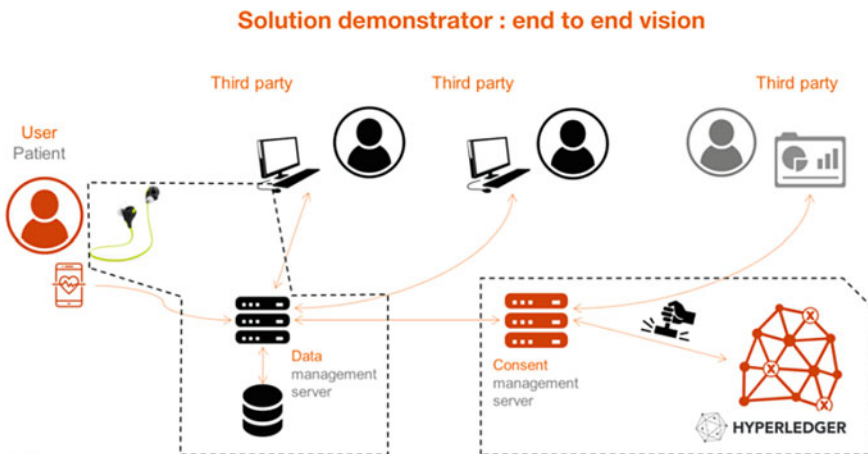
Fig. 9 Solution demonstrator
