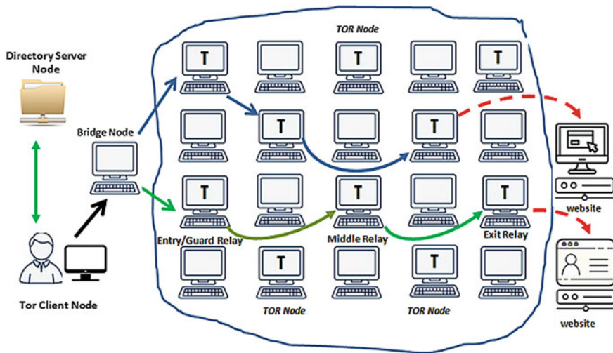
Fig. 9 Bridge node
