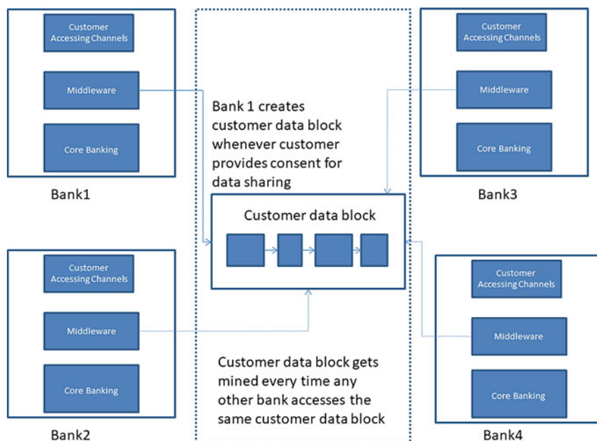
Fig. 6 Solution architecture
