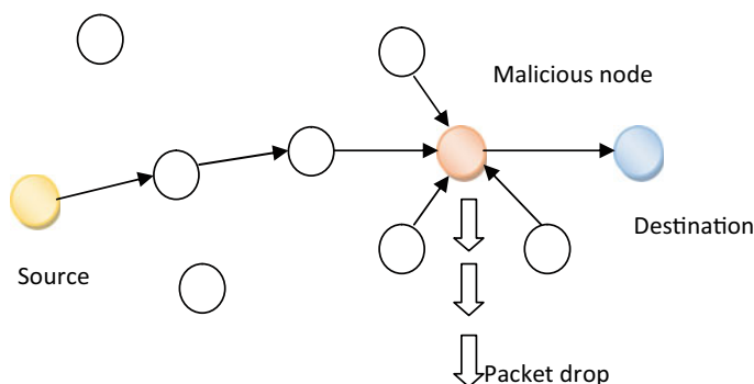
Fig. 7 Sinkhole
