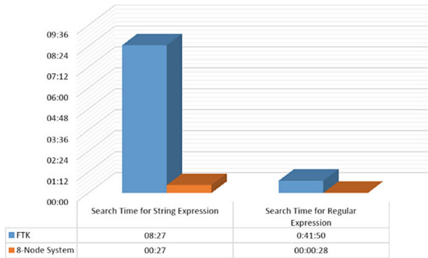
Graph 2 Search times on 8-node system
