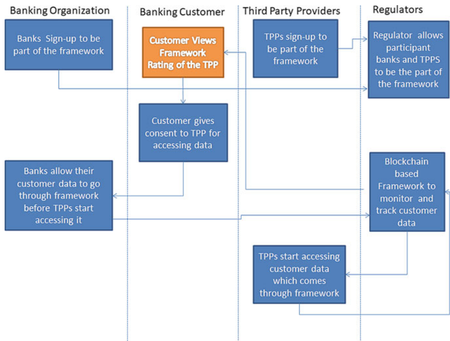
Fig. 5 Flow diagram to show the interactions by involved parties
