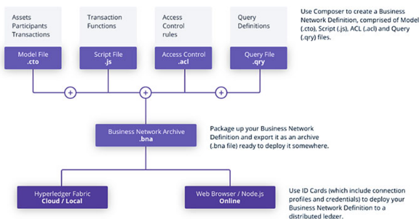
Fig. 7 Component in a typical permissioned blockchain architecture
