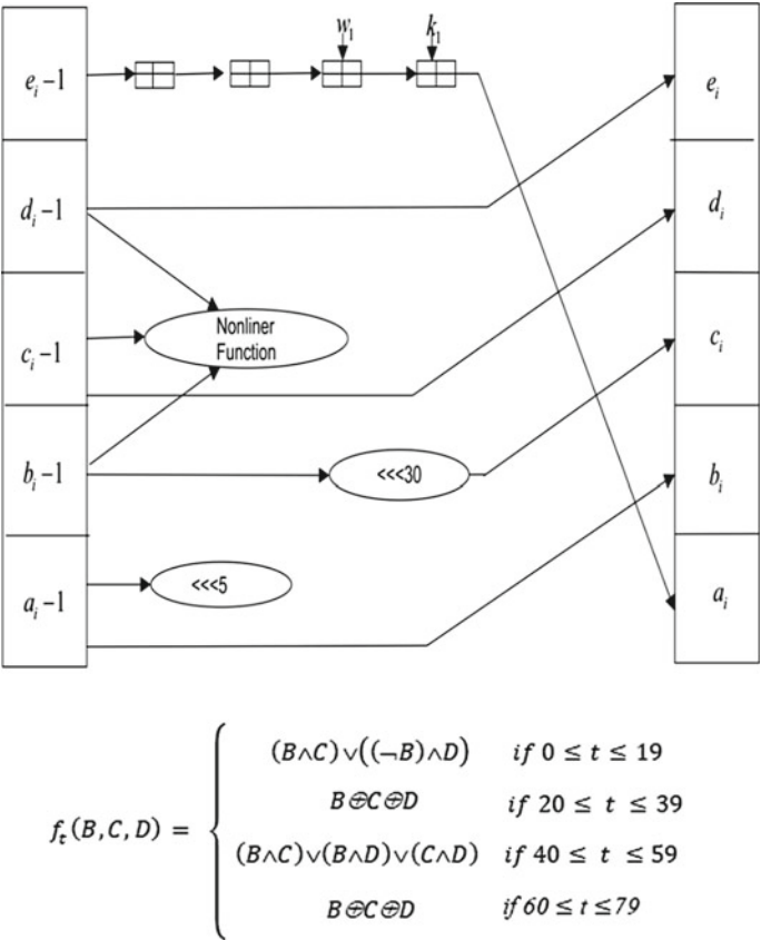
Fig. 9 Each round of SHA-1
