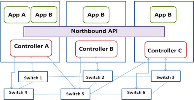
Fig. 5 Secure and dependable SDN
