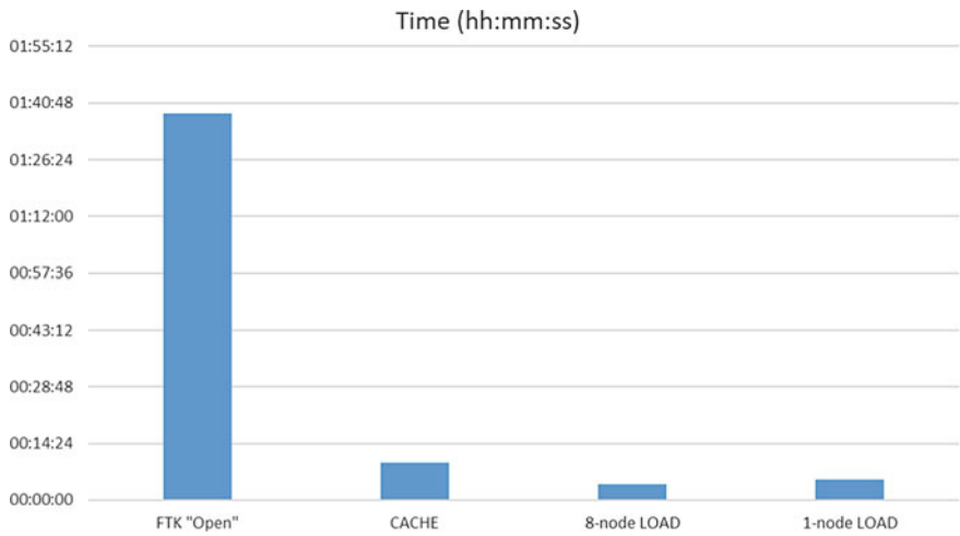
Graph 1 Initialization time by FTK
