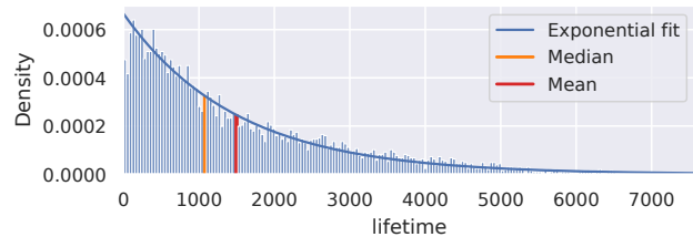
Figure 5: Distribution of vulnerability lifetimes. Equally sized bins.
