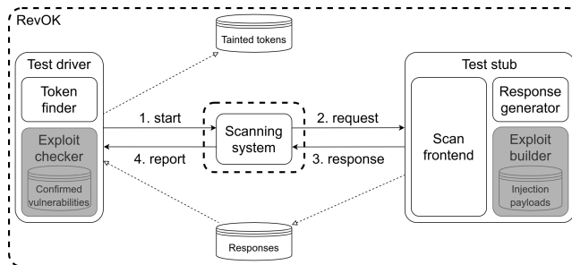
Figure 3: Phase 1 – find tainted flows.
