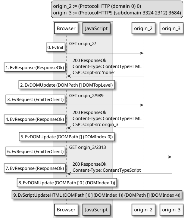
Fig. 7. CSP Inconsistency
