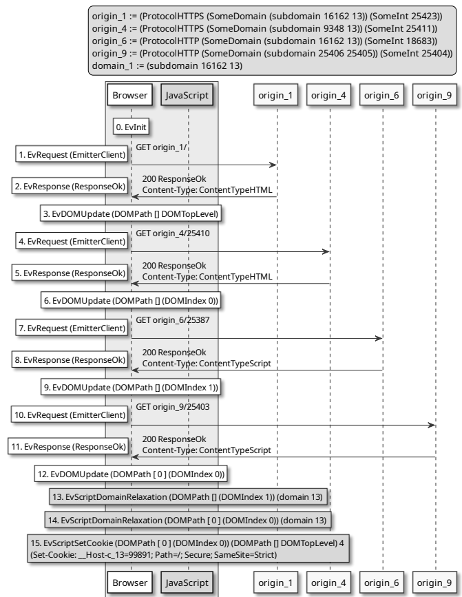
Fig. 4. Host Cookies Inconsistency
