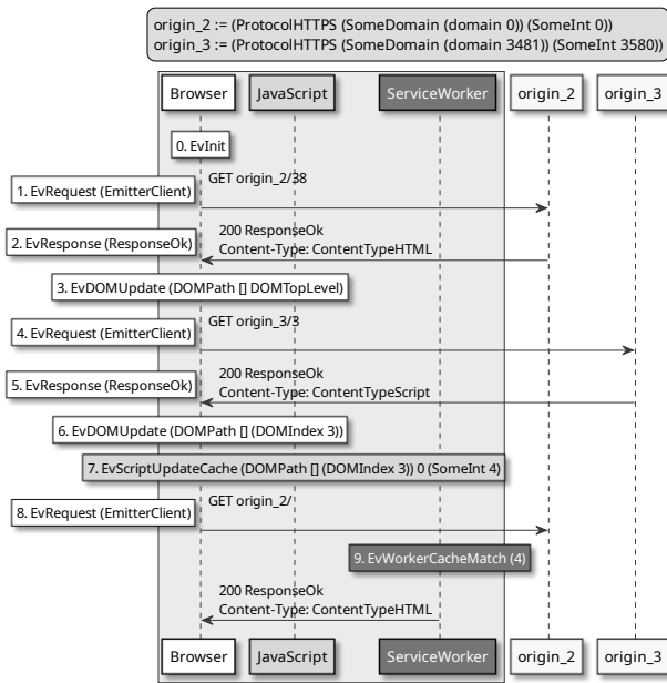
Fig. 8. Service Workers Cache Inconsistency
